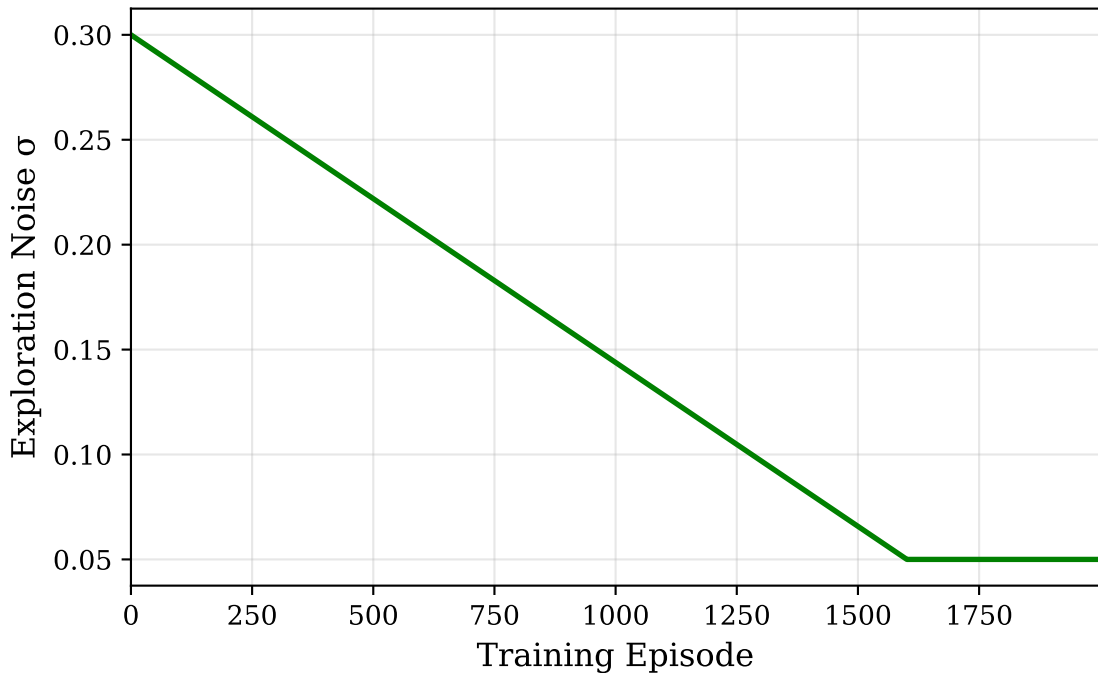
Exploration Noise Annealing
