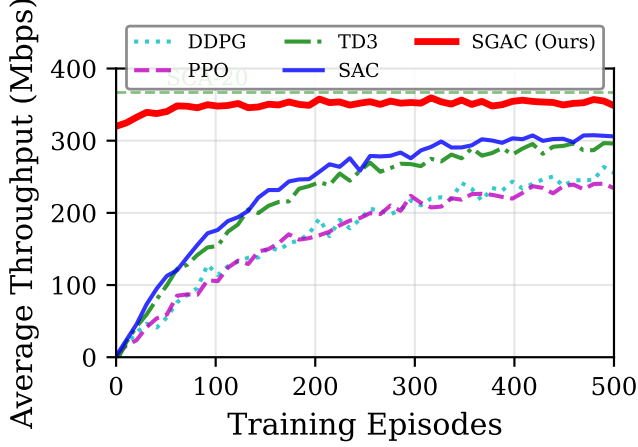
Fig. 2: Training convergence comparison across RL methods. SGAC reaches 95% performance in 50 episodes, 3.6-4.4 \times faster than DDPG, PPO, TD3, and SAC baselines.
