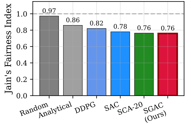
Fig. 4: Jain's fairness index comparison. SGAC balances throughput maximization with fair resource allocation.
