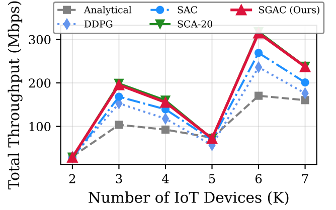
Fig. 3: Scalability with number of IoT devices. SGAC maintains performance parity with SCA across varying network sizes.
