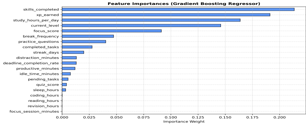
Figure 7: Model 2 Gradient Boosting Feature Importance Ranking
