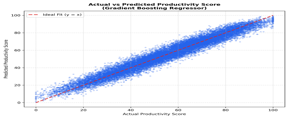
Figure 6: Predicted vs Actual Productivity Scores Scatter Plot
