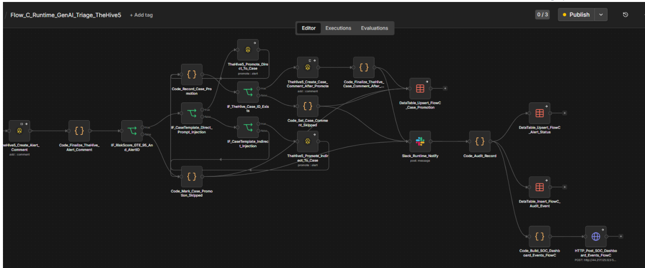
Figure C3 - Flow C right-side zoom: comments, case promotion, Slack, audit tables, and dashboard posting.
