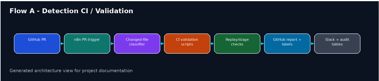
Architecture view - Flow A turns a GitHub PR into validated detection engineering evidence.
