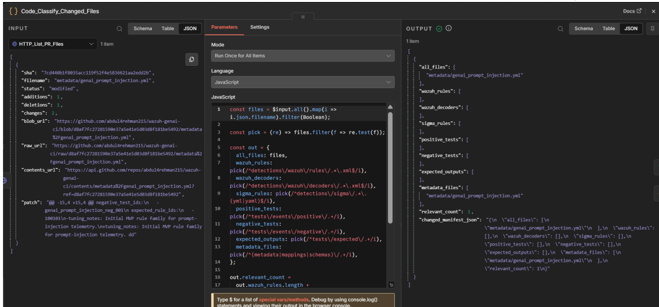
Figure A6 - Code_Classify_Changed_Files output proving metadata-only PR classification for the full CI path.
