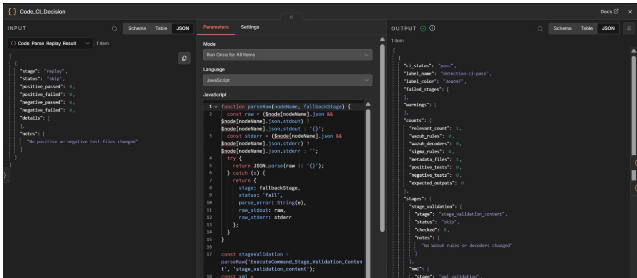
Figure A7 - Code_CI_Decision output showing pass result, no failed stages, and per-stage status details.
