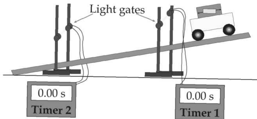
Fig 1.23 Light gates
