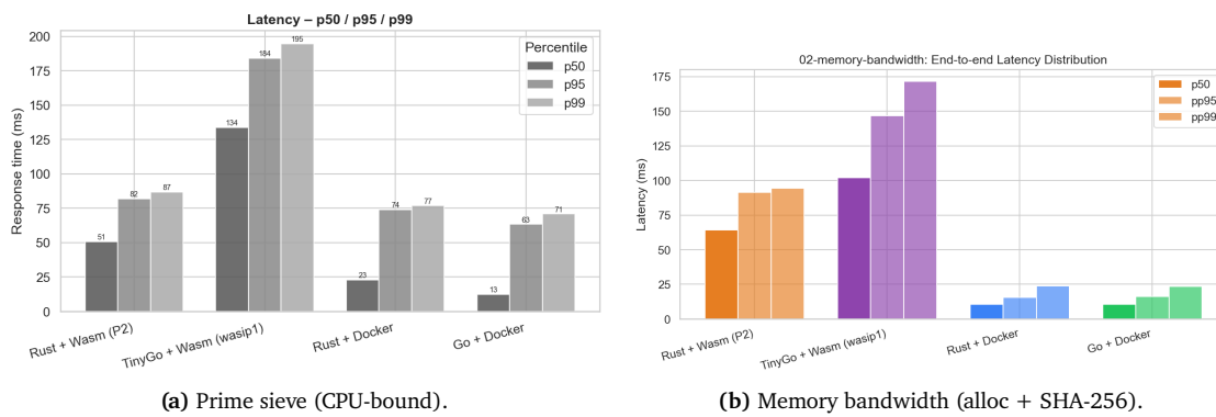
Figure 6.5 – End-to-end request latency (p50/p95/p99) per variant in limited mode.
