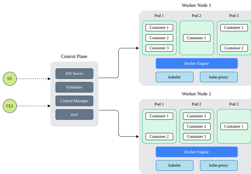
Figure 2.3 – Kubernetes Architecture
