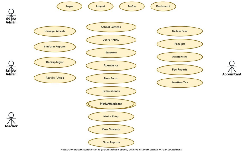
Figure 3.3 — Use Case Diagram School Portal (Four Canonical Roles)
