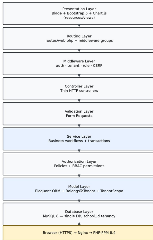
Figure 4.1 — Layered System Architecture School Portal (Laravel 13 Monolith)
