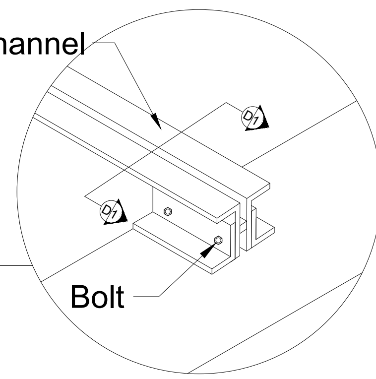
Detail 1 : JOIST CONNECTION TO TOP CHORD
