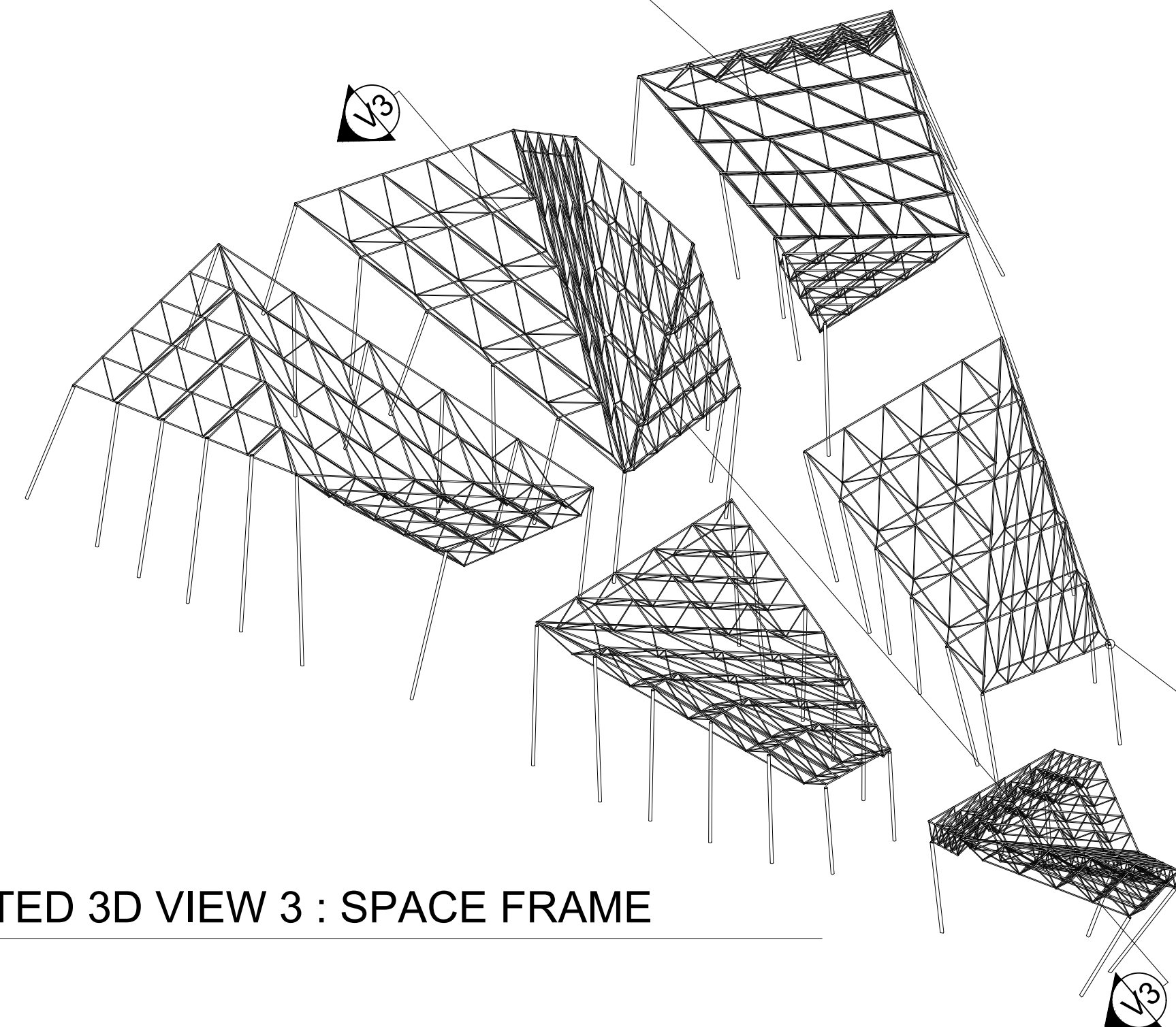
SPACE FRAME 4.8X4.8 GRID 4m DEPTH
