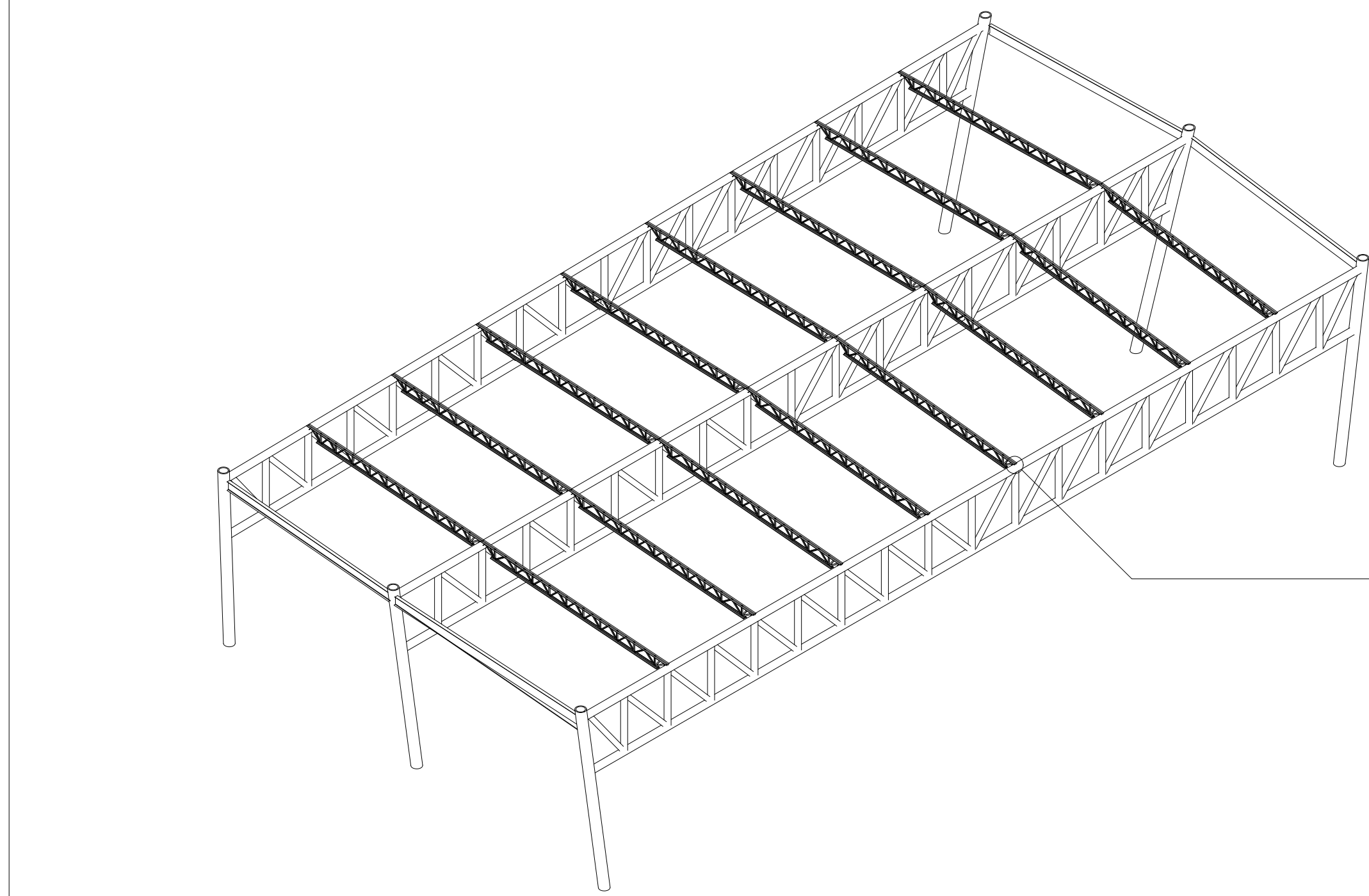
ISOLATED 3D VIEW 1 : TRUSS
