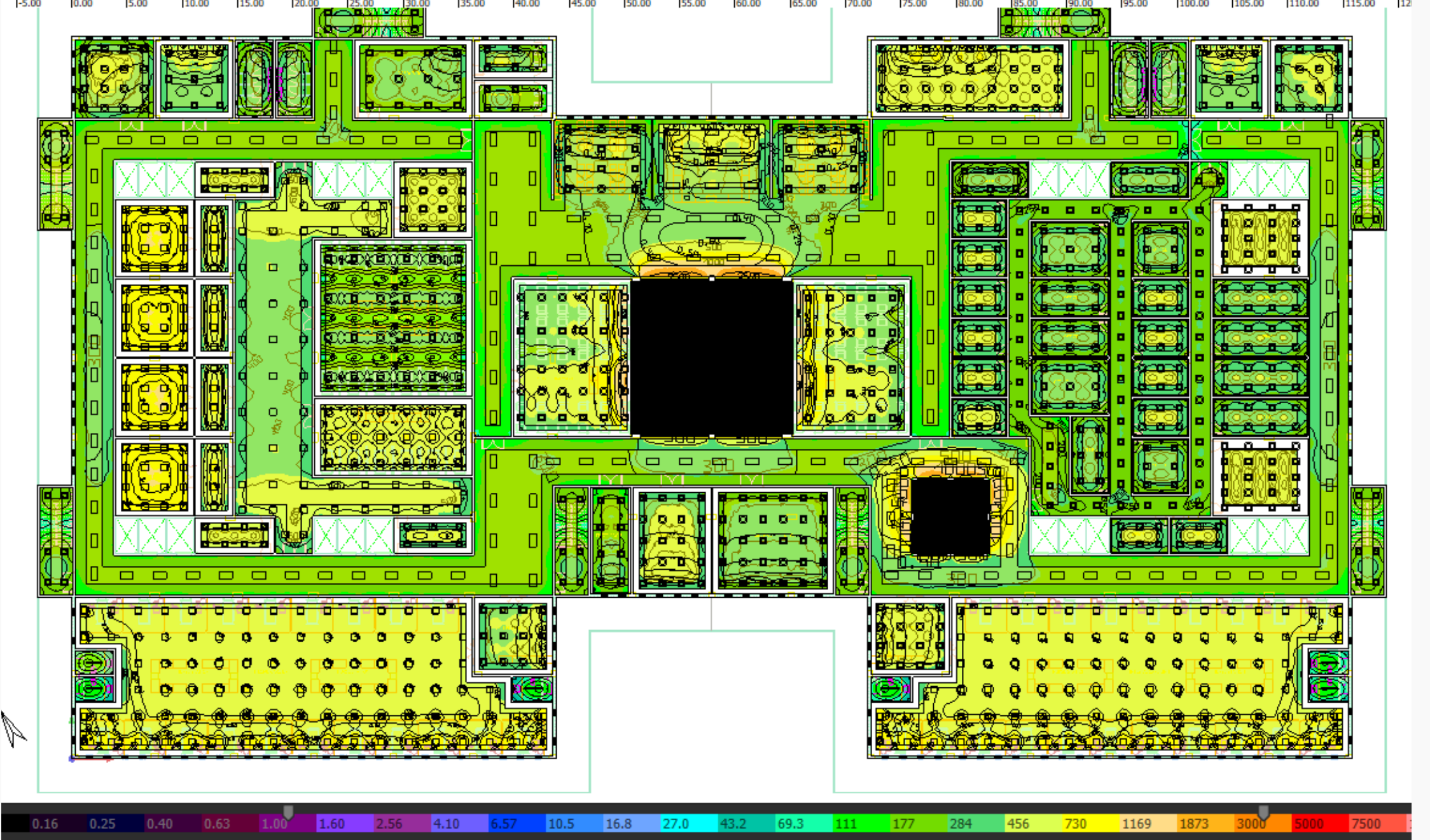
ALL-LIGHT WITH SHADING
