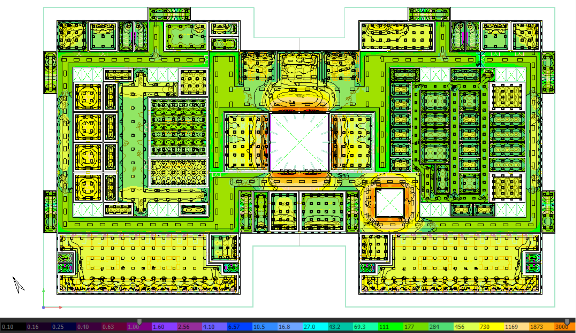
ALL-LIGHT WITHOUT SHADING
