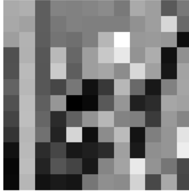
Sampled Image
