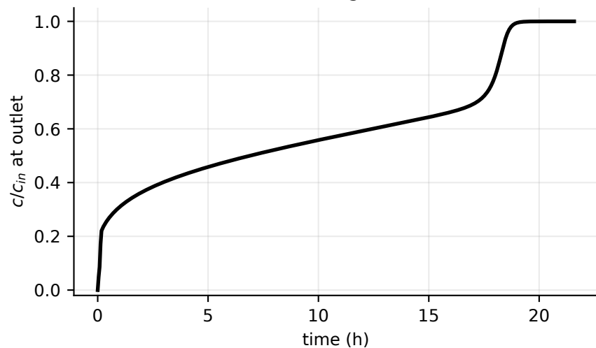
MOF-303-like, Type V breakthrough curve
