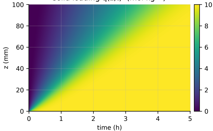
solid loading q(z,t) (mol kg -1 )
