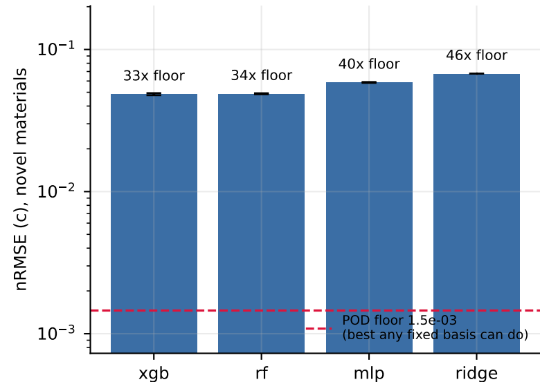
A. L1: data-driven arms vs the representation floor
