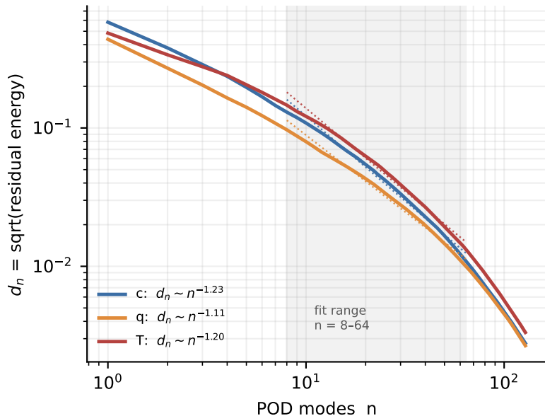
B. n-width: algebraic over the fitted range
