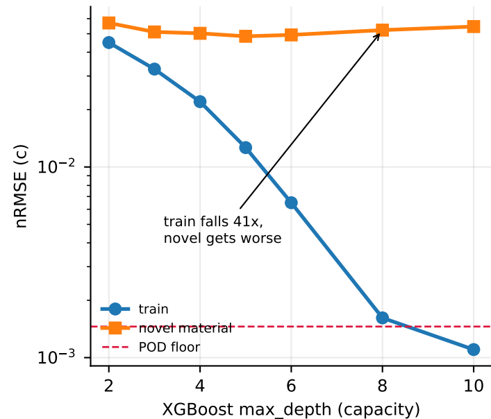
A. L2: capacity buys fit, not generalisation
