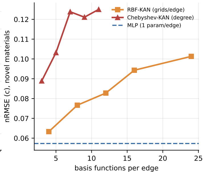
C. More basis per edge -&gt; worse generalisation
