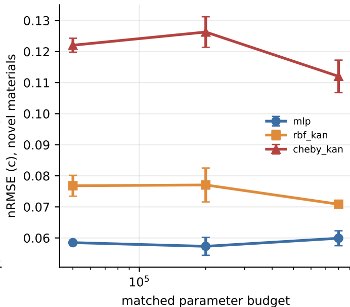
B. L3: ordering identical at every budget
