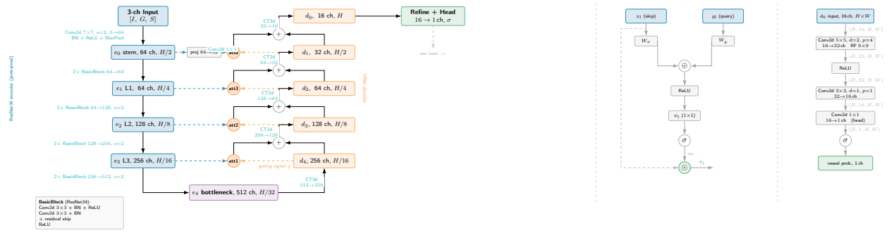
Figure 3: Attention U-Net with attention gate and dilated refine head detail. Left: The ResNet34 encoder (blue) descends from a Conv2d 7 \times 7 stem through four BasicBlock stages to the bottleneck ( e_4 , 512 ch, H/32 ); stage operations are annotated on each encoder arrow. Each decoder upsampling arrow is labelled with its ConvTranspose2d channel mapping (all k=2 , s=2 ). The e_0 skip passes through a 1 \times 1 Conv2d ( 64 \rightarrow 32 ) before the gate. Centre inset: Inside each attention gate, the encoder skip x_l and decoder query g_l are projected by W_x and W_g , summed, passed through ReLU, \psi_l , and sigmoid to give \alpha_l ; the gated skip \tilde{x}_l = \alpha_l \odot x_l is fused with the decoder state. Right inset: The dilated refine head applies Conv2d 5 \times 5 ( d=2 , RF 9 \times 9 , 16 \rightarrow 32 ), ReLU, Conv2d 3 \times 3 ( d=1 , 32 \rightarrow 16 ), a 1 \times 1 head Conv2d ( 16 \rightarrow 1 ), and sigmoid to produce the final vessel-probability map.
