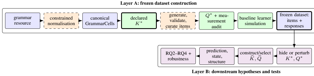
Figure 1: Grammar-KT separates dataset construction from downstream research. Generator truth is fixed before item responses exist. Later discovery and misspecification experiments may hide or perturb it but never redefine the immutable baseline. Model assistance is confined to the dashed linguistic normalisation and item-construction boxes.
