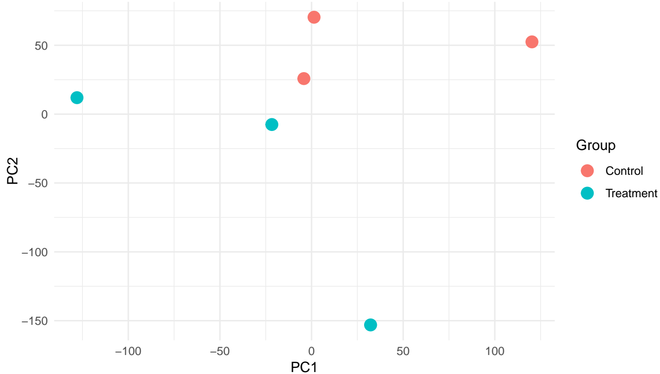
PCA of RNA-seq Samples by Abdullah Alvi
