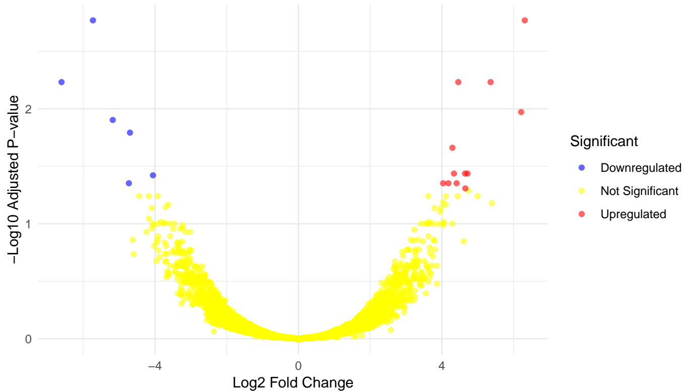
Volcano Plot by Abdullah Alvi
