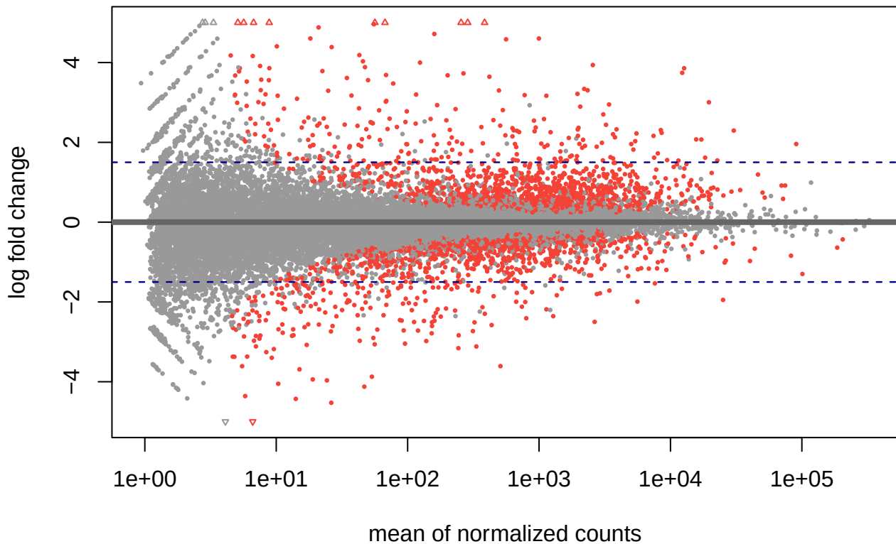
MA Plot — DESeq2 (trt vs untrt)
