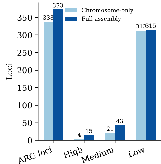
(a) ARG loci by risk tier
