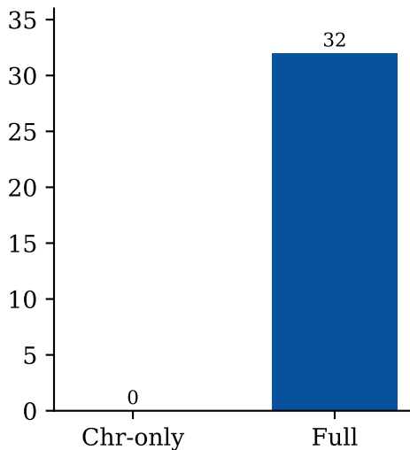
(b) Plasmid replicons
