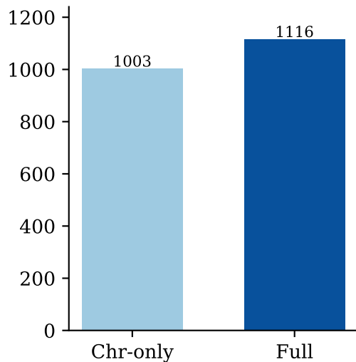
(c) IS features
