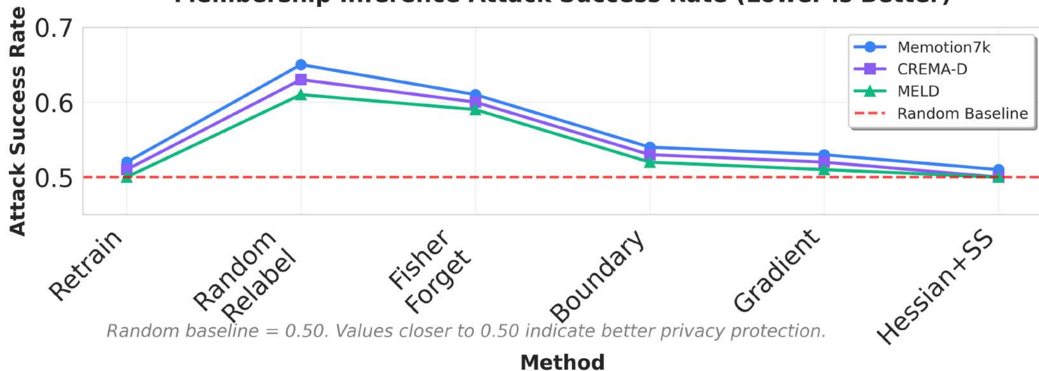
Membership Inference Attack Success Rate (Lower is Better)
