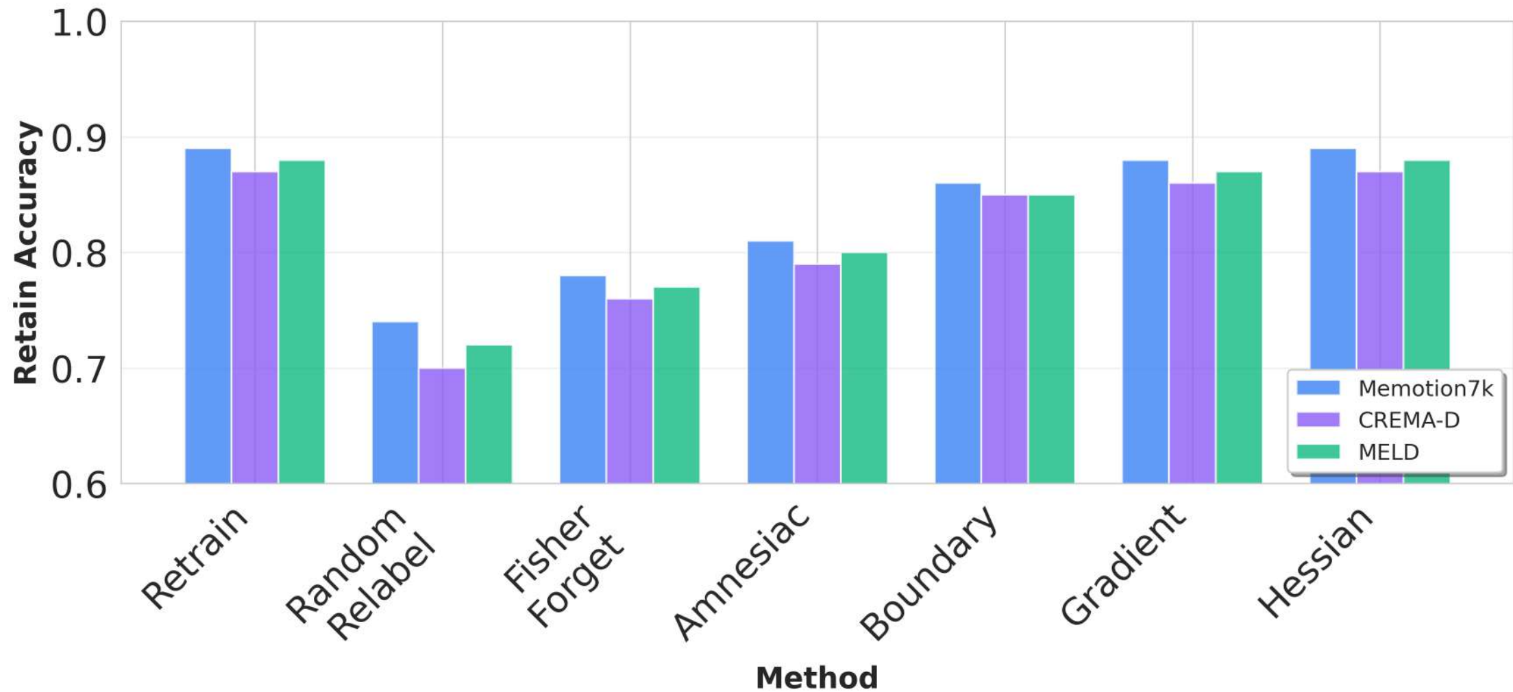
Retain Accuracy Across Methods (Higher is Better)
