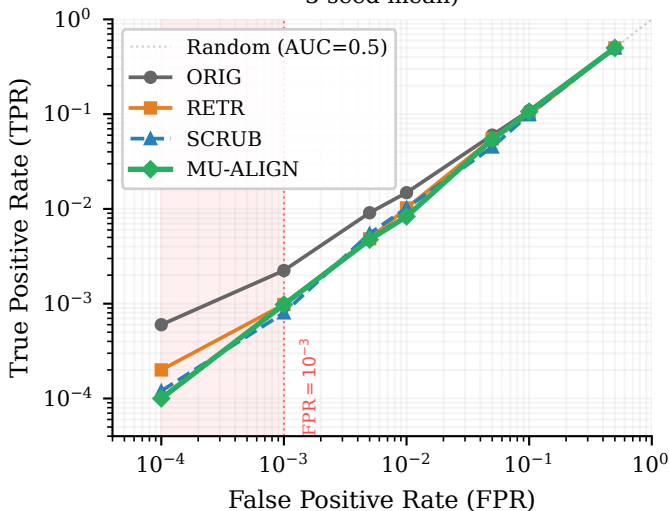
Low-FPR MIA (method-specific calibration, 3-seed mean)
