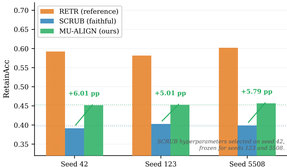
VQA-v2 Answer-Class Deletion: Seed-Level Retained Accuracy
