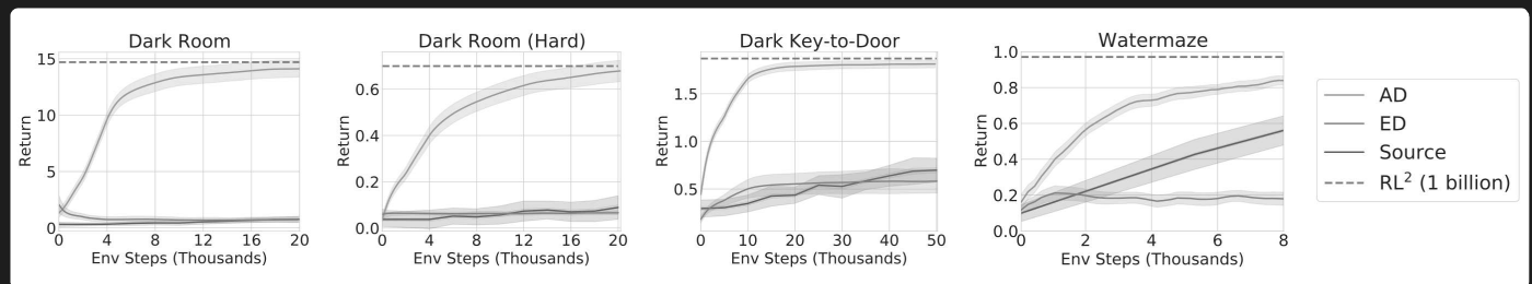
Figure 7: Comparison of AD, ED, source policy and RL^2 on environments that require memory and exploration. Only binary reward is assigned. The source policies are trained with A3C for "dark" environments and DQN for watermaze.
