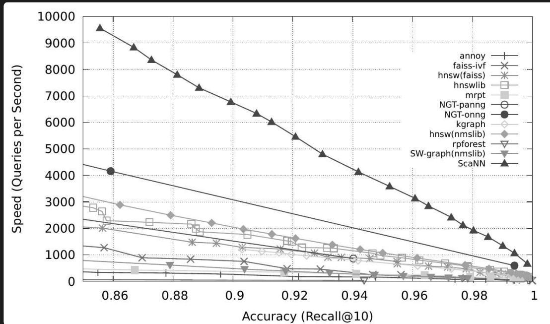
Figure 9: Comparison of MIPS algorithms, measured in recall@10. (Image source: Google Blog, 2020 )
