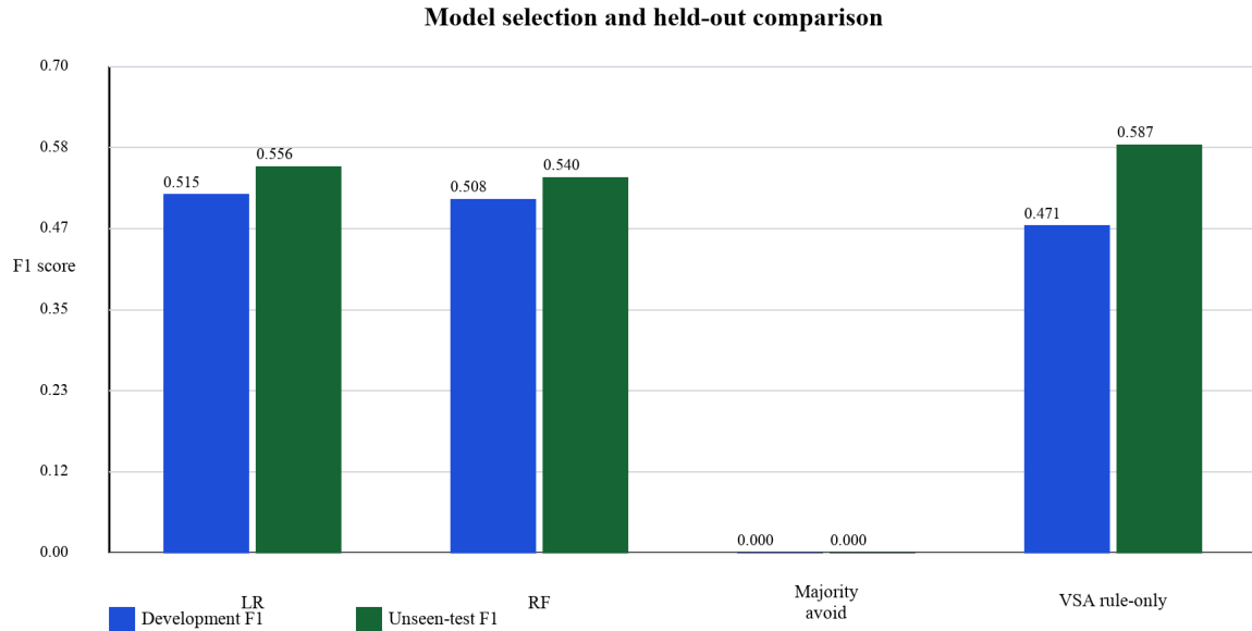
Figure 10. Development and unseen-test F1 for candidate models and baselines. Source: author’s own results.
