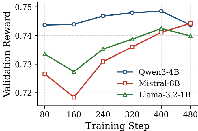
Faith Dataset: Validation Reward vs. Training Step
