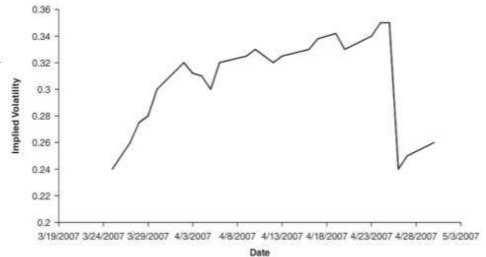
The AAPL Front-Month Volatility around the 2007 Earning Release
