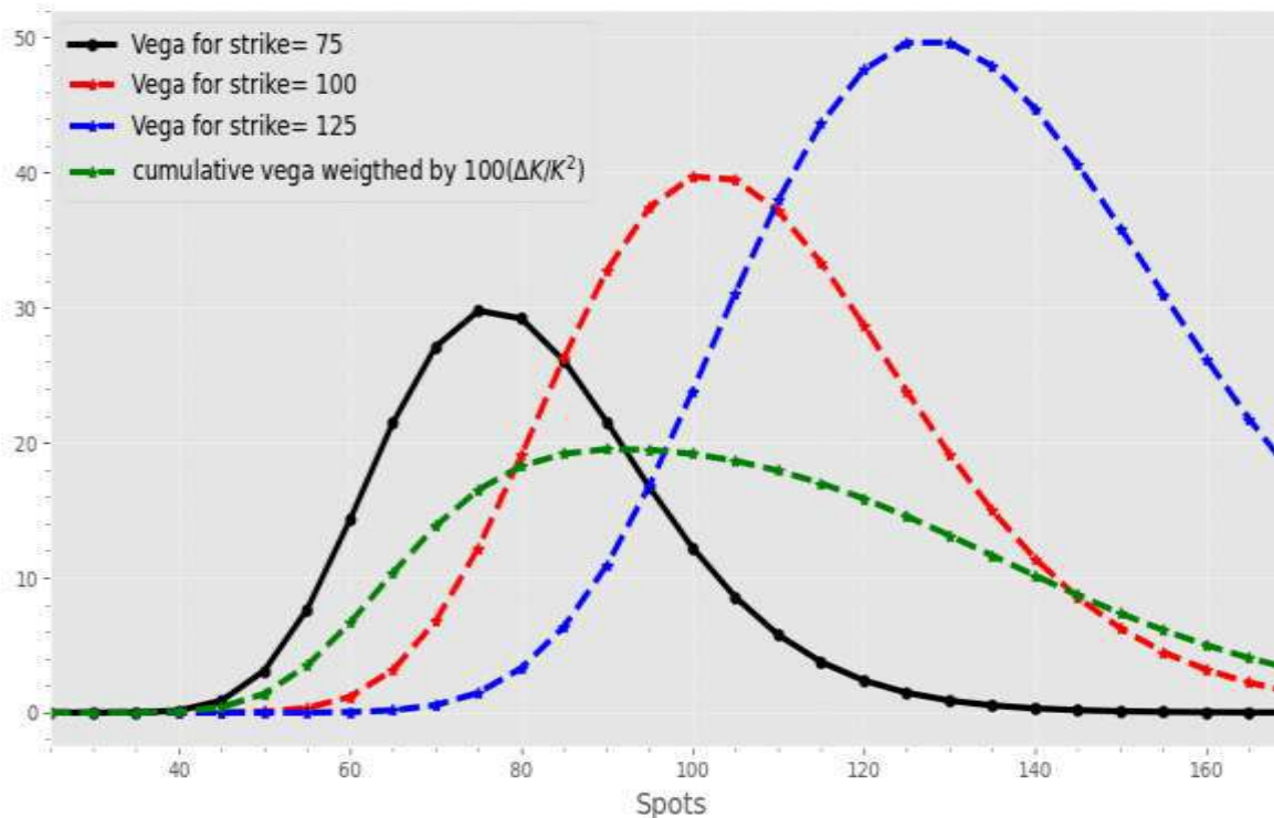
Vega Profile \sigma = 0.2, T = 1
