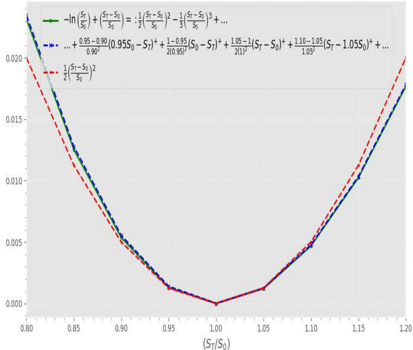
Replicating Higher Order Terms in Log Contract via Options Strip
