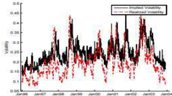
Figure 1A: Implied versus Realized Volatility for Index Options
