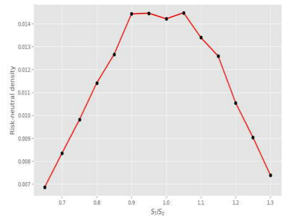
Option pricing via Heston (Vol-of-Vol and skew (dsdv=-0.5))
