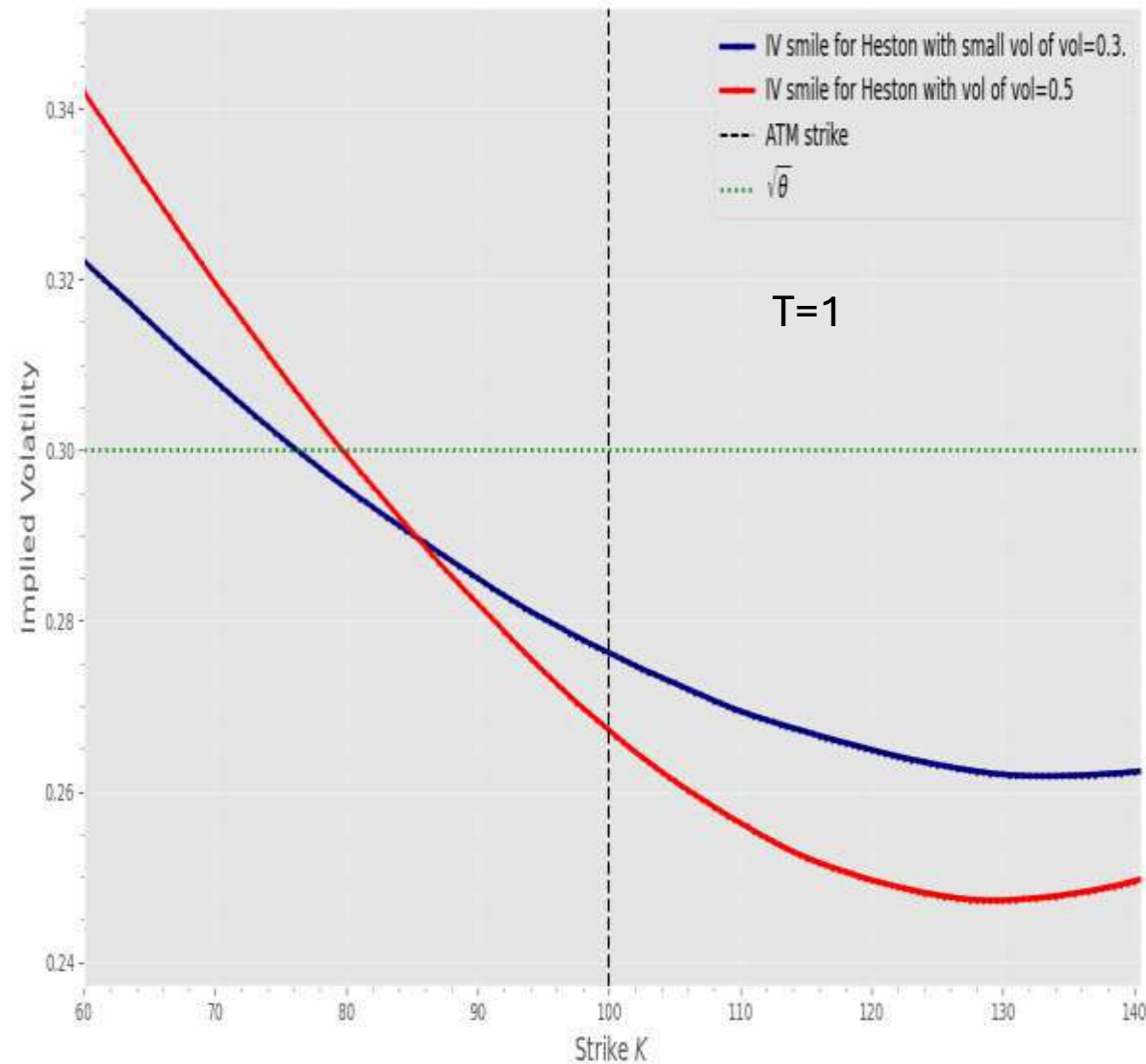
Option pricing via Heston (Vol -of- Vol and skew ( d\sigma dv = -0.5 ))
