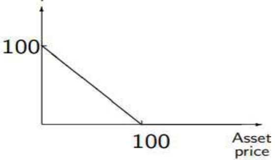
Payoff of buying a put
