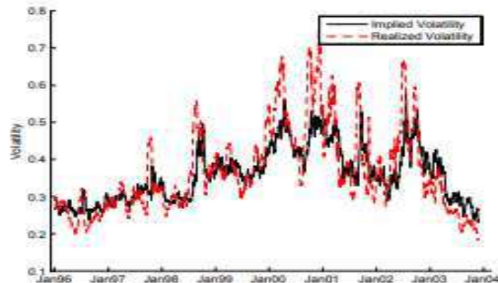
Figure 1B: Implied versus Realized Volatility for Individual Options
