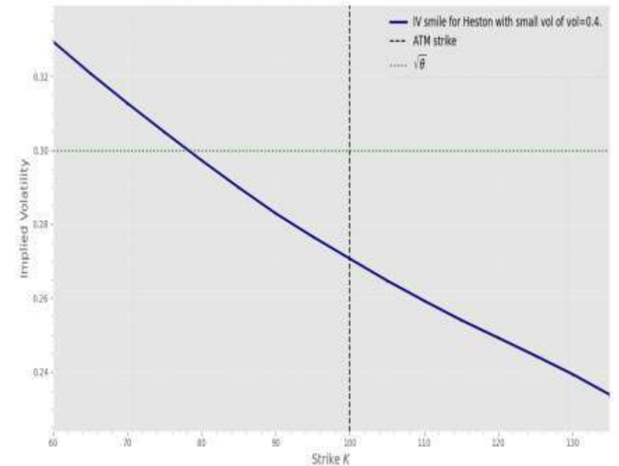
Option pricing via Heston (Vol-of-Vol and skew (dsdv=-0.5))
