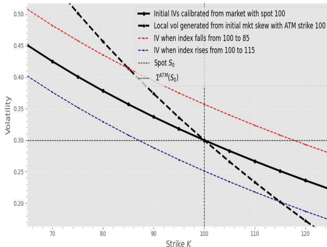
Index Implied Vol Skew and Dynamics
