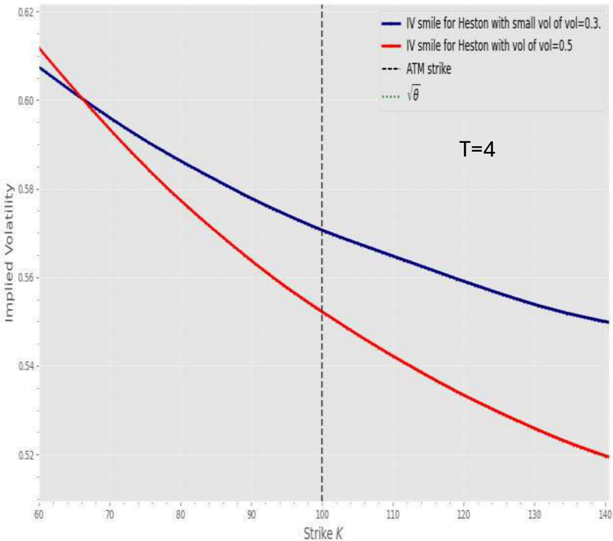
Option pricing via Heston (Vol -of- Vol and skew ( d\sigma dv = -0.5 ))
