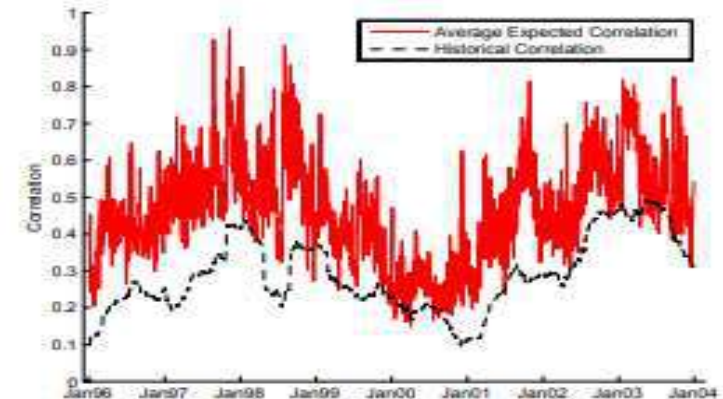
Figure 2A: Risk-Neutral Expected Average Correlation and Historical Correlation
