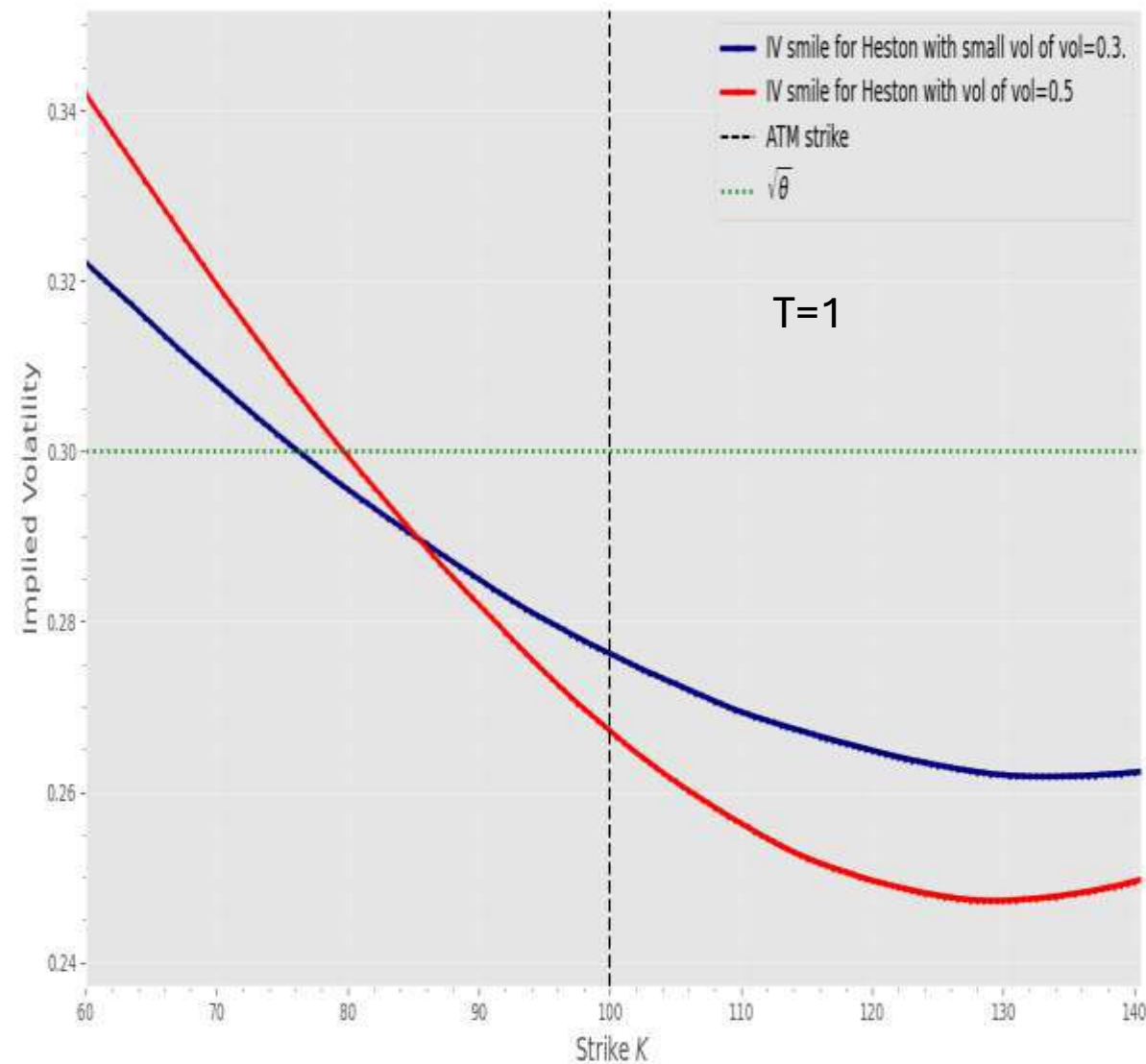
Option pricing via Heston (Vol -of- Vol and skew ( dsdv=-0.5 ))
