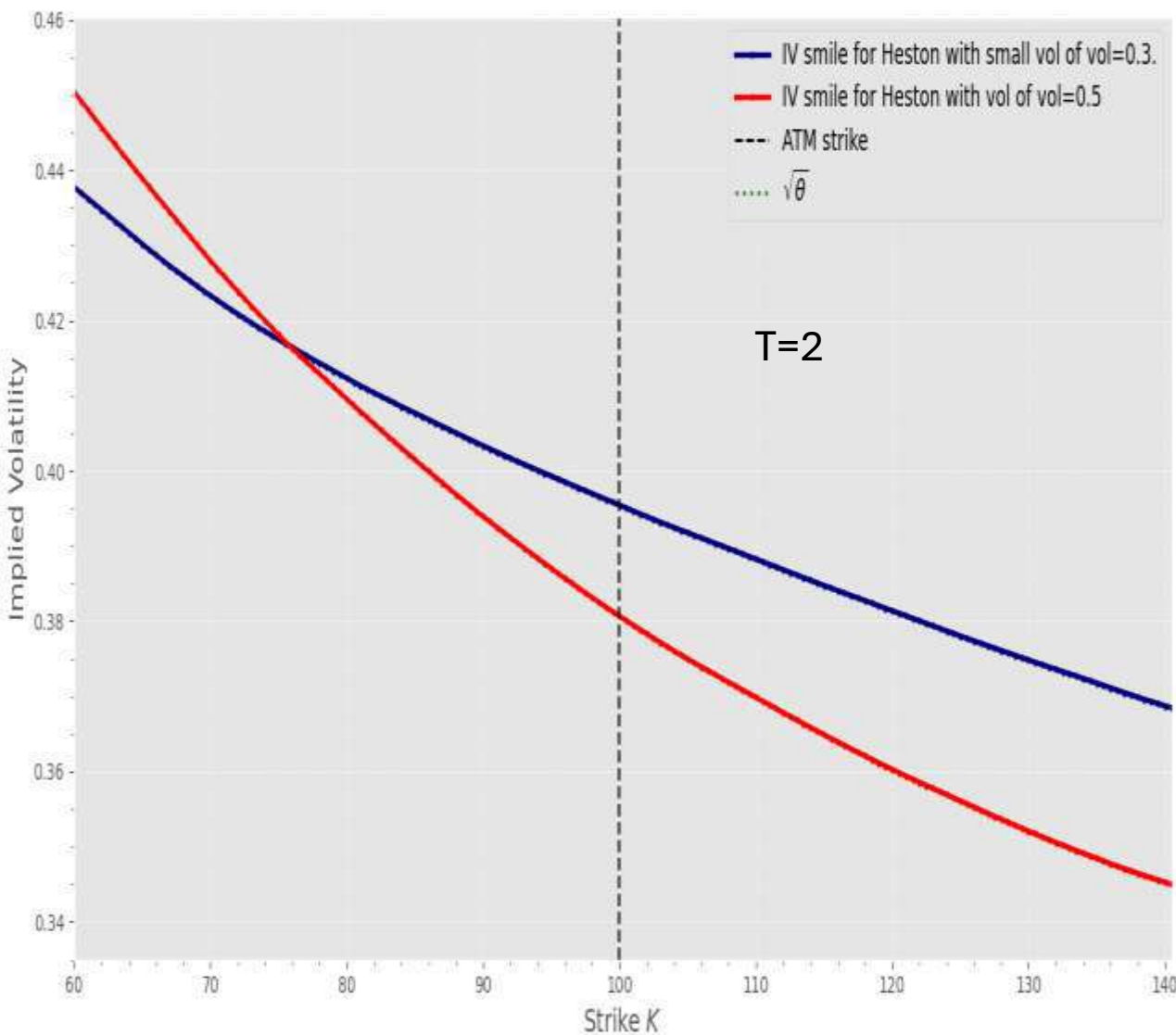
Option pricing via Heston (Vol -of- Vol and skew ( dsdv=-0.5 ))
