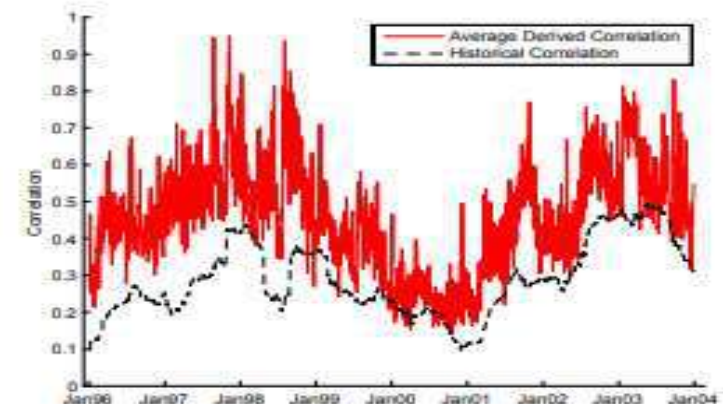
Figure 2B: Average Derived Correlation based on \bar{C}(t) and Historical Correlation
