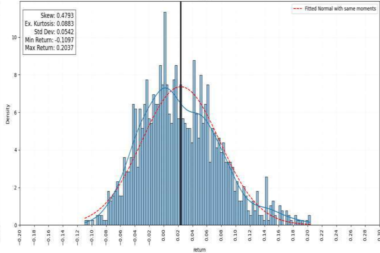
KSE-100 actual return distribution (21 business days) from 2021-01-01 to before crash 2026-02-01
