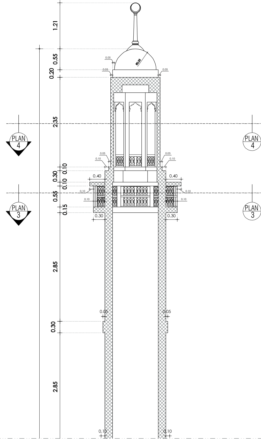
SECTION Y-Y ( SCALE = 1 : 50 )
