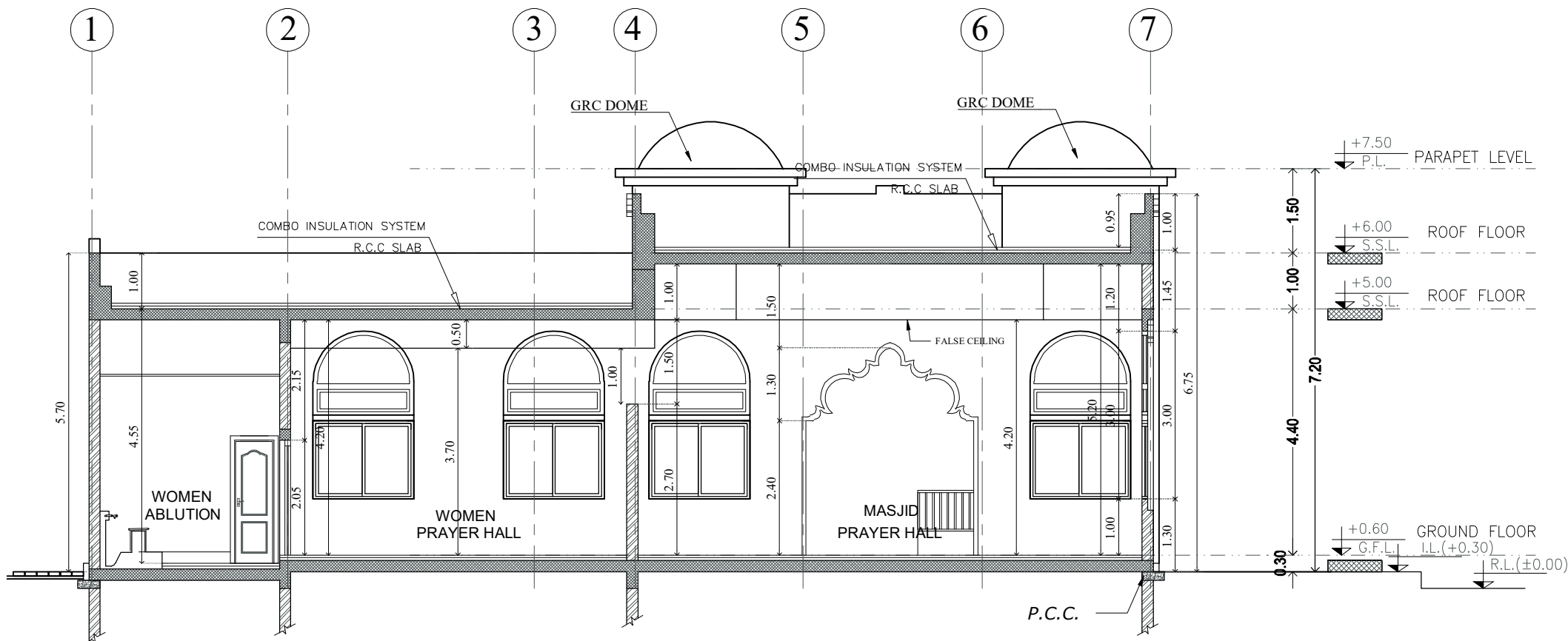
SECTION X - X
