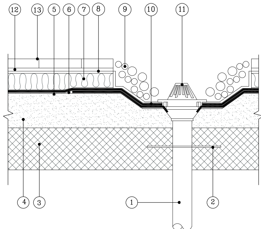
TYPICAL RAIN WATER OUTLET DRESSING DETAILS
