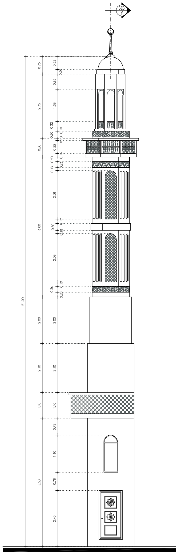
MANAR ELEVATION ( SCALE = 1 : 100 )
