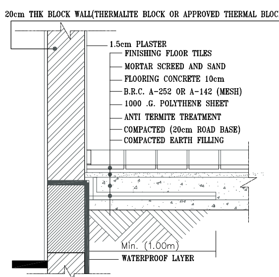
GROUND FLOOR DETAILS
