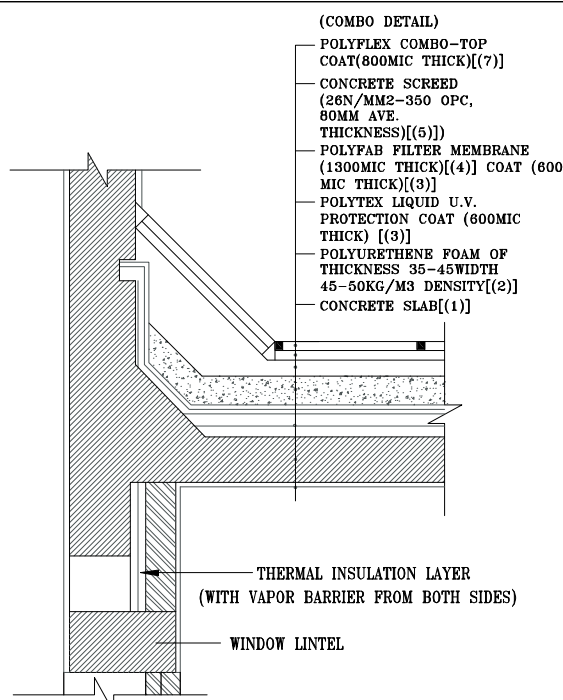
PARAPET & ROOF FINISHING DETAILS
