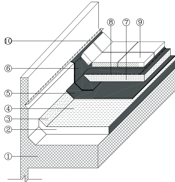
TYPICAL ROOF WATERPROOFING &amp; INSULATION DETAIL WITH GROOVE SYSTEM
