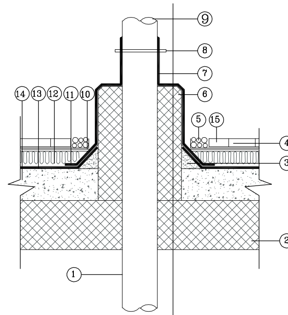
TYPICAL WATER PROOFING DETAILS FOR PIPE PENETRATION
