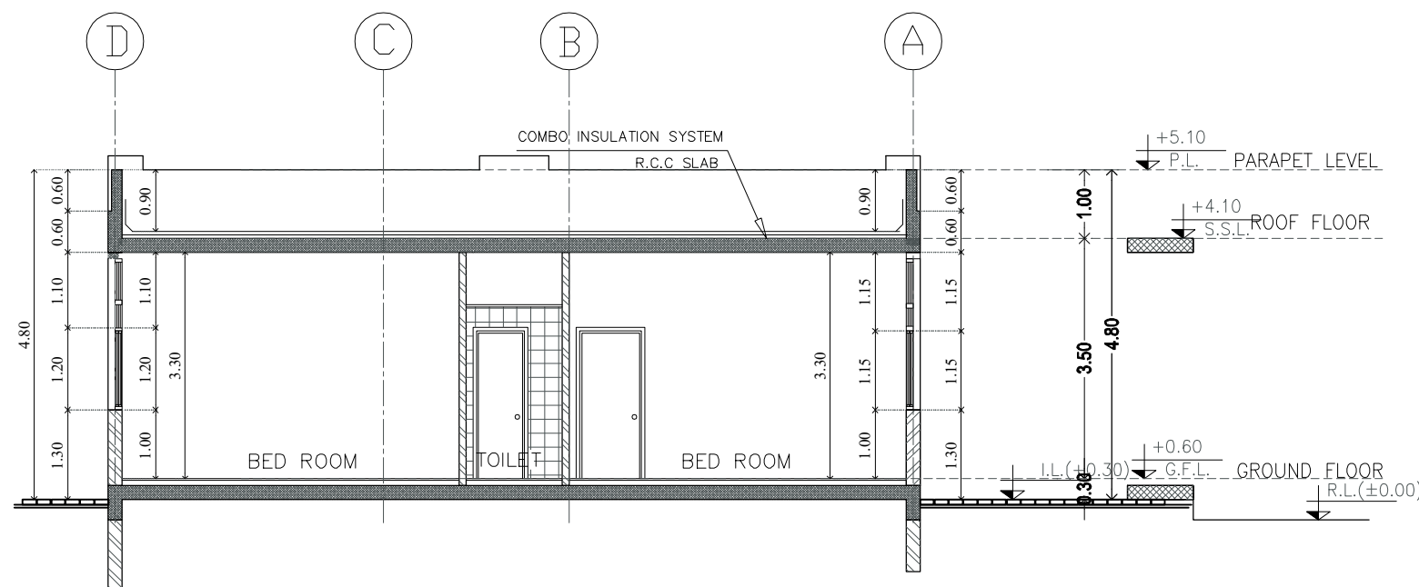
SECTION Y-Y SCALE 1:100
