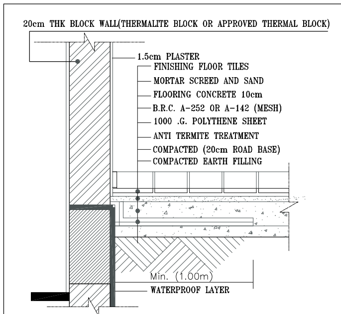
GROUND FLOOR DETAILS
