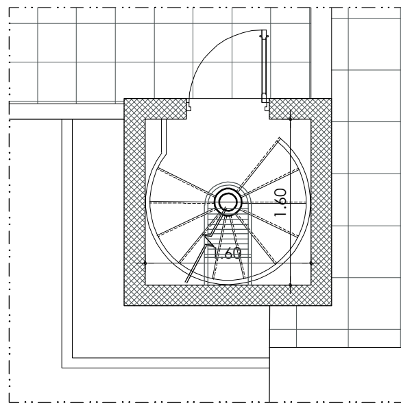
PLAN -2 ( SCALE = 1 : 50 )
