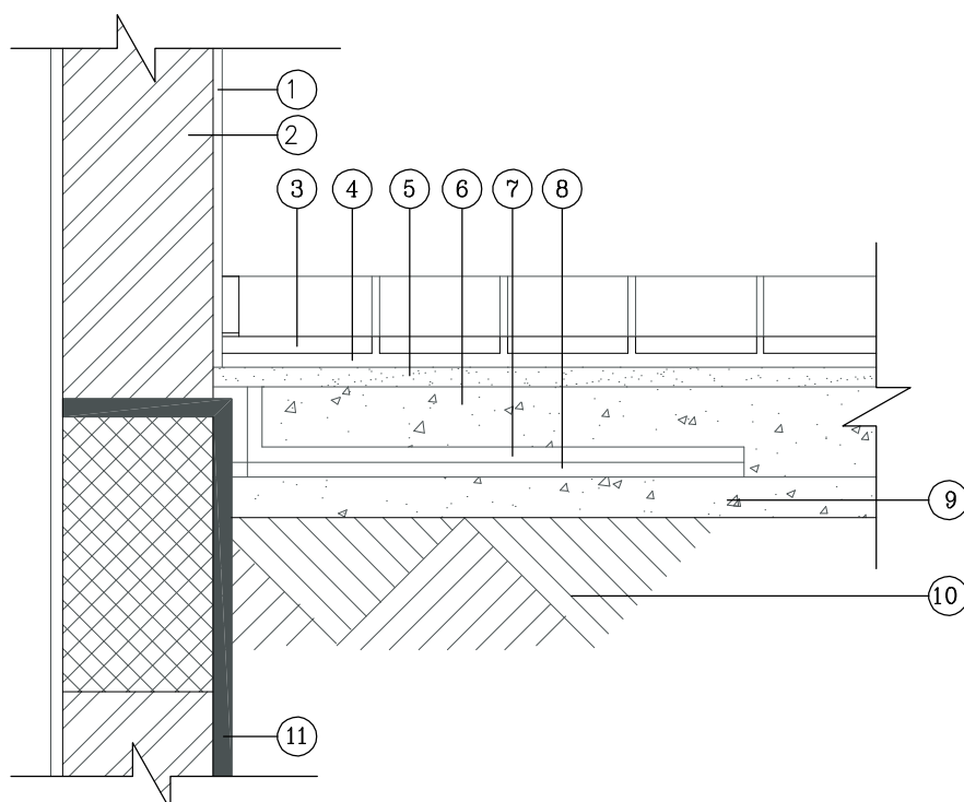
GROUND FLOOR DETIALS
