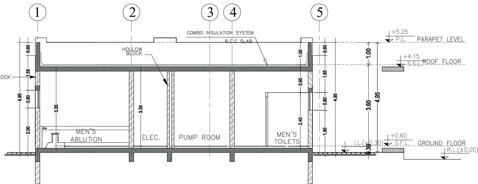
SECTION Z-Z
