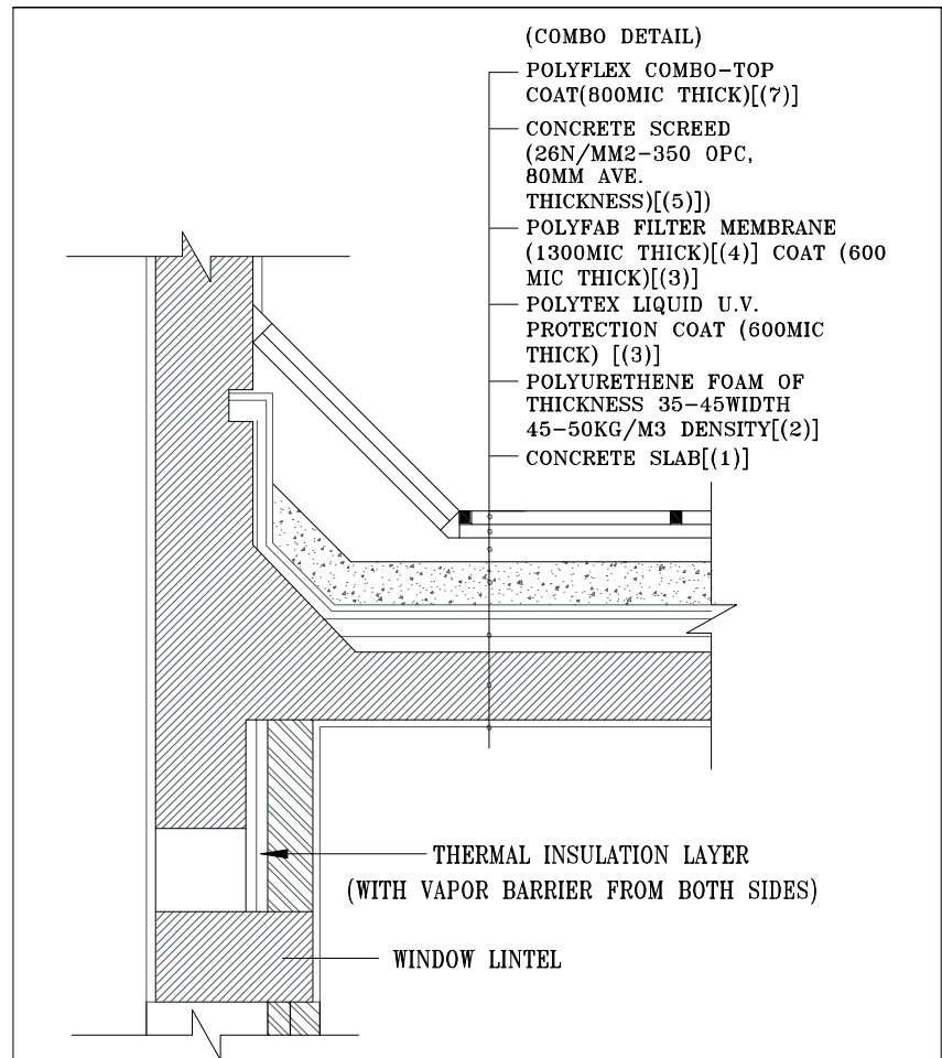
PARAPET & ROOF FINISHING DETAILS
