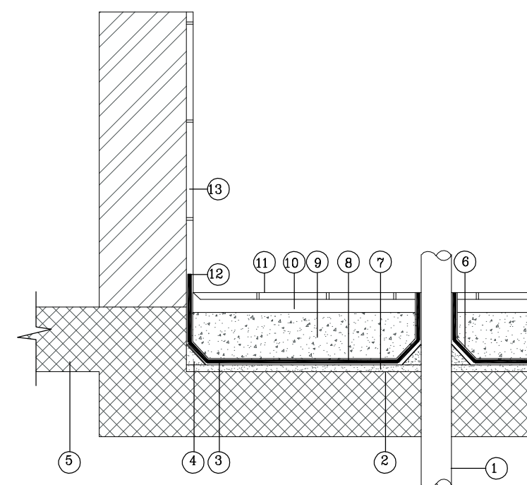
TYPICAL WATERPROOFING DETAILS TO TOILETS, UTILITIES AND OTHER INTERNAL WET AREAS
