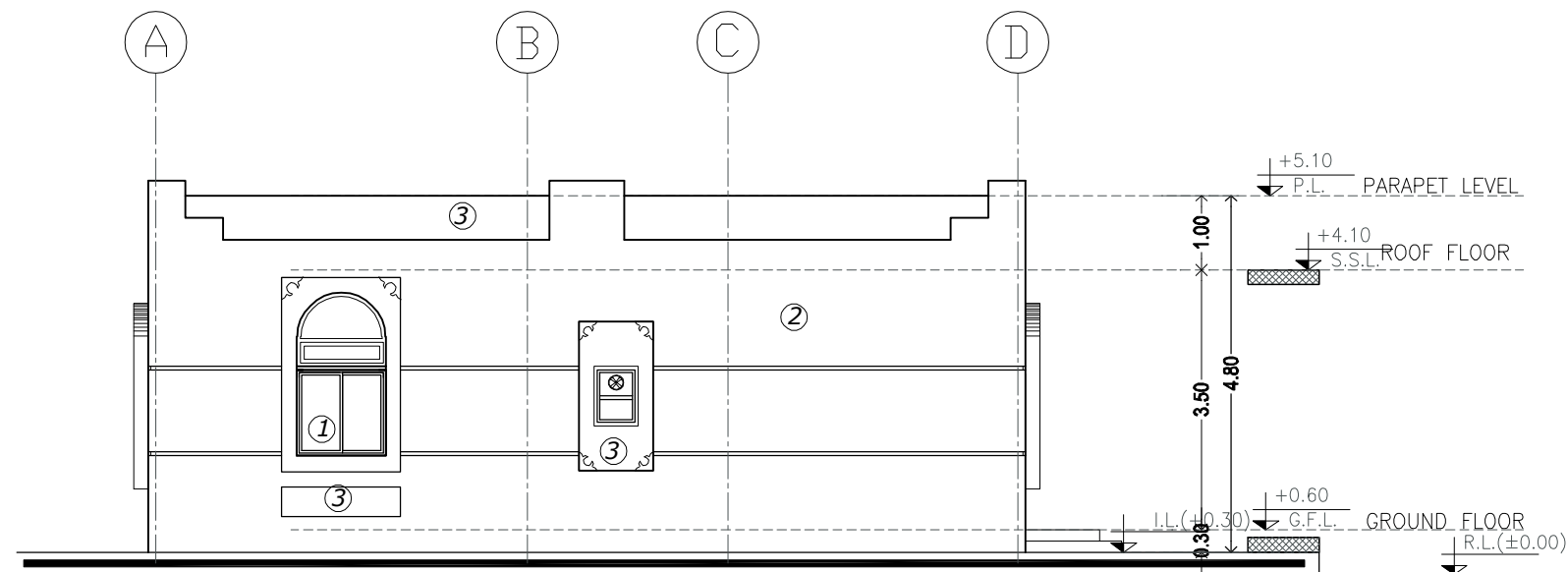
ELEVATION - B SCALE 1:100
