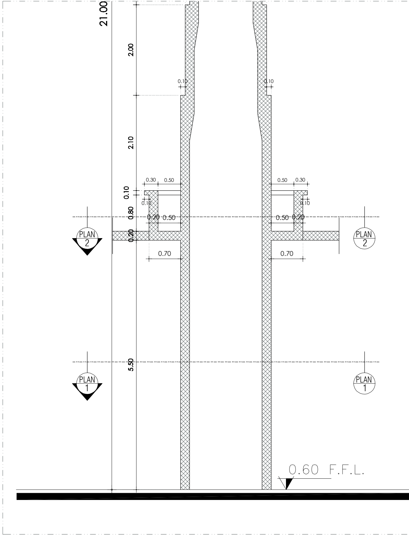
SECTION Y-Y ( SCALE = 1 : 50 )
