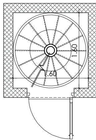
PLAN -1 ( SCALE = 1 : 50 )
