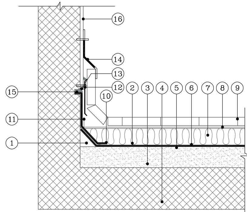
TYPICAL WATERPROOFING DETAILS AT SOUTH PARAPET
