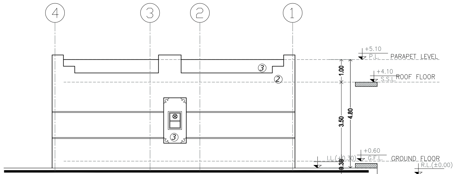
ELEVATION - A SCALE 1:100
