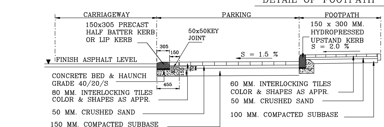
DETAIL OF FOOTPATH & PARKING
