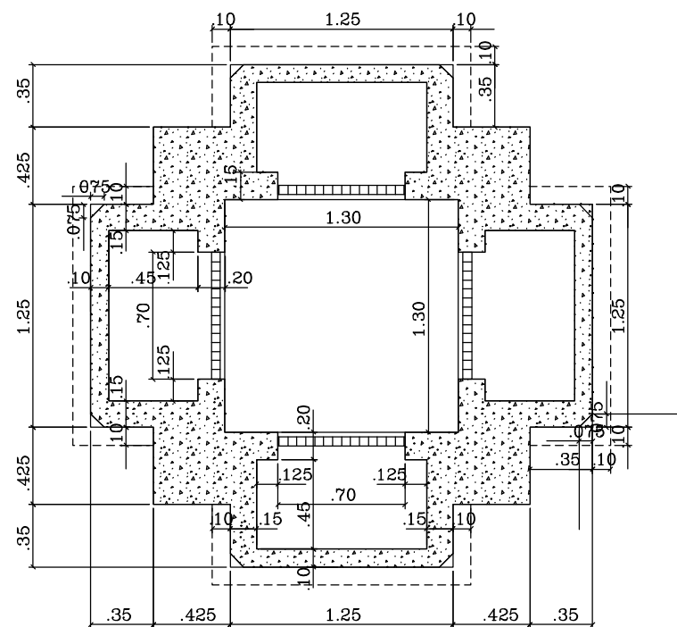
SECTION 3-3
