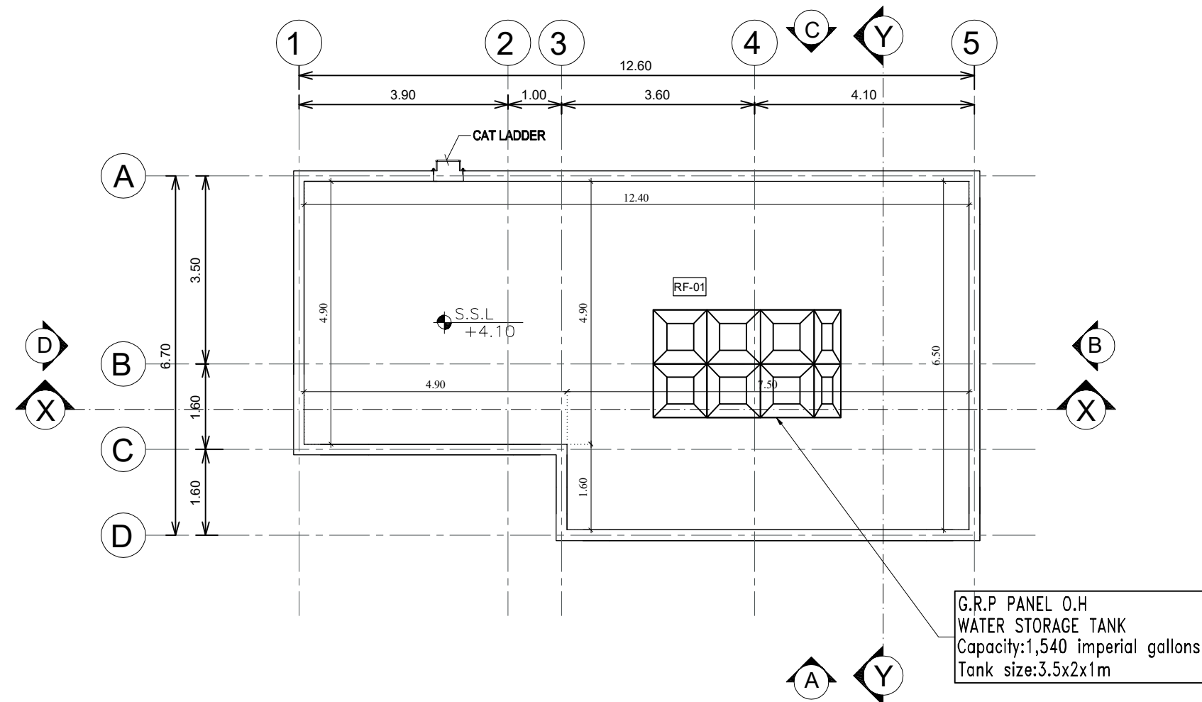
1 ABLUTION BLOCK ROOF PLAN SCALE : 1:100
