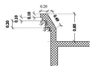
TYPICAL PARAPET DETAIL z-z
