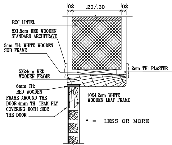
SECTIONAL DETAIL OF HOLLOW CORE DOOR
