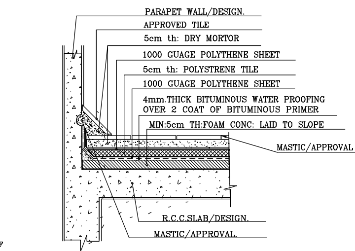
DETAIL-1
