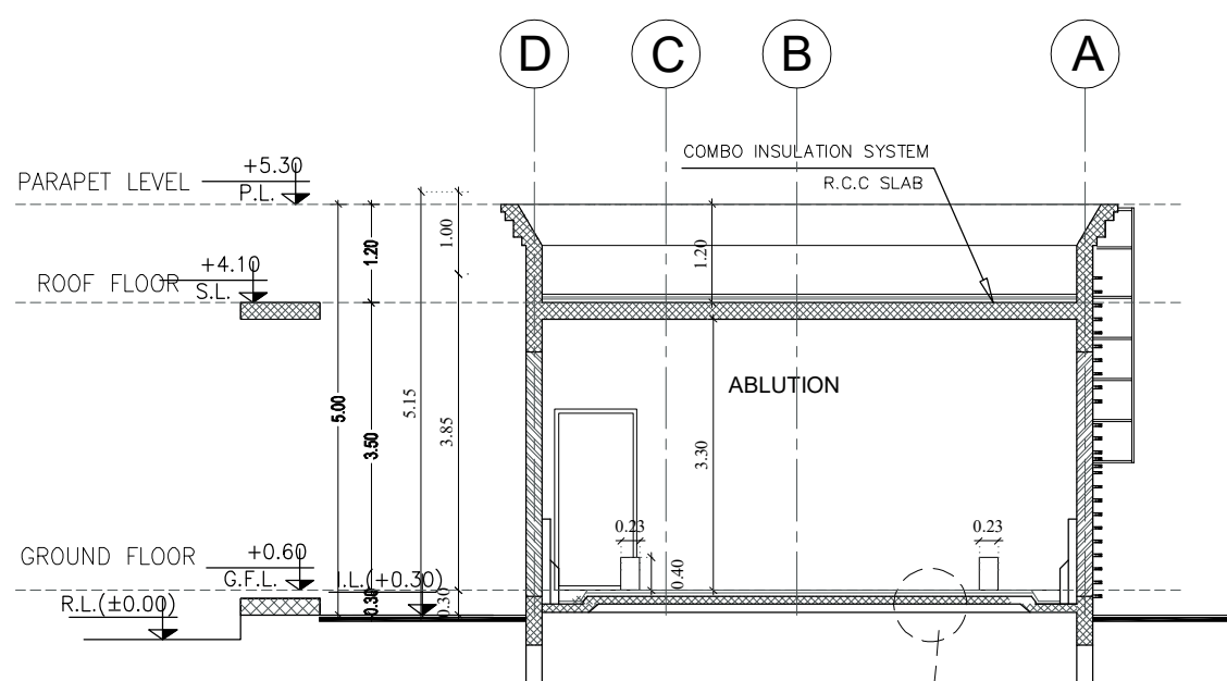
1 ABLUTION BLOCK SECTION Y-Y
