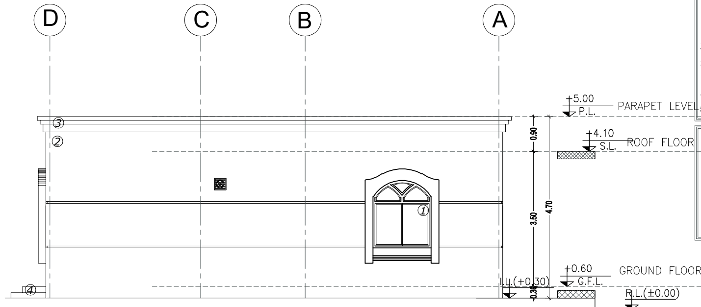
ELEVATION -B (SCALE = 1 : 100)
