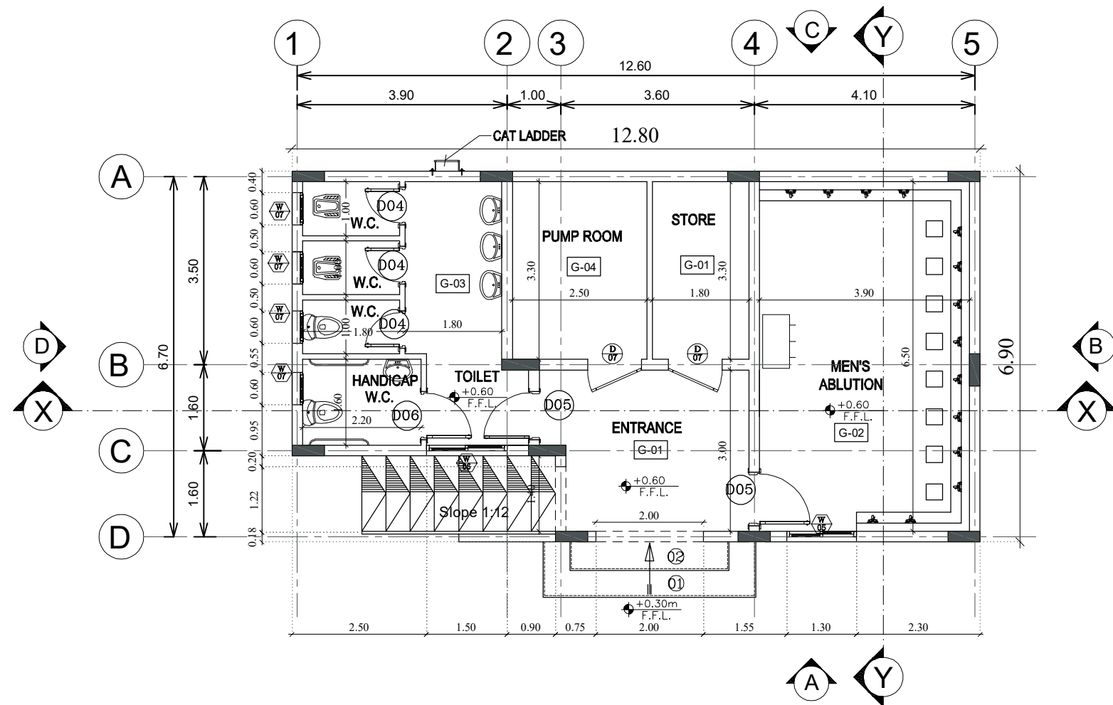
1 ABLUTION BLOCK GROUND FLOOR PLAN SCALE : 1:100
