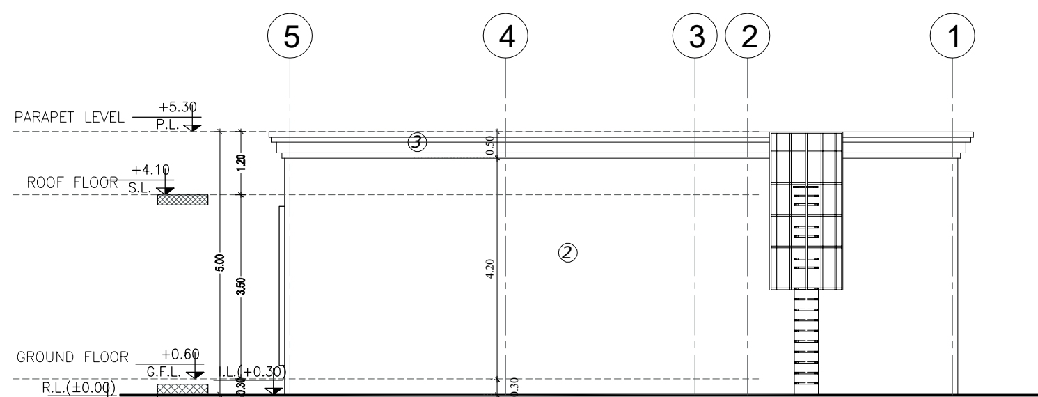
1 ABLUTION BLOCK ELEVATION C
