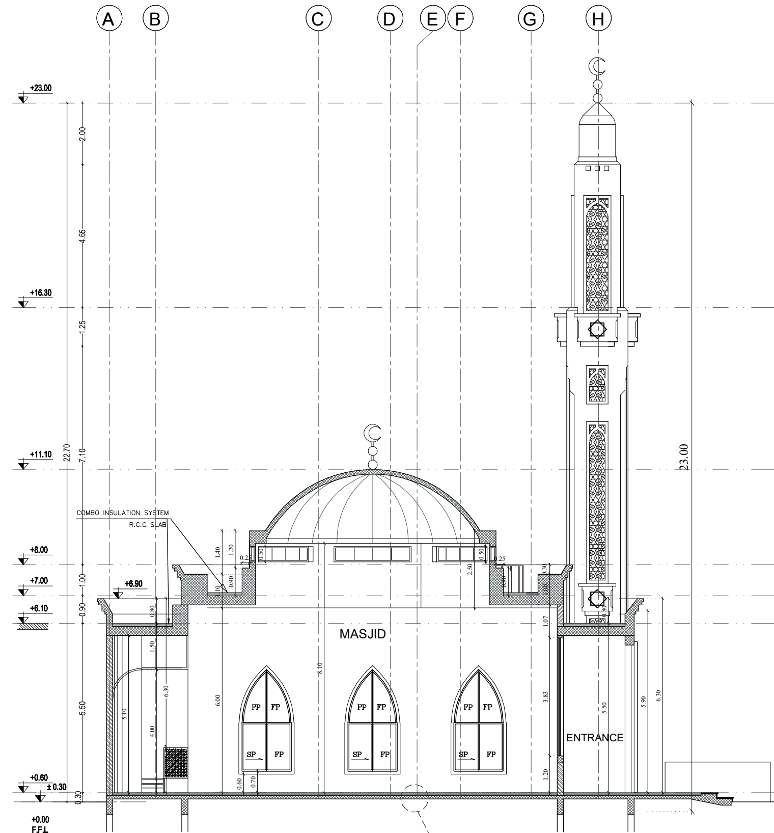
MASJID SECTION Y-Y
