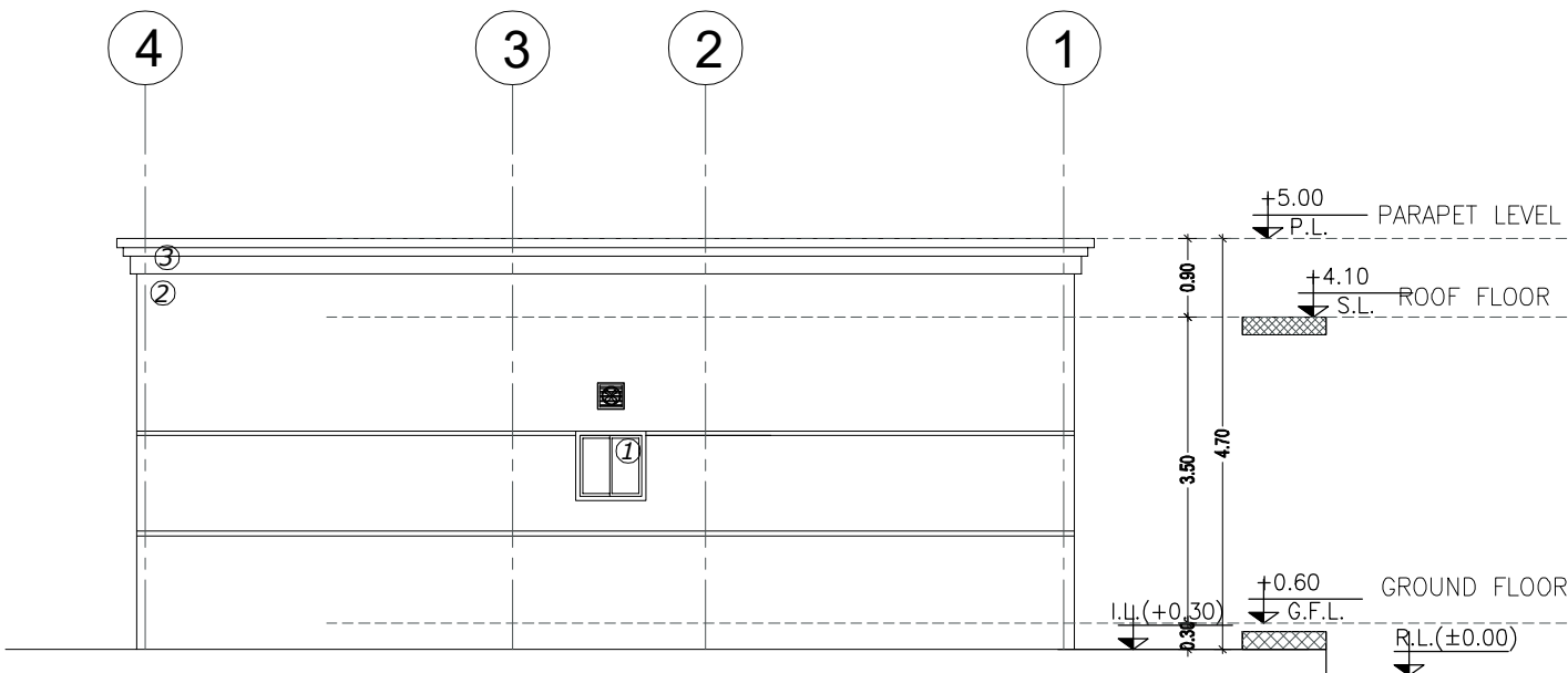
ELEVATION -C (SCALE = 1 : 100)
