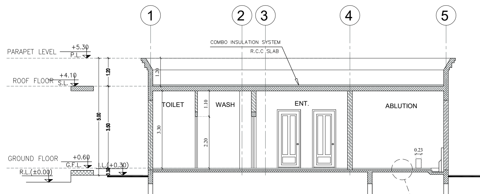
1 ABLUTION BLOCK SECTION X-X
