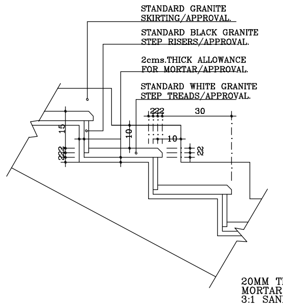
TYP: ENT: STEPS DETAIL
