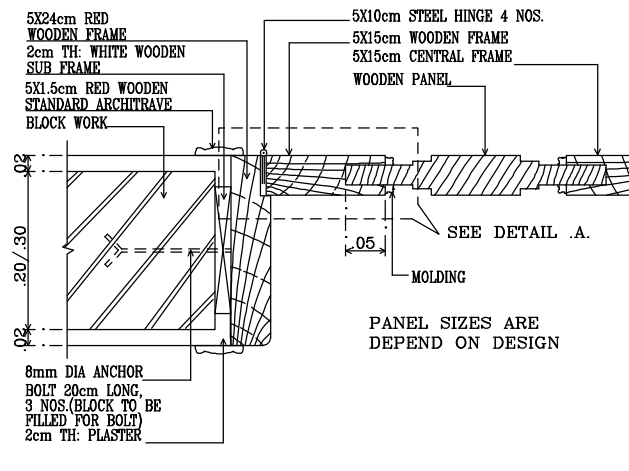
SECTIONAL DETAIL OF SOLID OR PANEL DOOR
