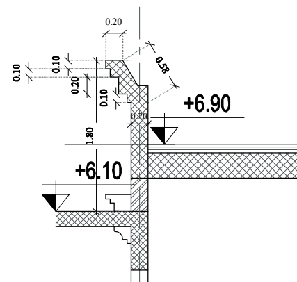
TYPICAL PARAPET DETAIL f-f
