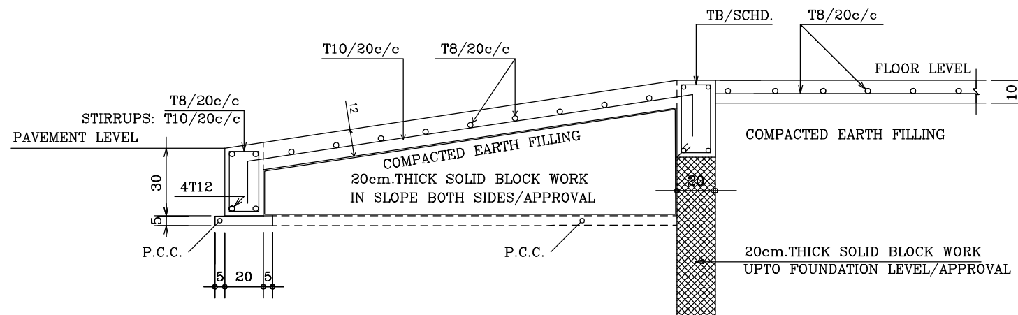
RAMP DETAIL
