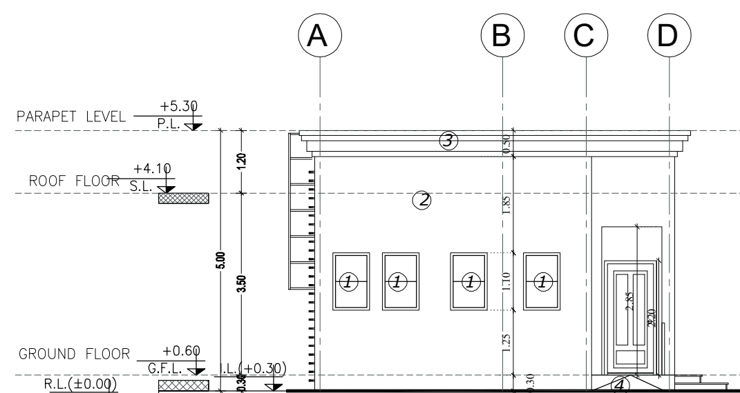
1 ABLUTION BLOCK ELEVATION D
