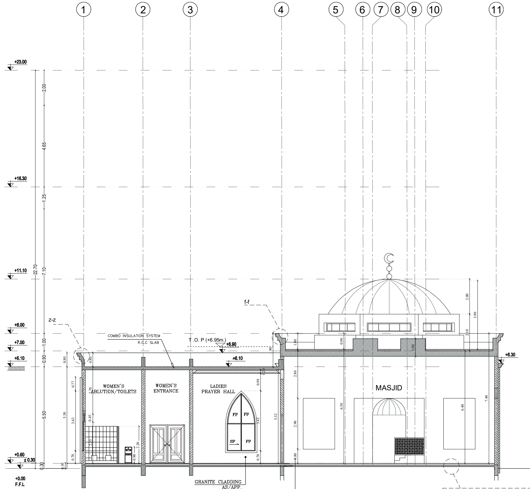
MASJID SECTION X-X
