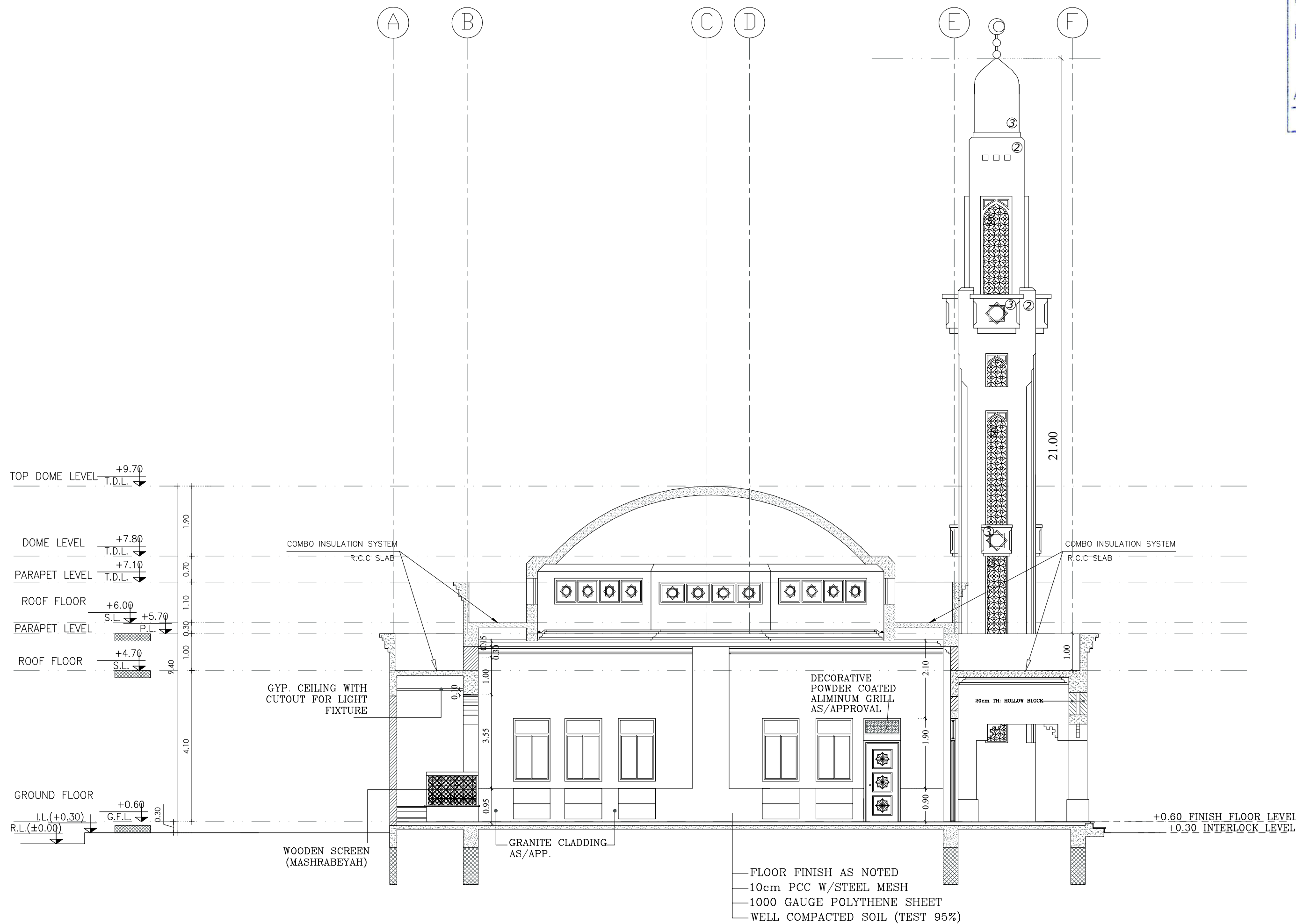
SECTION Y-Y
