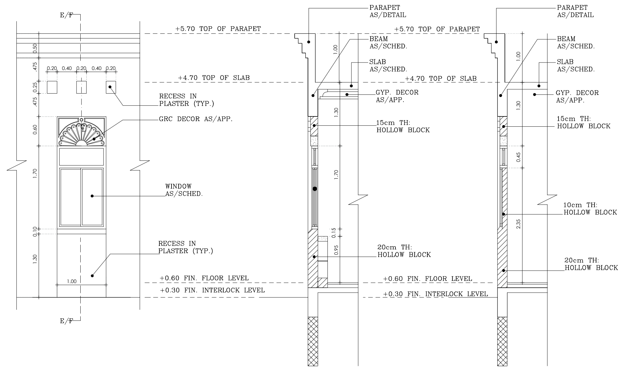
DETAIL AT W1/W4/W5
