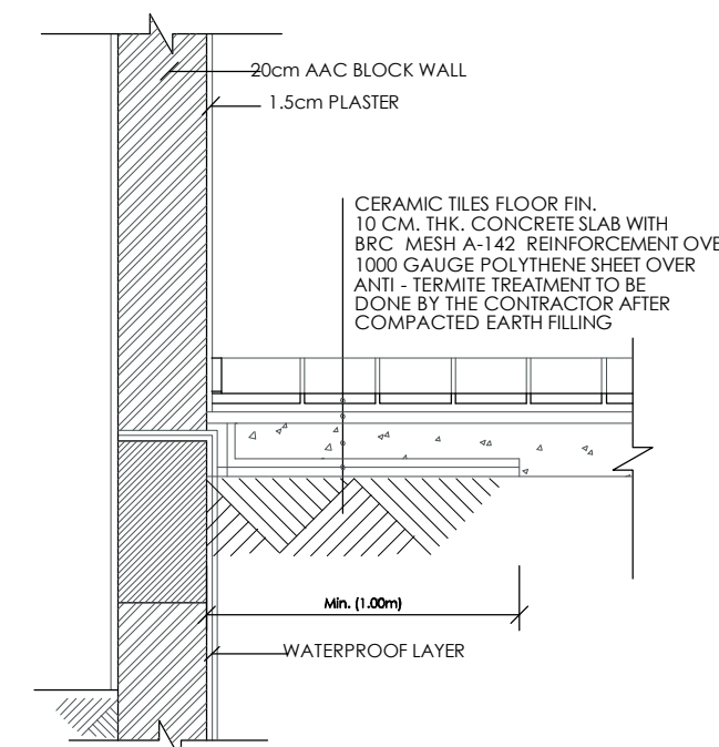
DETAIL 2 (SCALE = 1 : 25)
