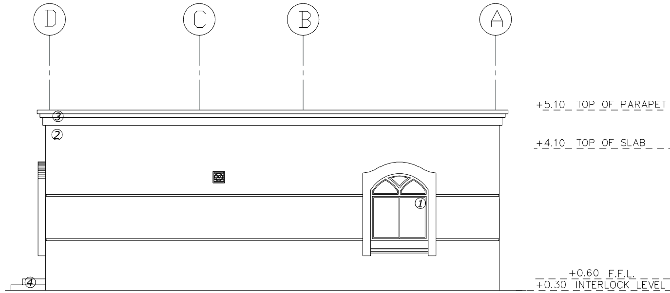
ELEVATION -B (SCALE = 1 : 100)
