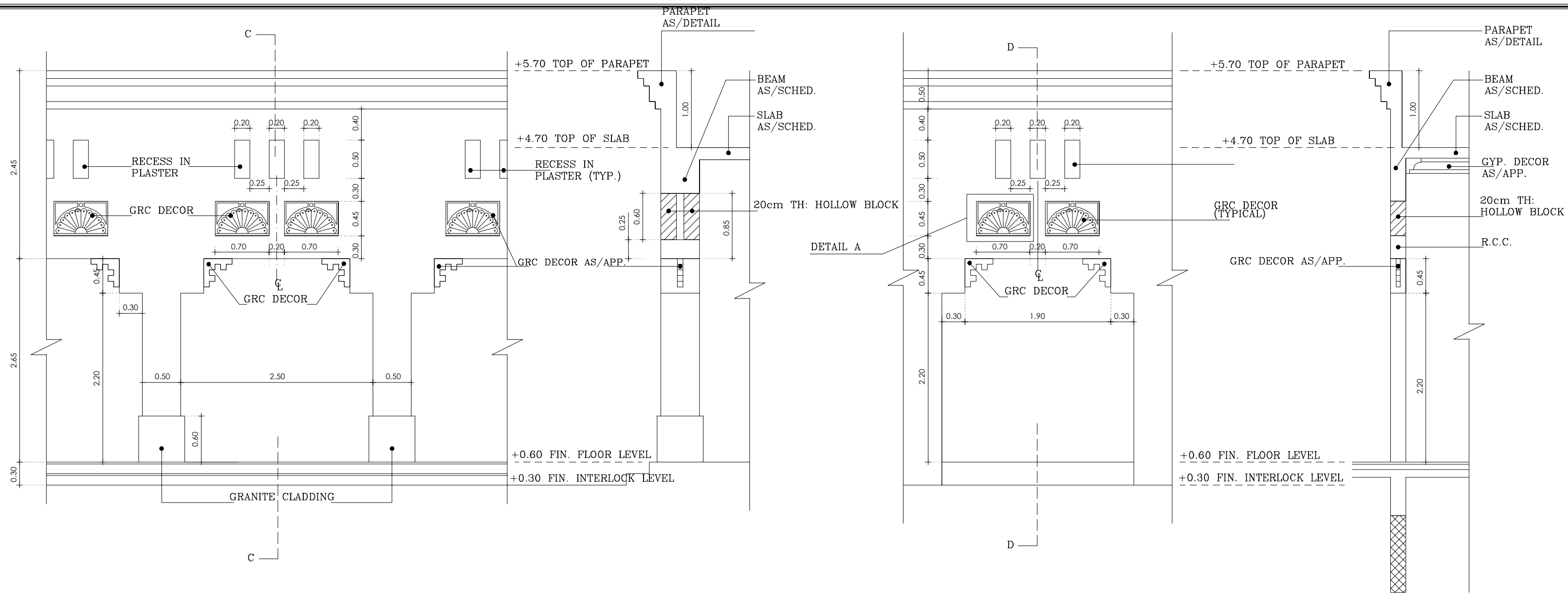
TYP. DETAIL AT FRONT ENTRANCE – MAIN MOSQUE
