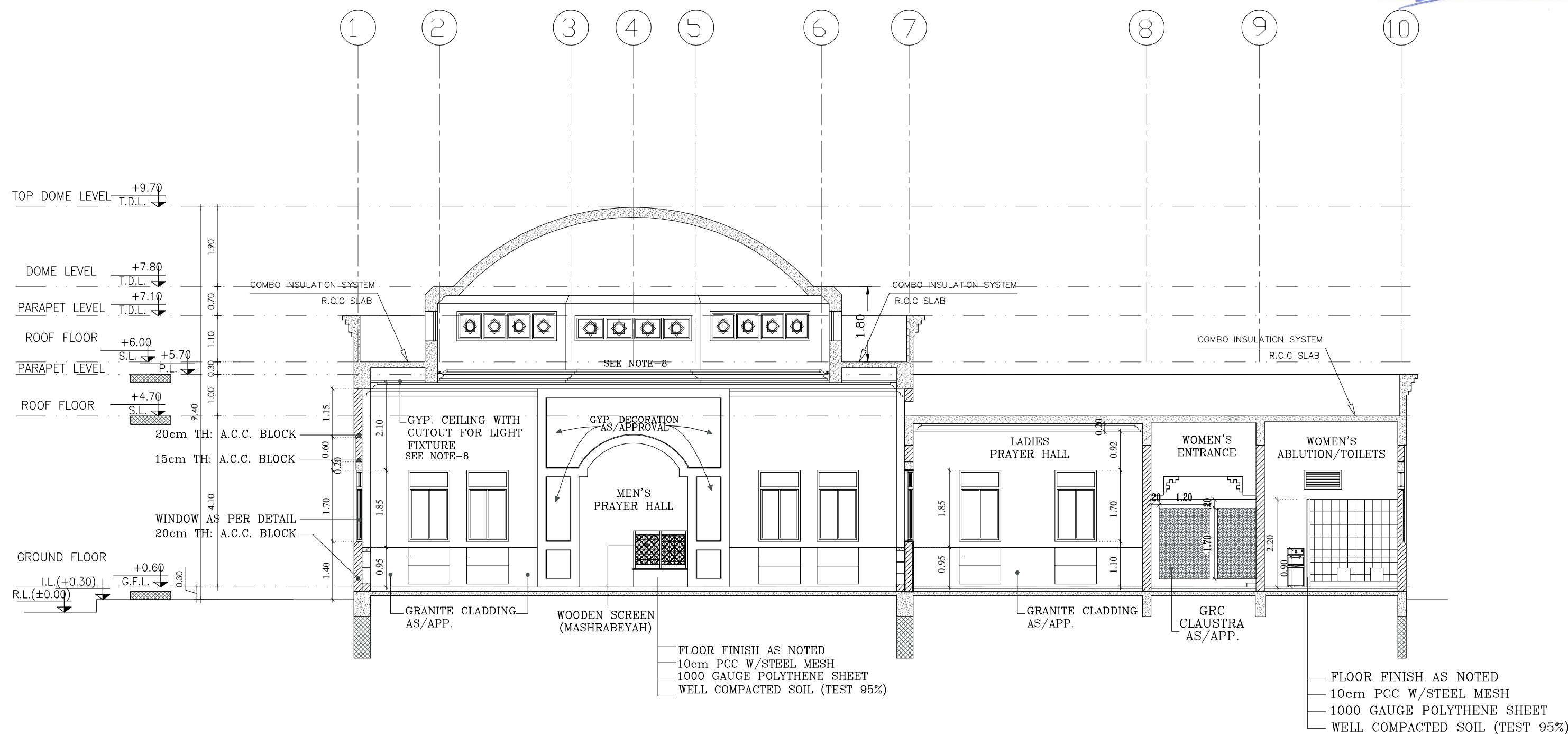
SECTION X-X
