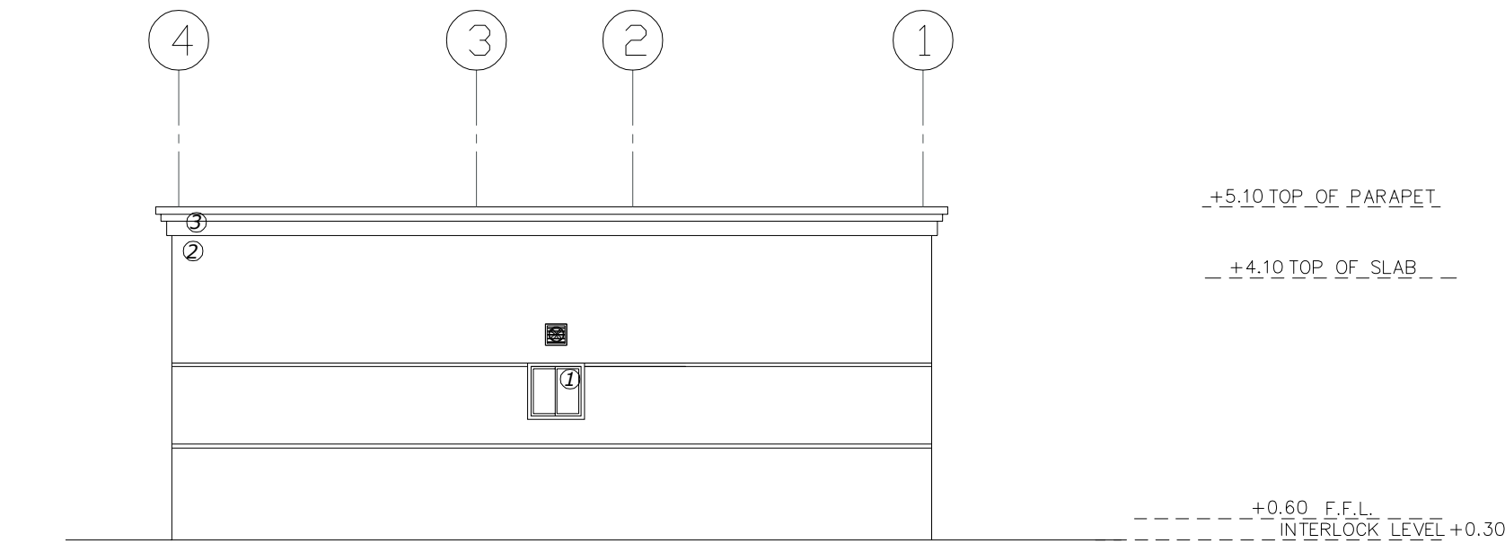
ELEVATION -C (SCALE = 1 : 100)
