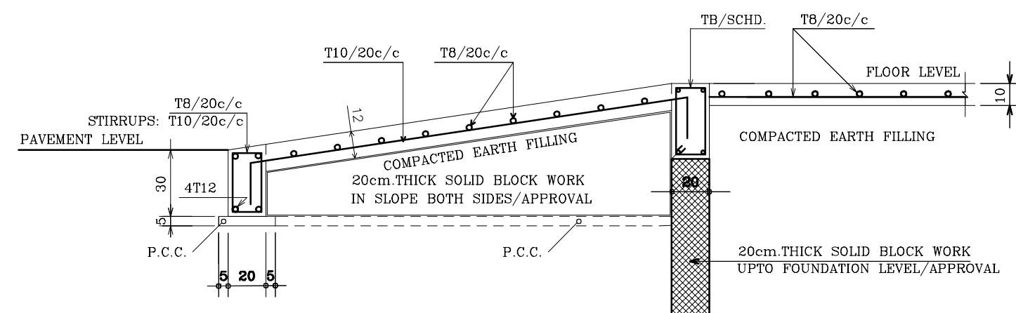
RAMP DETAIL
