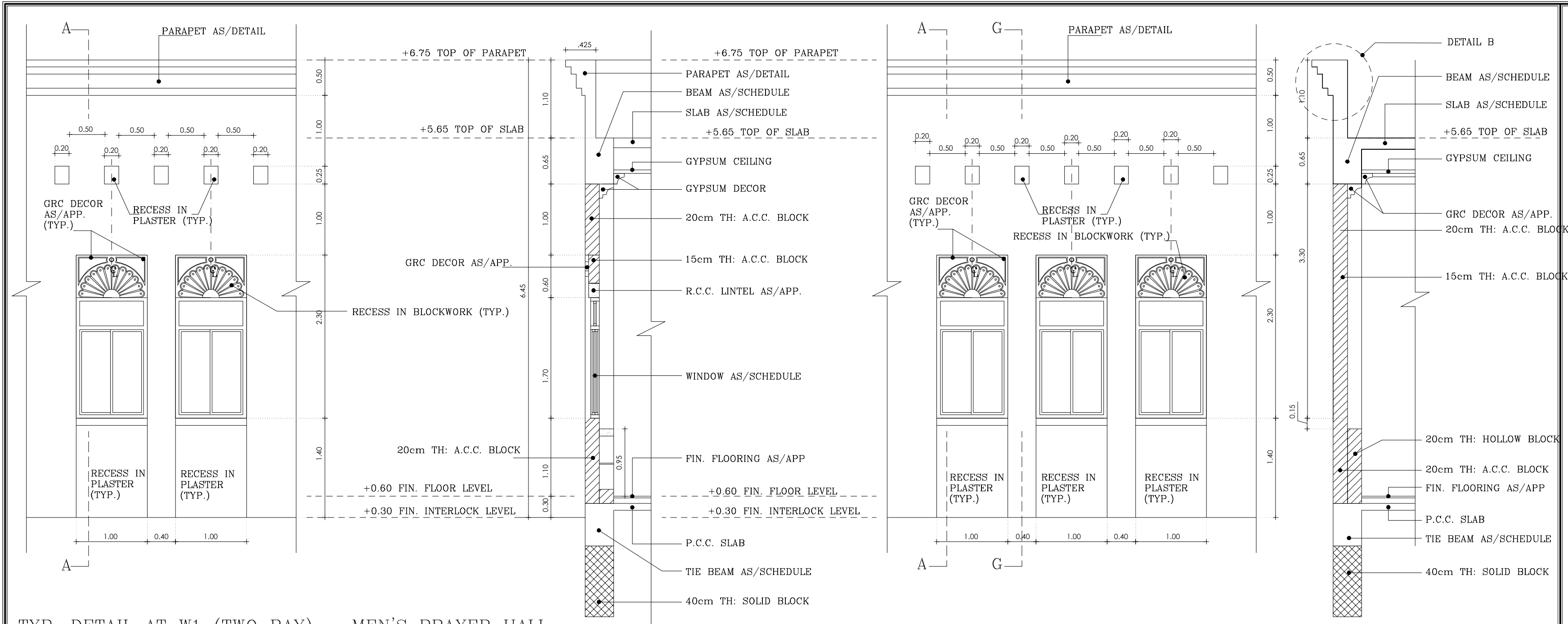
TYP. DETAIL AT W1 (TWO BAY) – MEN’S PRAYER HALL
