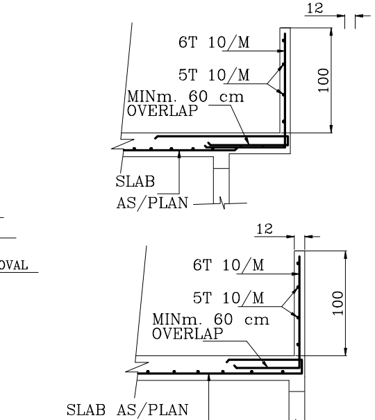
RCC PARAPET WALL FINISHES AS PER PWD ENG.APPROVAL
