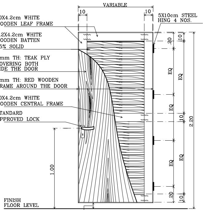
ELEVATIONAL DETAIL OF HOLLOW CORE DOOR
