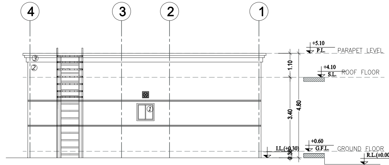
ELEVATION -C
