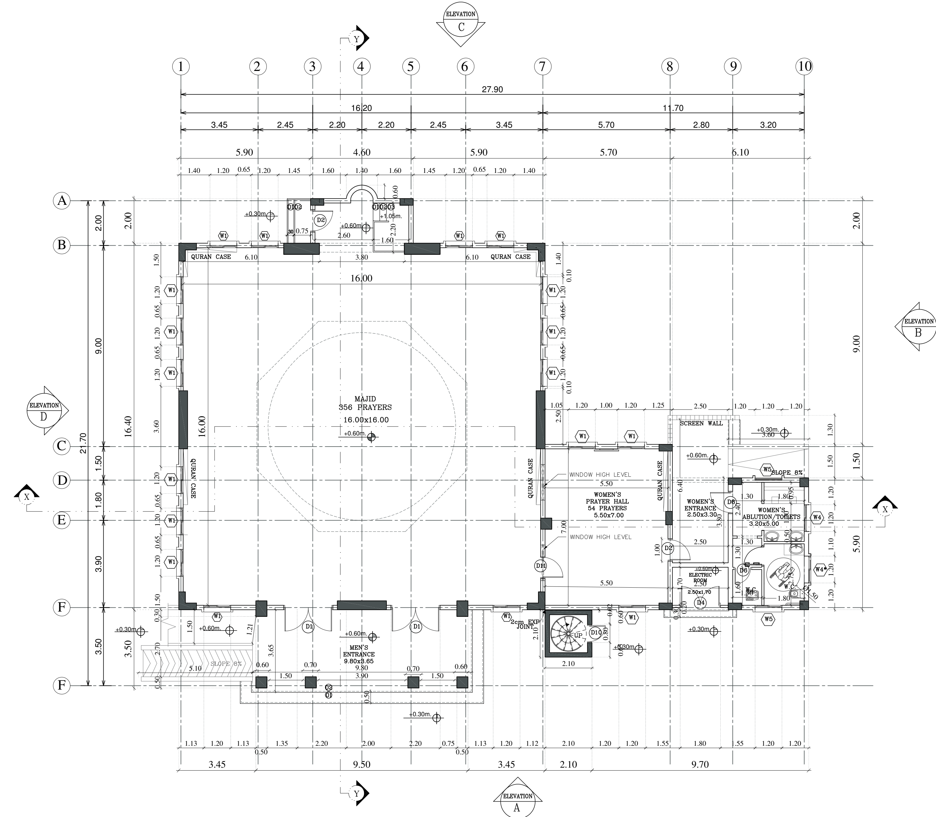
GROUND FLOOR PLAN ( SCALE = 1 : 100 )
