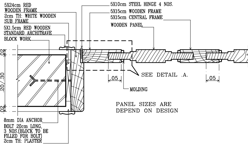
SECTIONAL DETAIL OF SOLID OR PANEL DOOR
