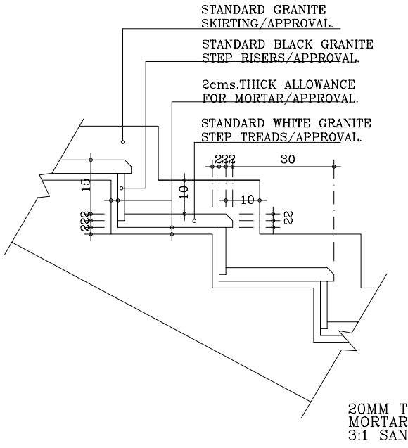
TYP: ENT: STEPS DETAIL
