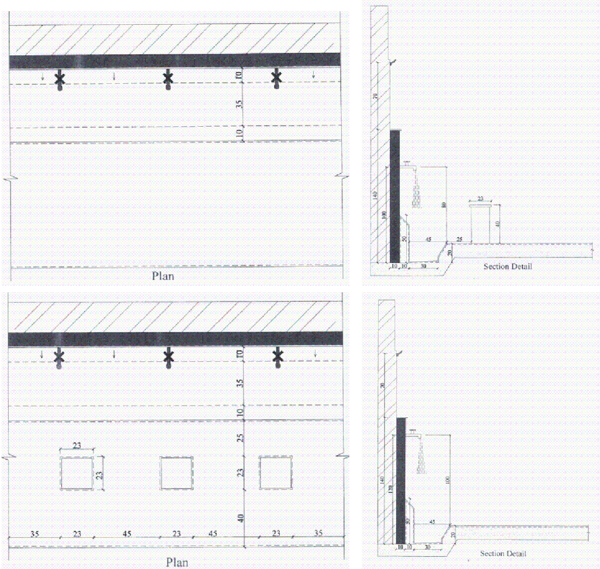
ABLUTION DETAIL
