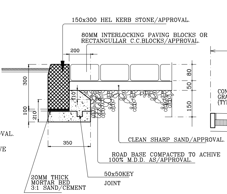
TYPICAL DETAIL FOR DRIVE WAY
