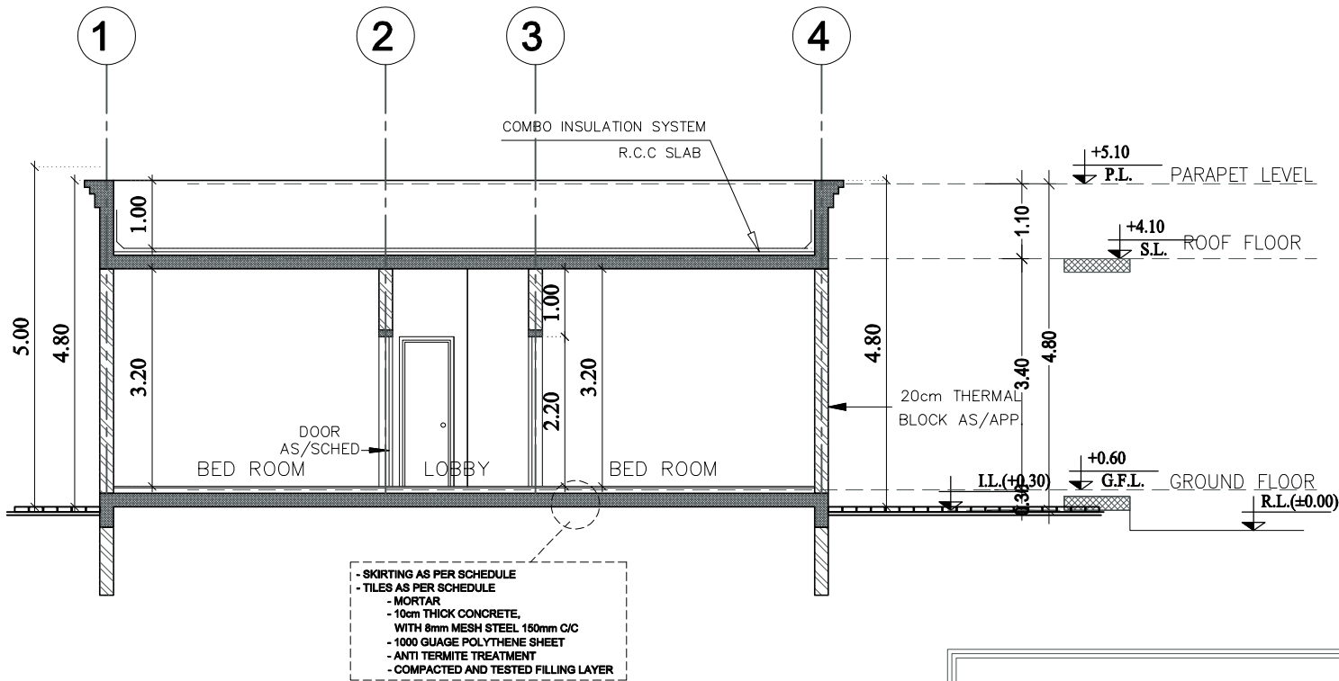
SECTION Y-Y
