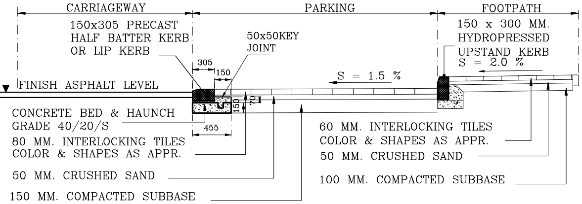
DETAIL OF FOOTPATH & PARKING
