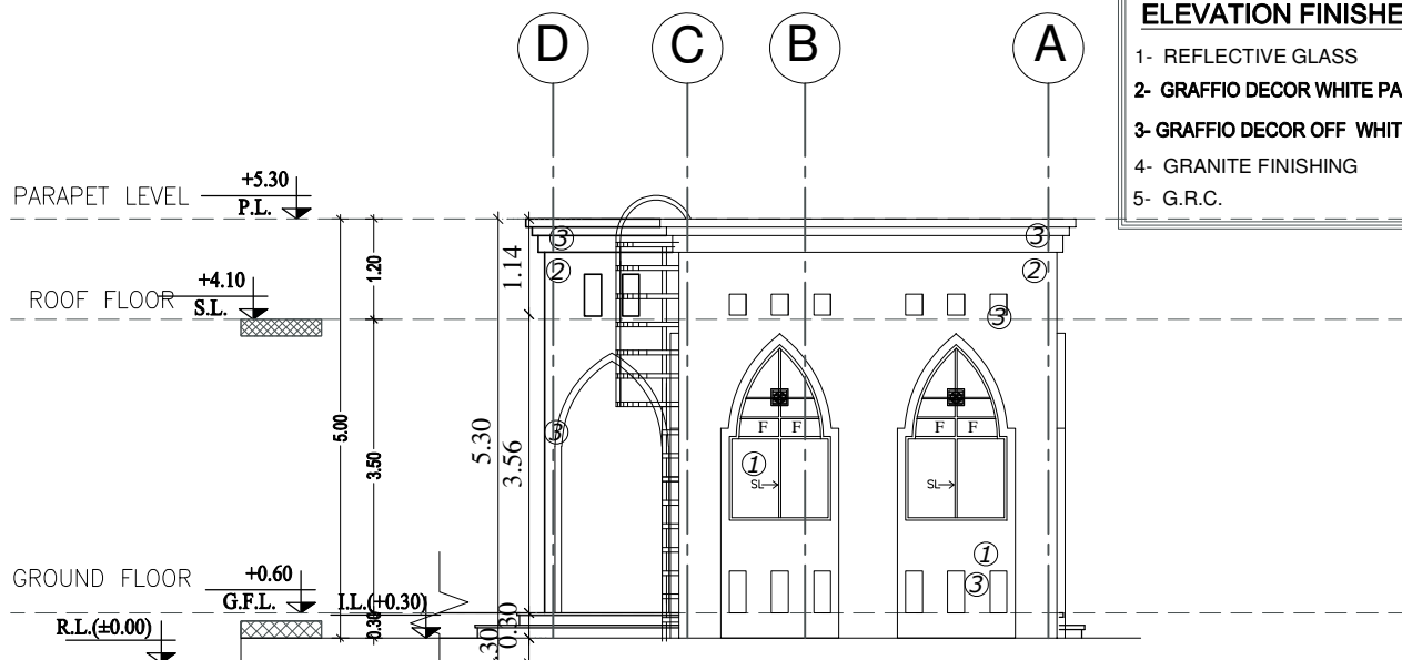
ELEVATION -B ( SCALE = 1 : 100 )
