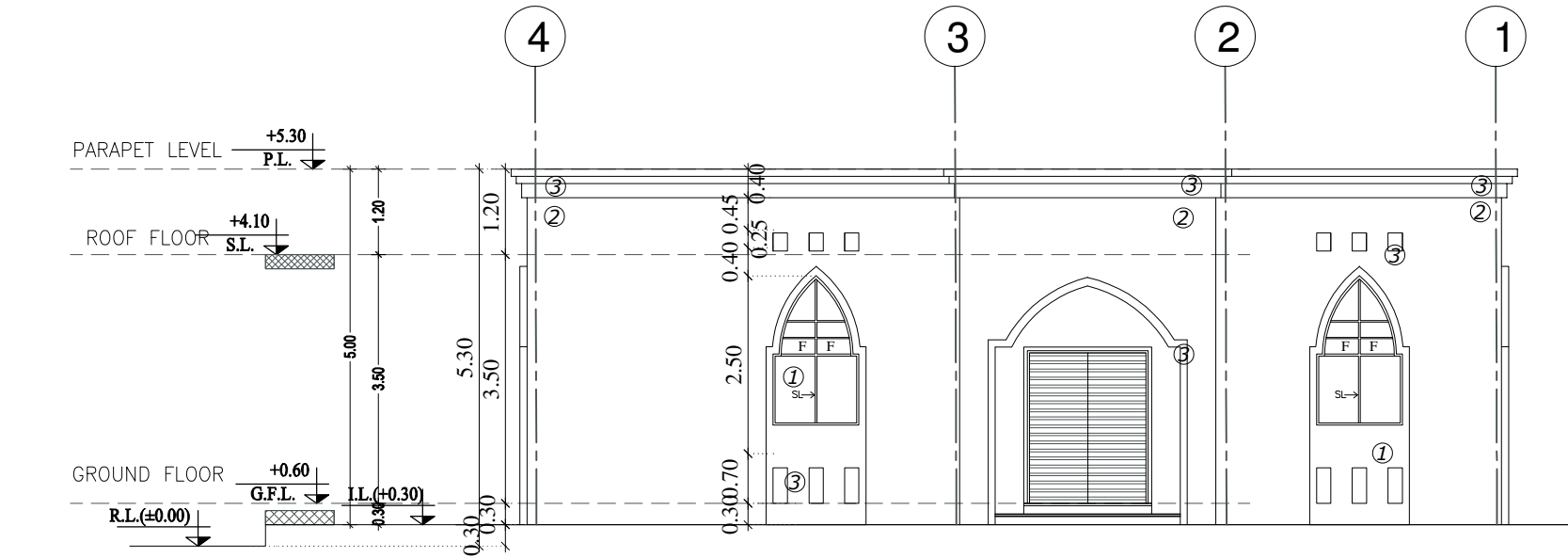
ELEVATION -C ( SCALE = 1 : 100 )
