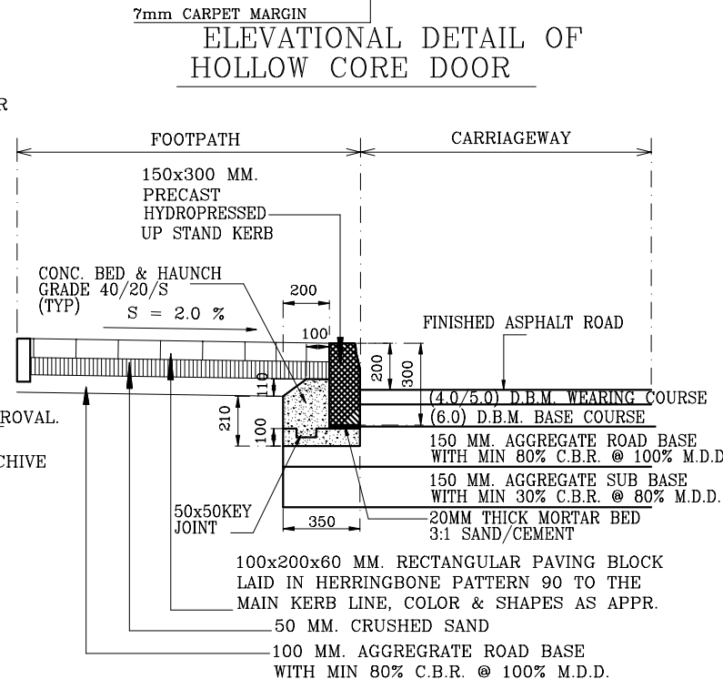
DETAIL OF FOOTPATH
