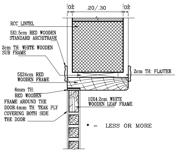
SECTIONAL DETAIL OF HOLLOW CORE DOOR
