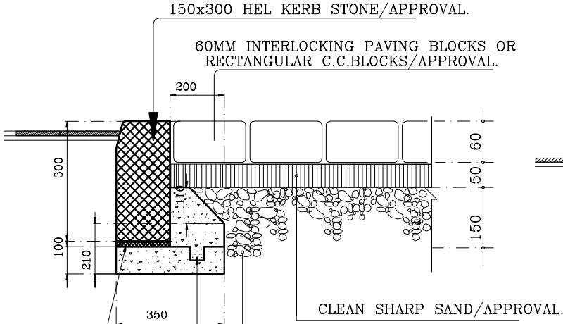
TYPICAL DETAIL FOR INTER LOCKING
