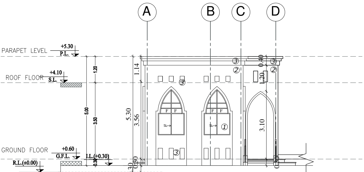
ELEVATION -D ( SCALE = 1 : 100 )
