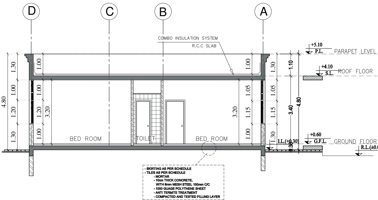
SECTION X-X
