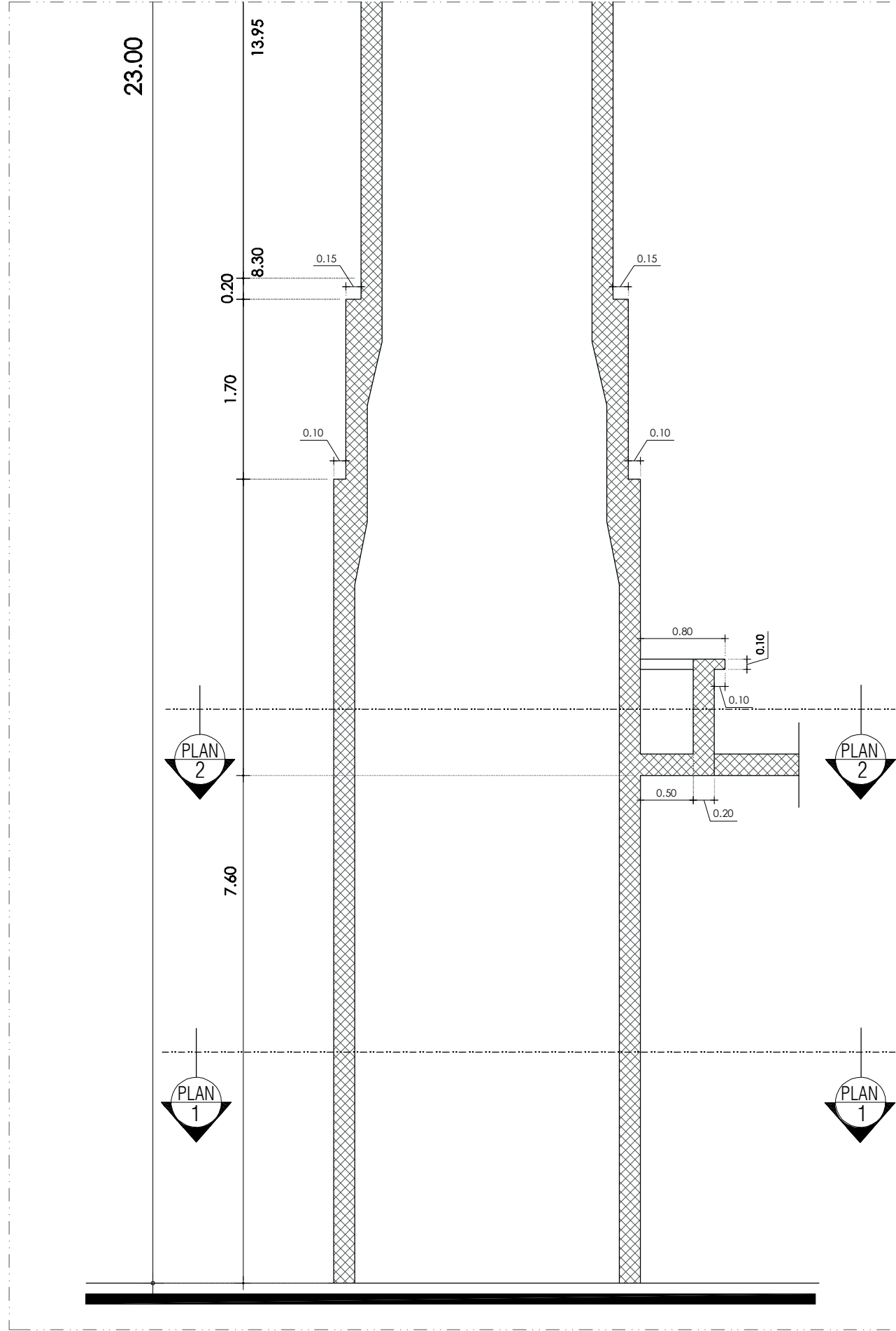
SECTION Y-Y ( SCALE = 1 : 50 )
