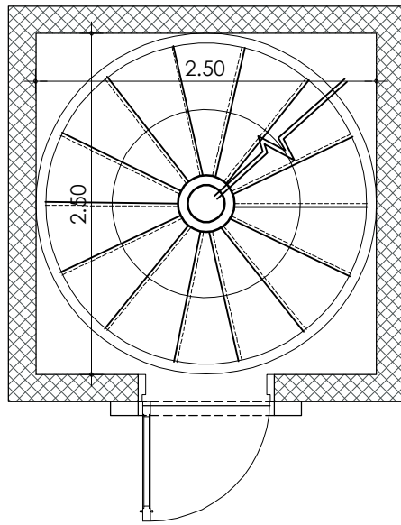
PLAN -1 ( SCALE = 1 : 50 )
