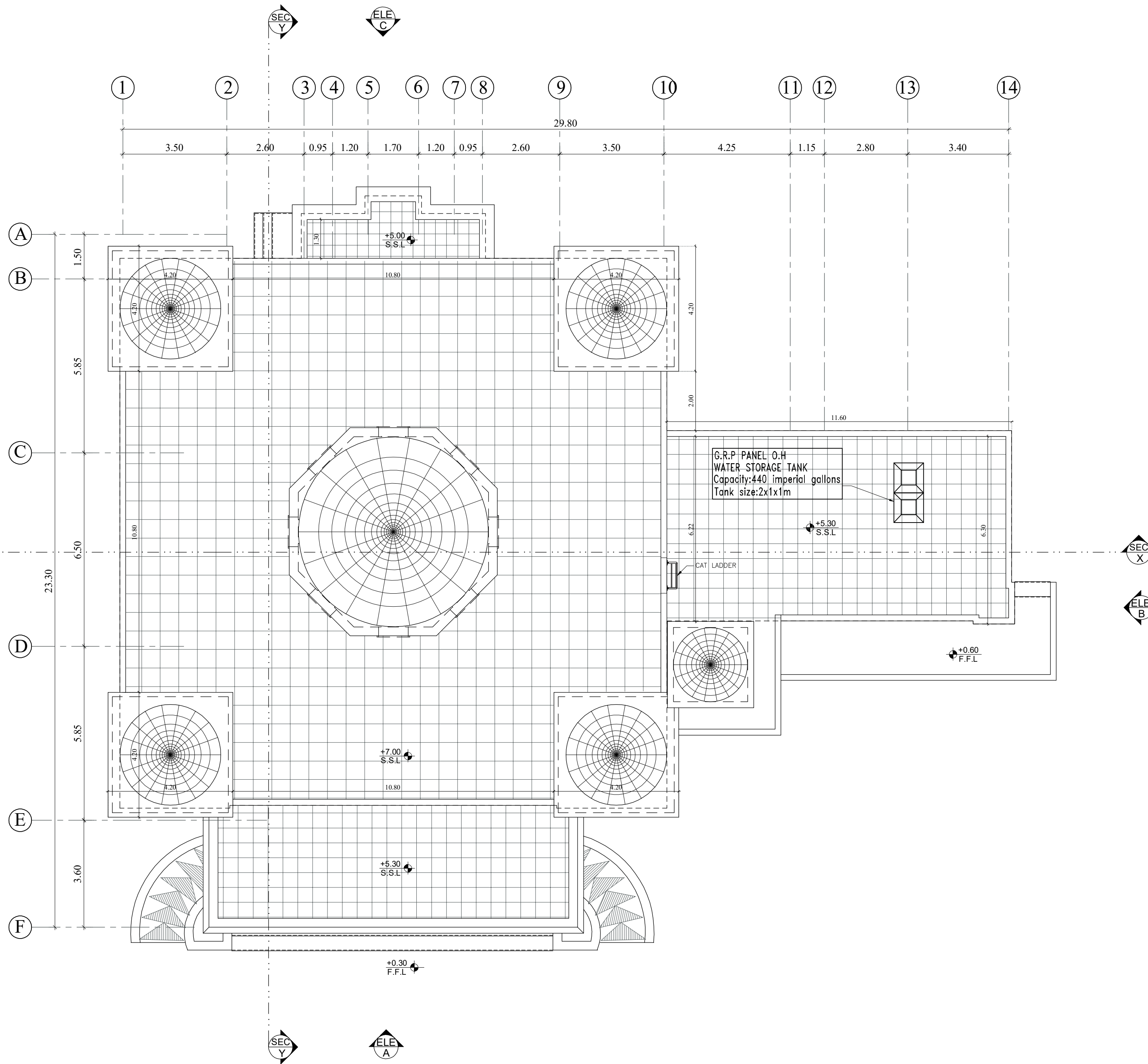
TOP ROOF FLOOR PLAN SCALE 1:100
