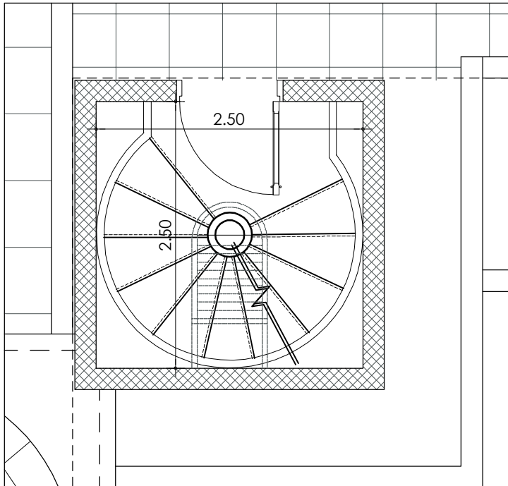
PLAN -2 ( SCALE = 1 : 50 )
