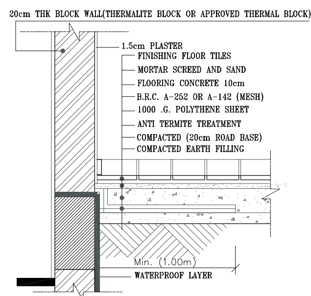
GROUND FLOOR DETAILS
