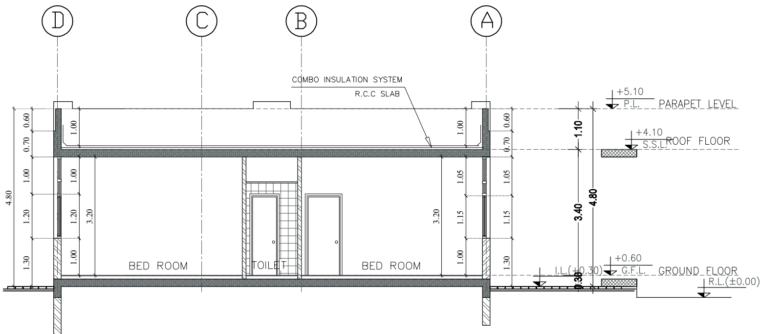
SECTION Y-Y
