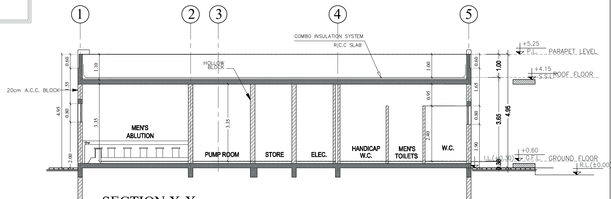
SECTION X-X
