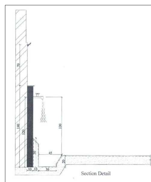
SECTION X-X
