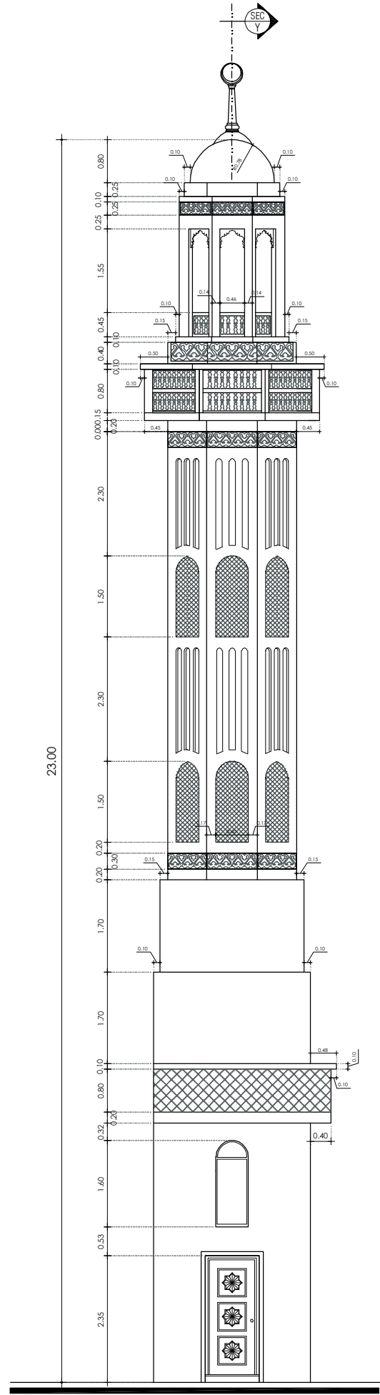
MANAR ELEVATION ( SCALE = 1 : 100 )
