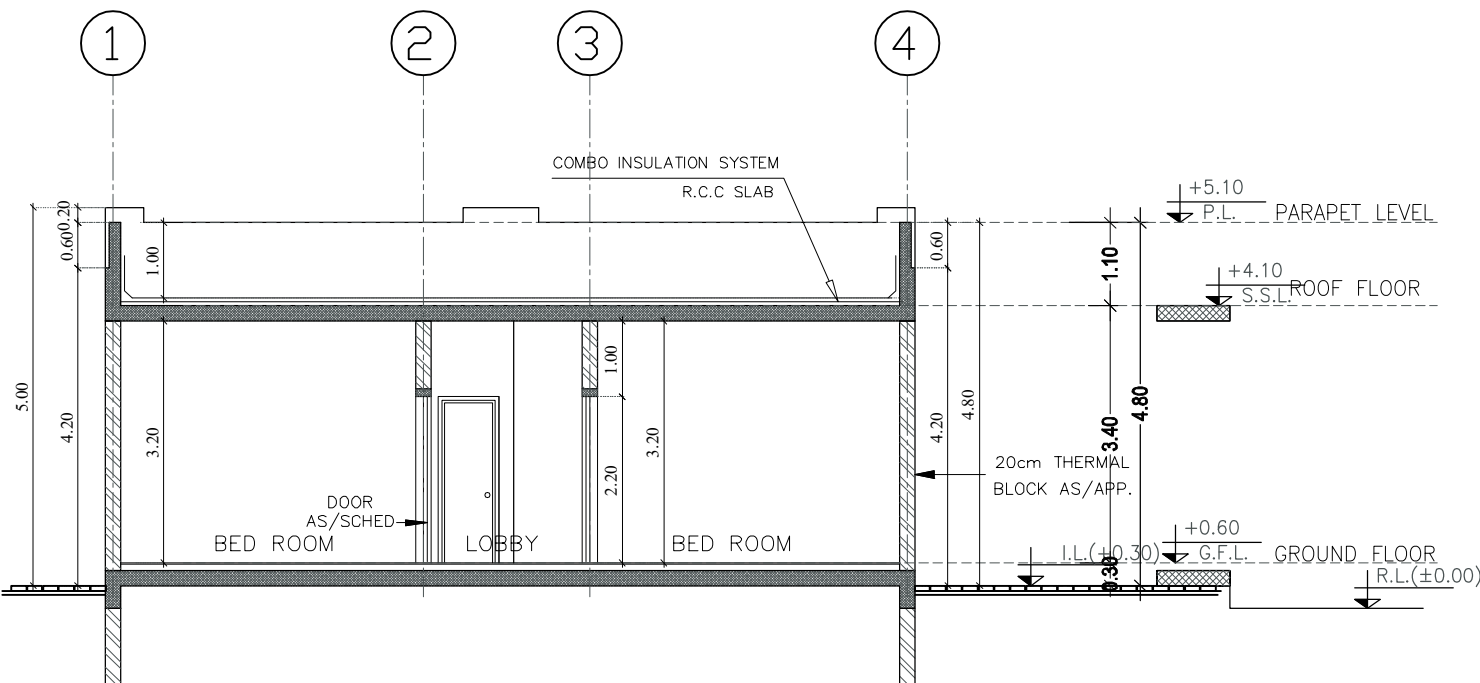
SECTION X-X
