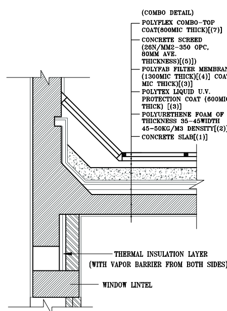
PARAPET & ROOF FINISHING DETAILS
