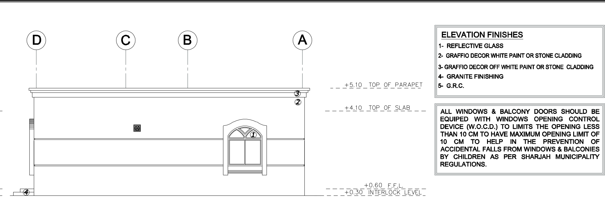
ELEVATION -B (SCALE = 1 : 100)
