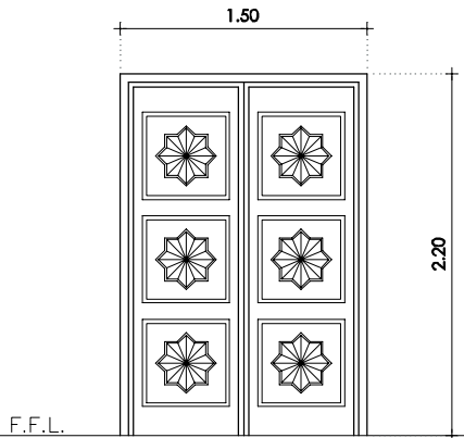
WOODEN DOUBLE LEAF DECORATIVE SOLID PANEL AS PER APPROVAL
