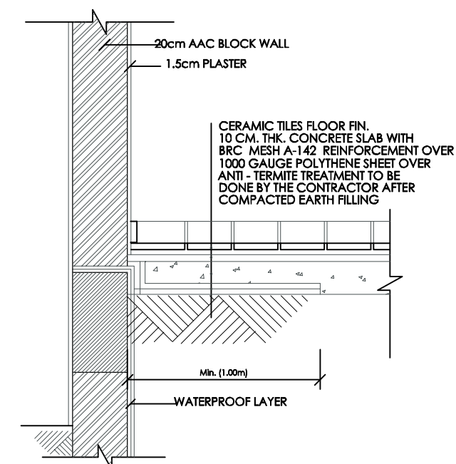
DETAIL 2 ( SCALE = 1 : 25 )
