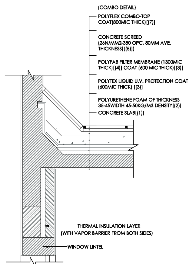
DETAIL 1 ( SCALE = 1 : 25 )
