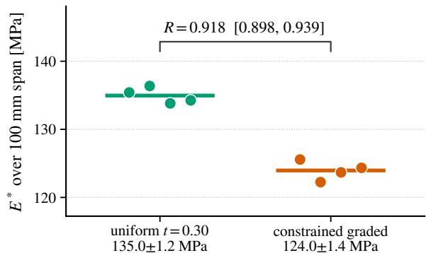
(c) Per-specimen E^* and ratio R
