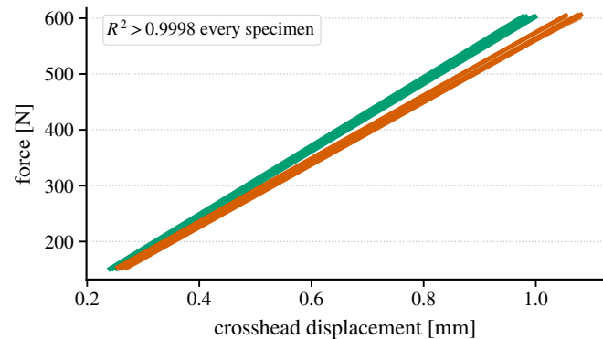
(b) Elastic-window fits
