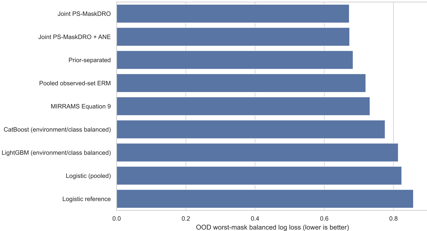
Independent patient-disjoint readmission result
