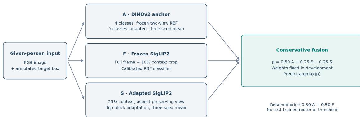
Figure 1. Person-centric branches and development-fixed probability fusion.
