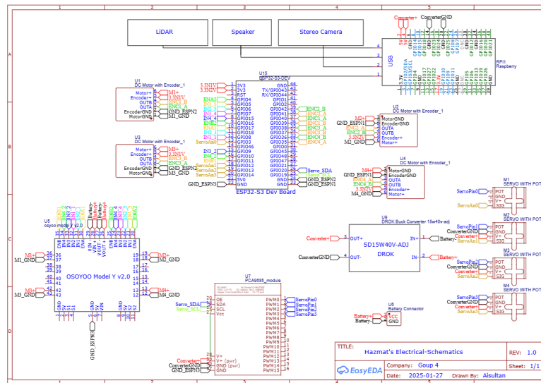
Figure 22: Previous schematics
