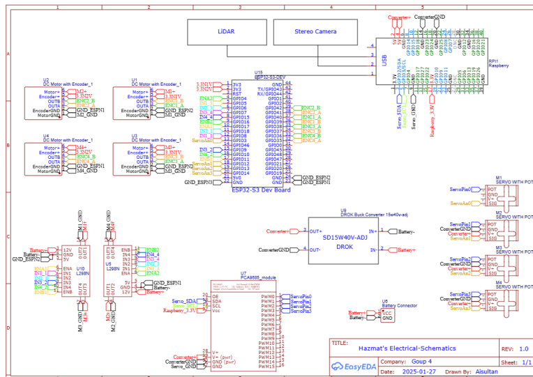
Figure 20: current schematics
