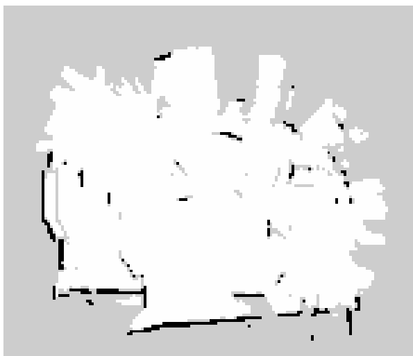
Figure 22: 2D occupancy map of the East end of the EE lab
