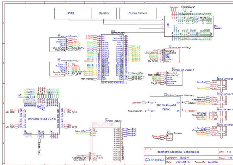
Figure 19: Previous schematics
