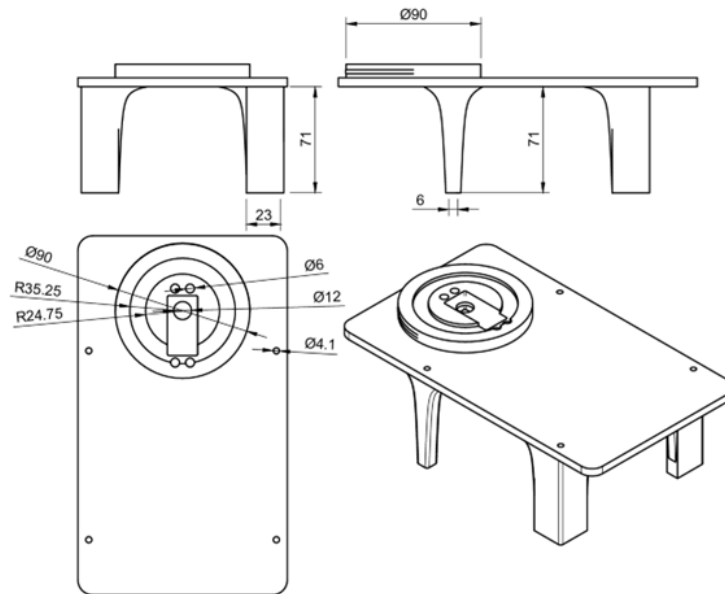
Figure 8: Engineering drawing of the top plate
