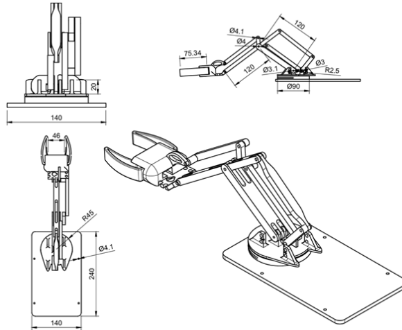
Figure 12: Engineering drawing of the arm
