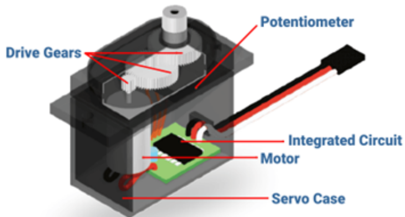
Figure 13: Servomotor working principle
