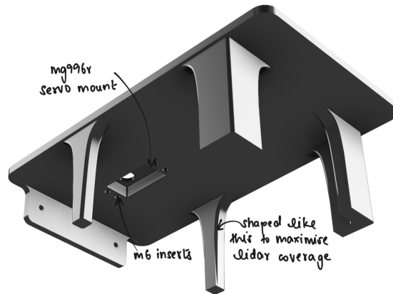
Figure 7: Another view of the top plate
