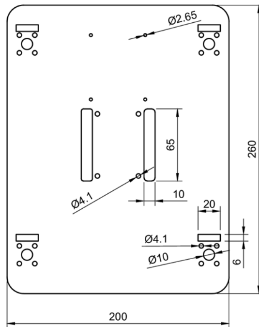
Figure 5: Engineering drawing of the base plate
