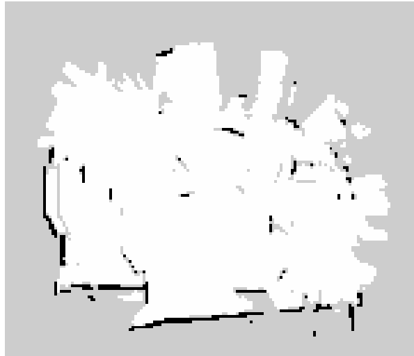
Figure 23: 2D occupancy map of the East end of the EE lab
