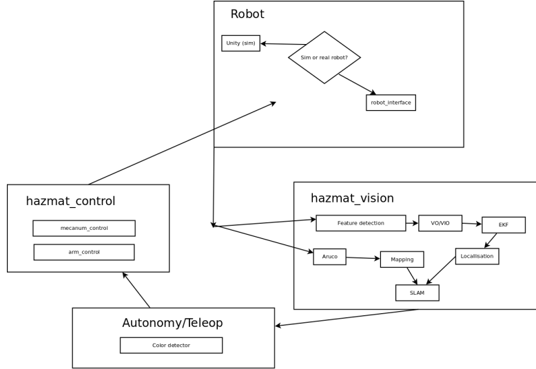
Figure 15: High level overview of the ROS nodes and topics
