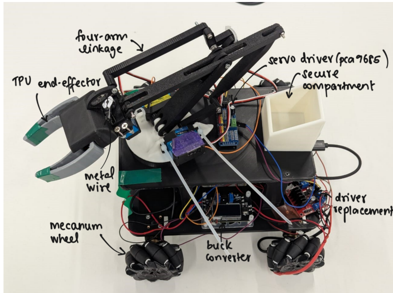
Figure 10: The final assembly
