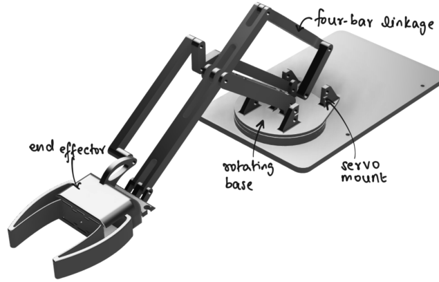
Figure 11: 3D render of the base arm
