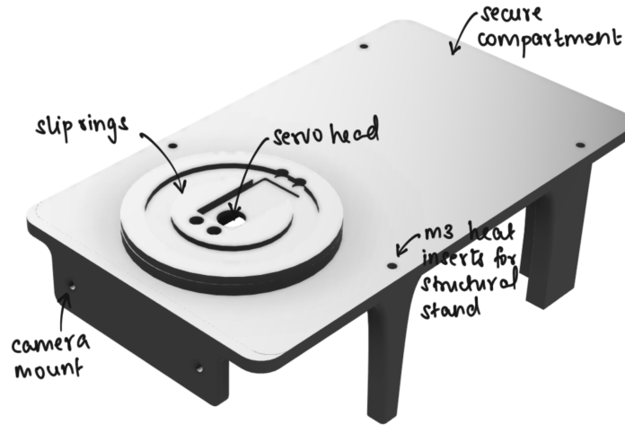
Figure 6: 3D render of the top plate
