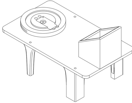
Figure 9: Top plate with payload compartment
