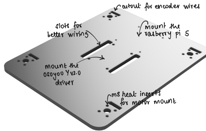
Figure 4: 3D render of the base plate
