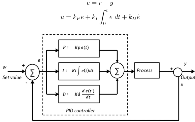
Figure 3: Block diagram of PID control
