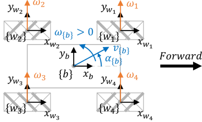
Figure 2: A common 4-wheeled mecanum configuration
