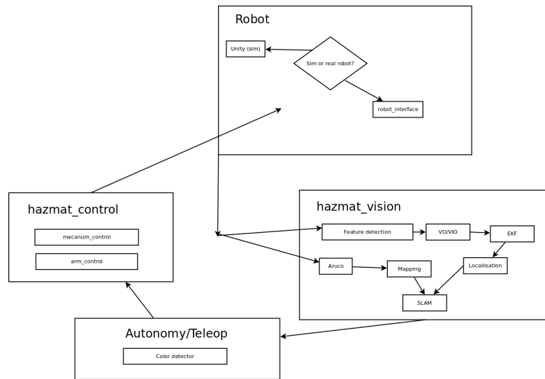
Figure 1: High level overview of the ROS nodes and topics
