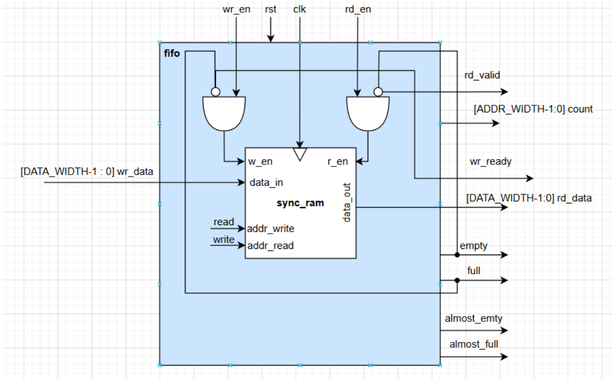
Block Diagram
