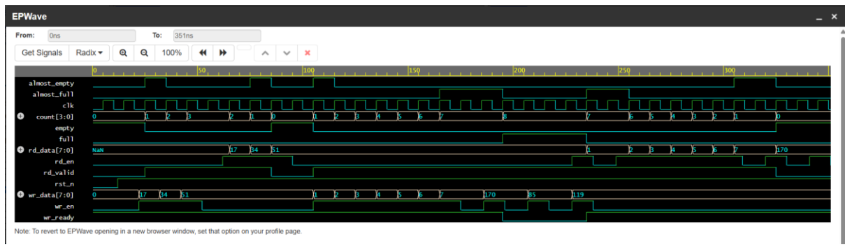
Waveform Screenshot
