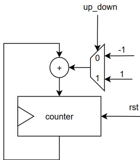
4-bit Updown Counter
