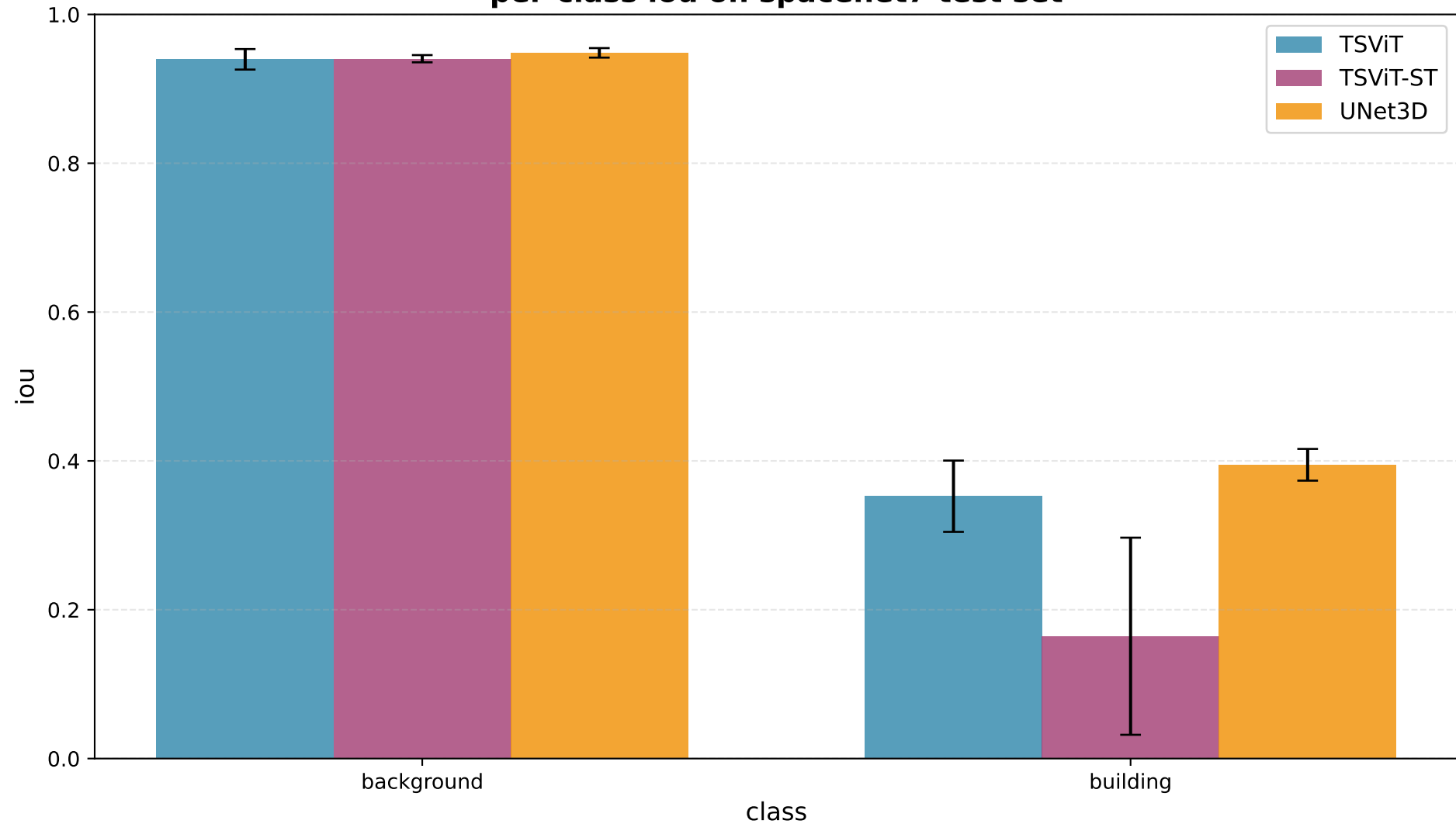
per-class iou on spacenet7 test set
