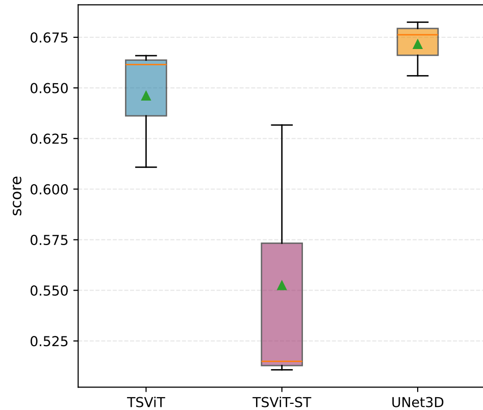
IoU
