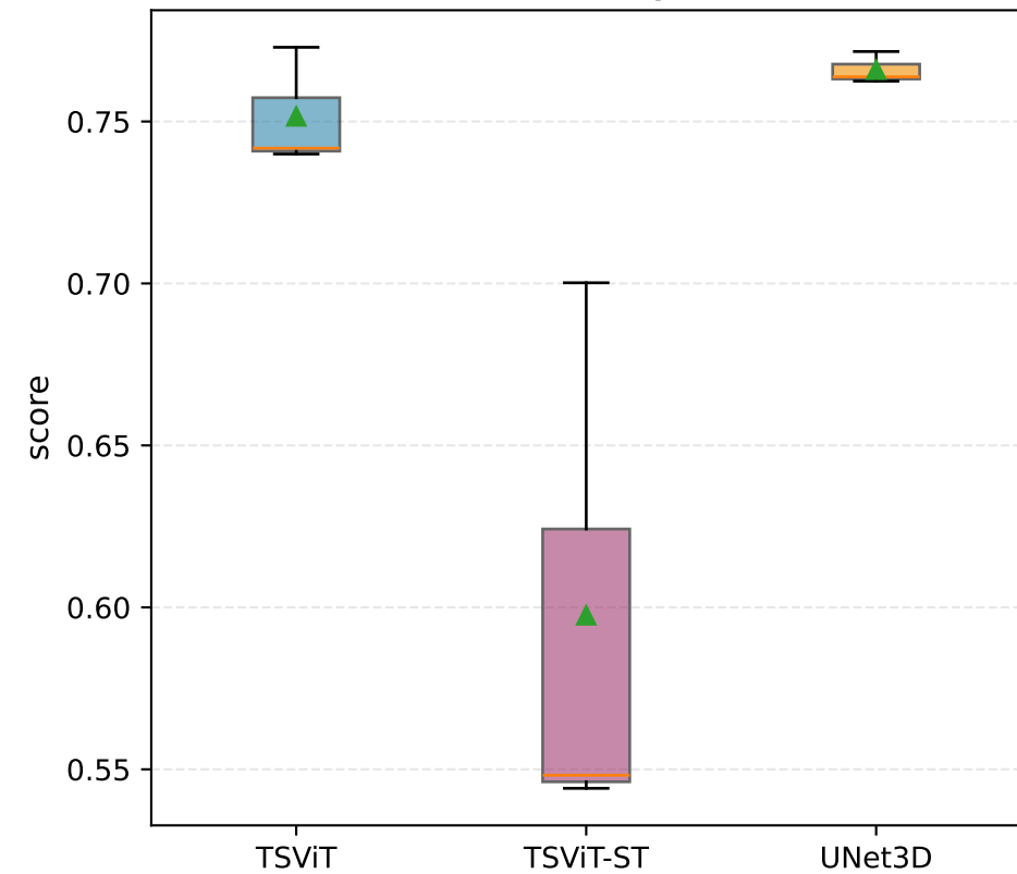
Accuracy
