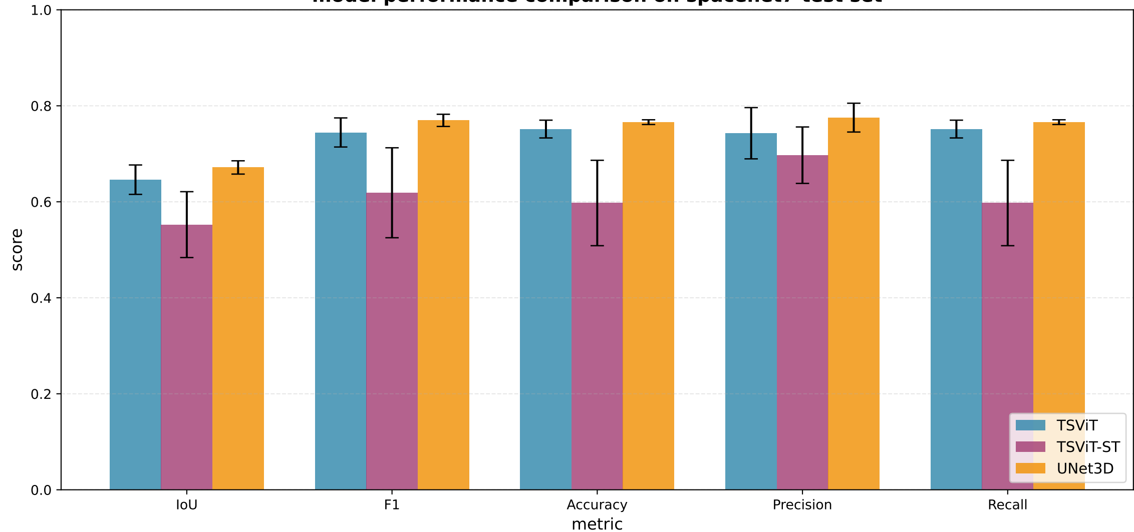
model performance comparison on spacenet7 test set
