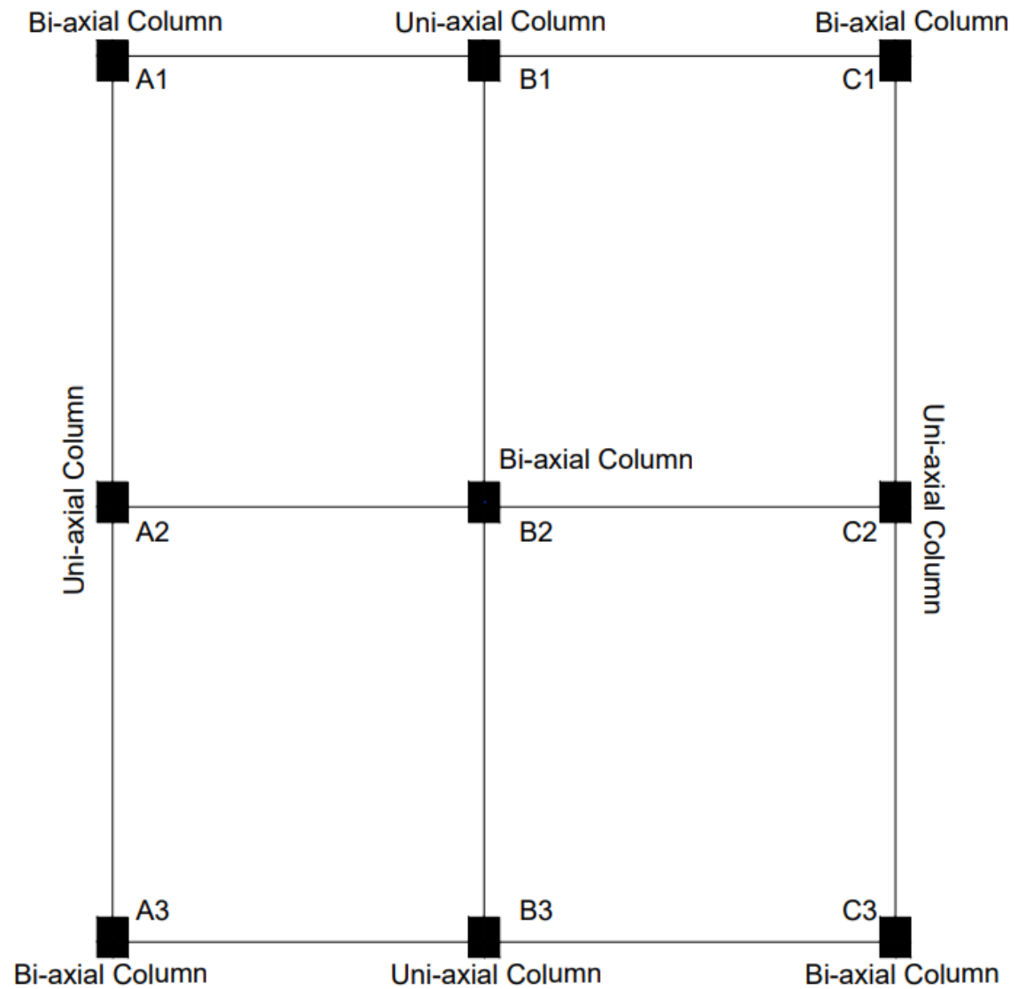
Figure 4.4: Classification of column based on position and loading.
