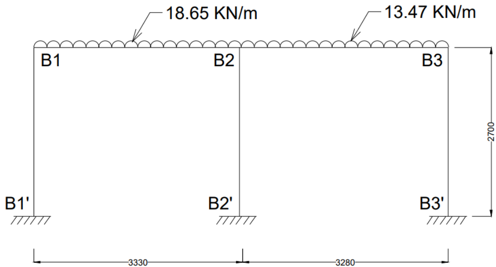
Figure 3.13: Frame B1-B2-B3 with loads.
