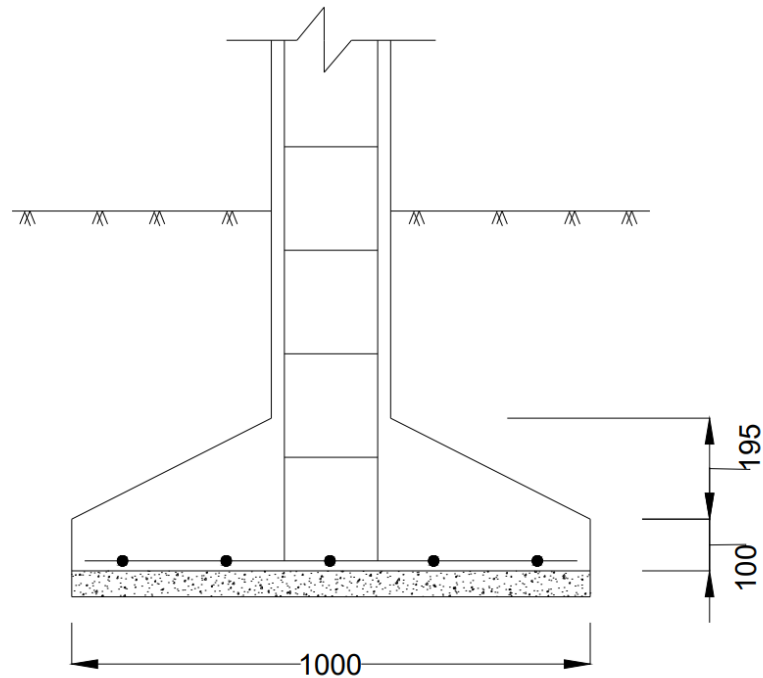
Figure 5.5: Footing reinforcement
