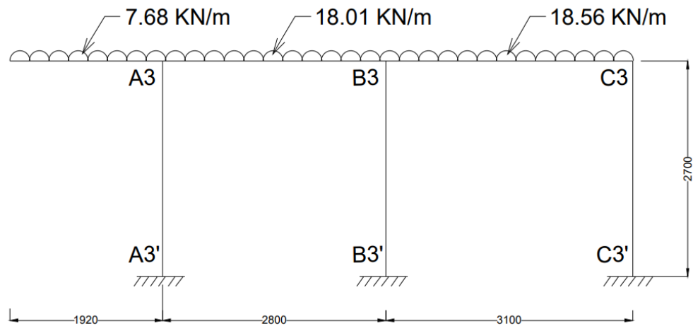
Figure 3.9: Frame A3-B3-C3 with loads.
