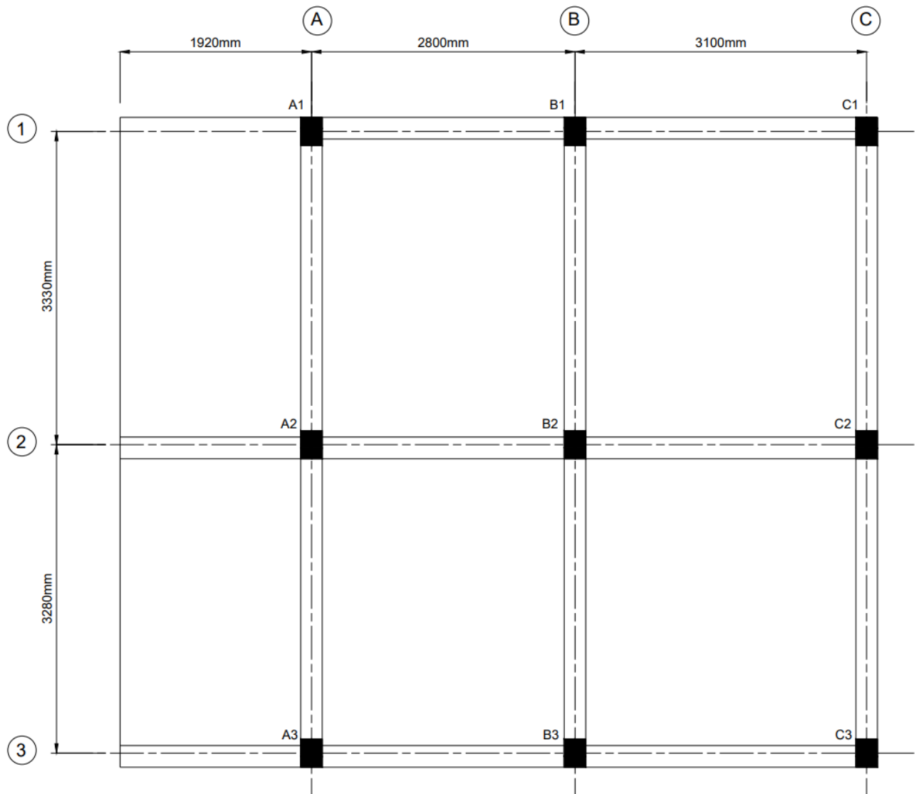
Figure 5.4: Beam layout
