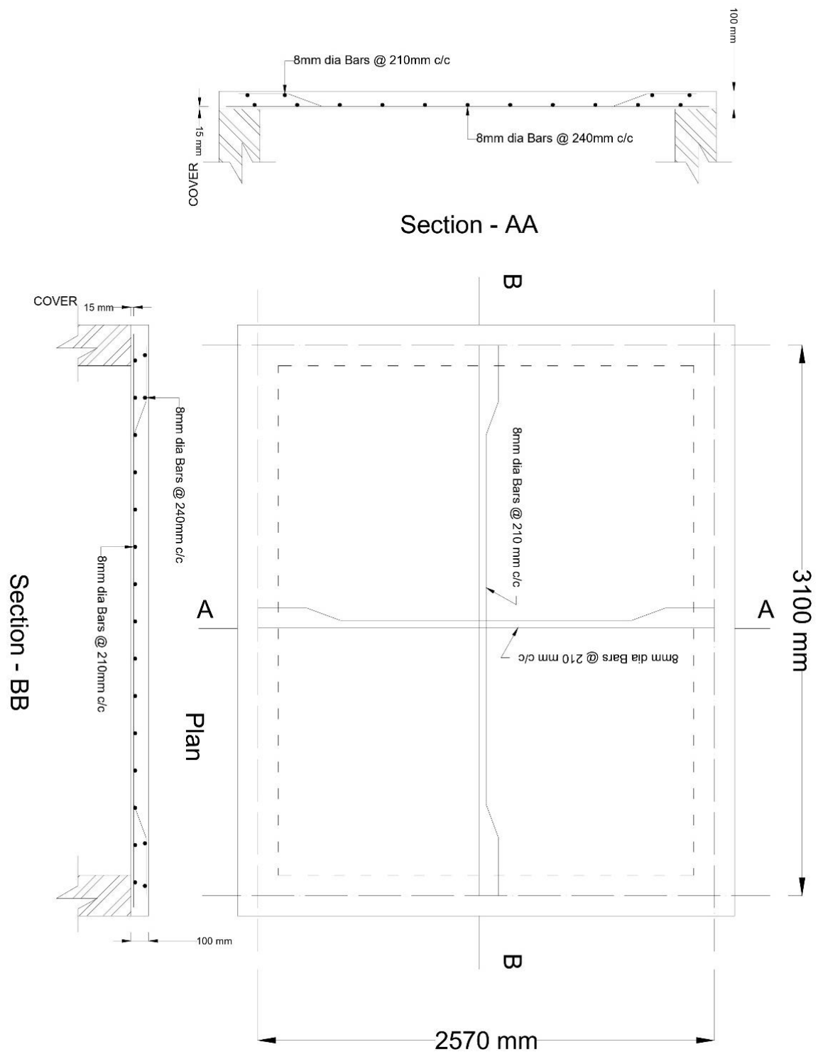
Figure 5.6: Slab reinforcement
