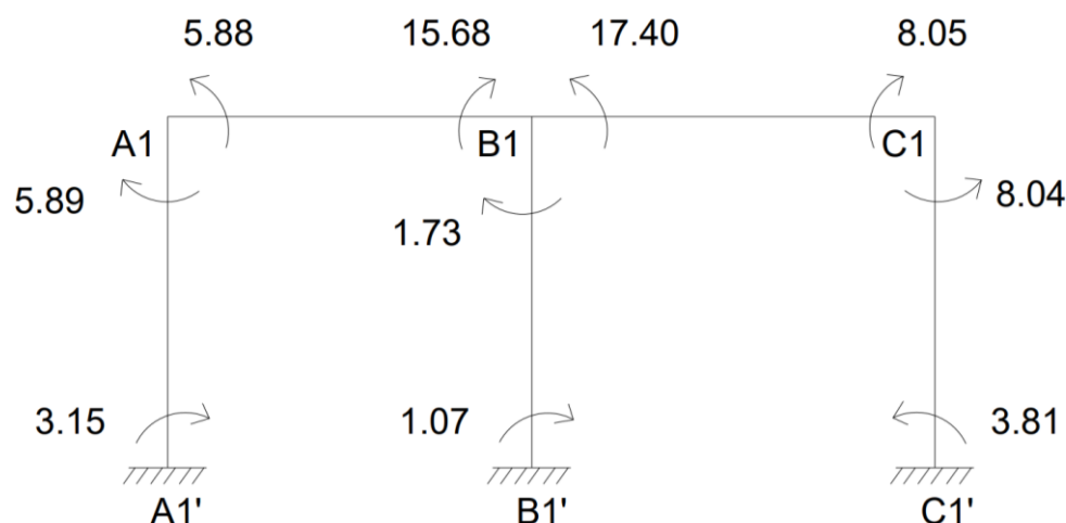
Figure 3.18: Final End Moments
