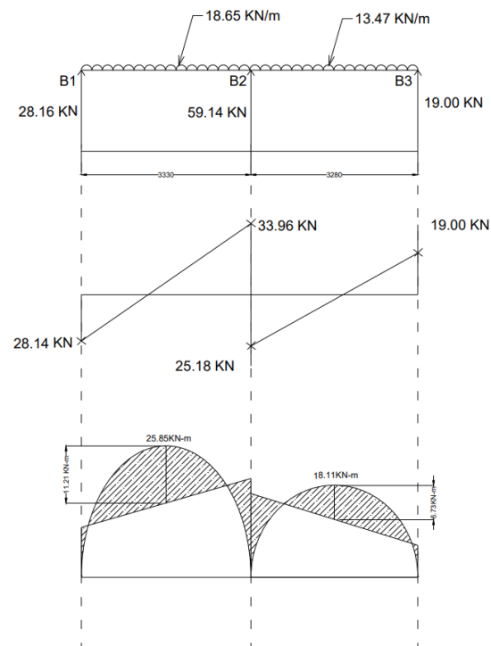
Figure 3.25: Bending Moment and Shear Force Diagram of B1-B2-B3
