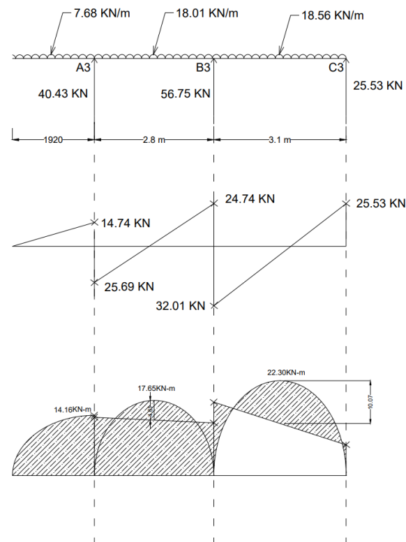
Figure 3.23: Bending Moment and Shear Force Diagram of A3-B3-C3
