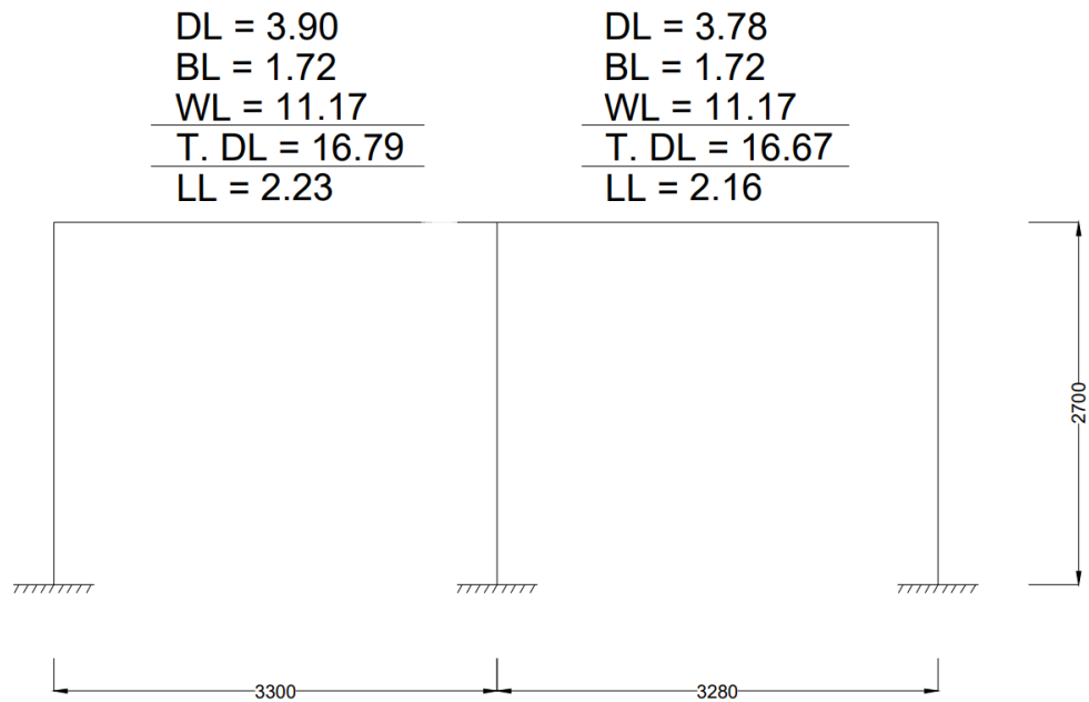
Figure 3.14: Load calculation in frame C1-C2-C3.
