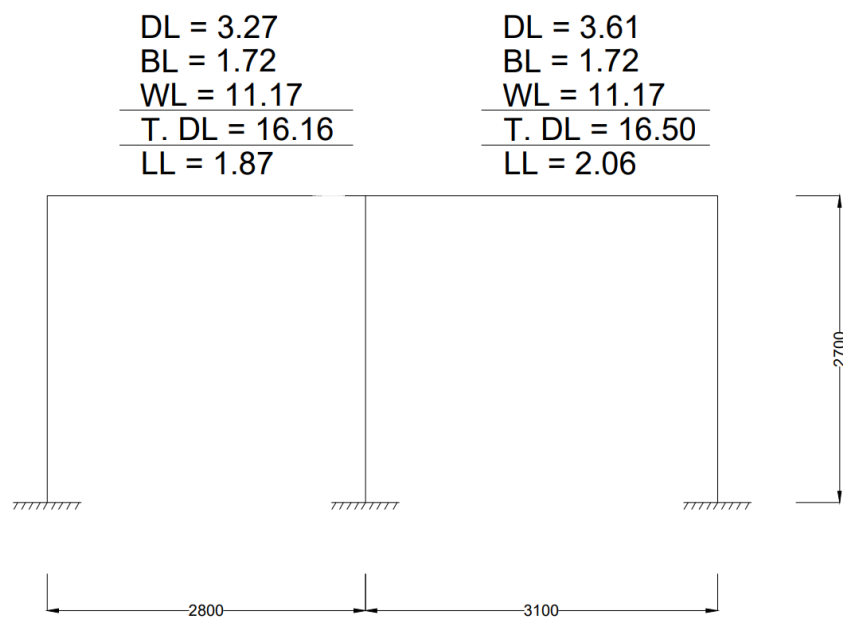
Figure 3.4: Load calculation in frame A1-B1-C1.
