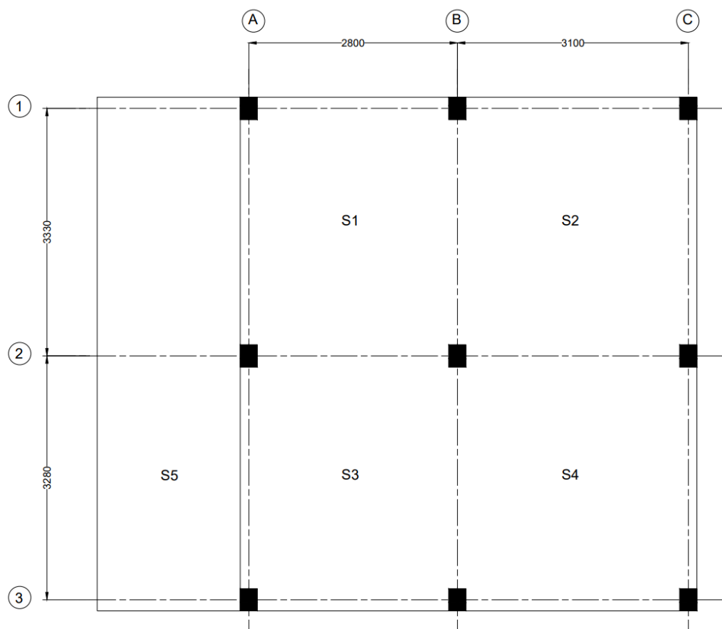
Figure 4.1: Floor Slab.
