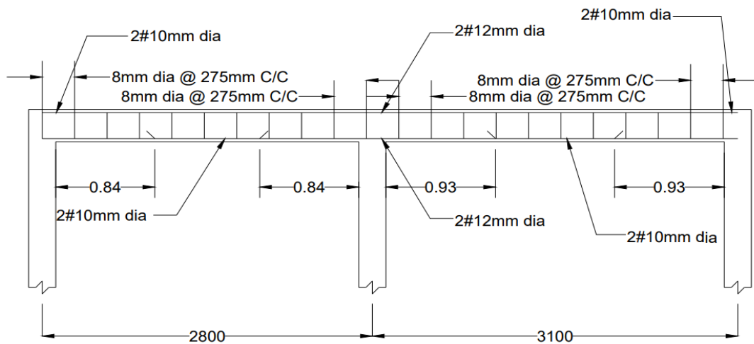
Figure 4.3: Reinforcement details of beam A1-B1-C1.
