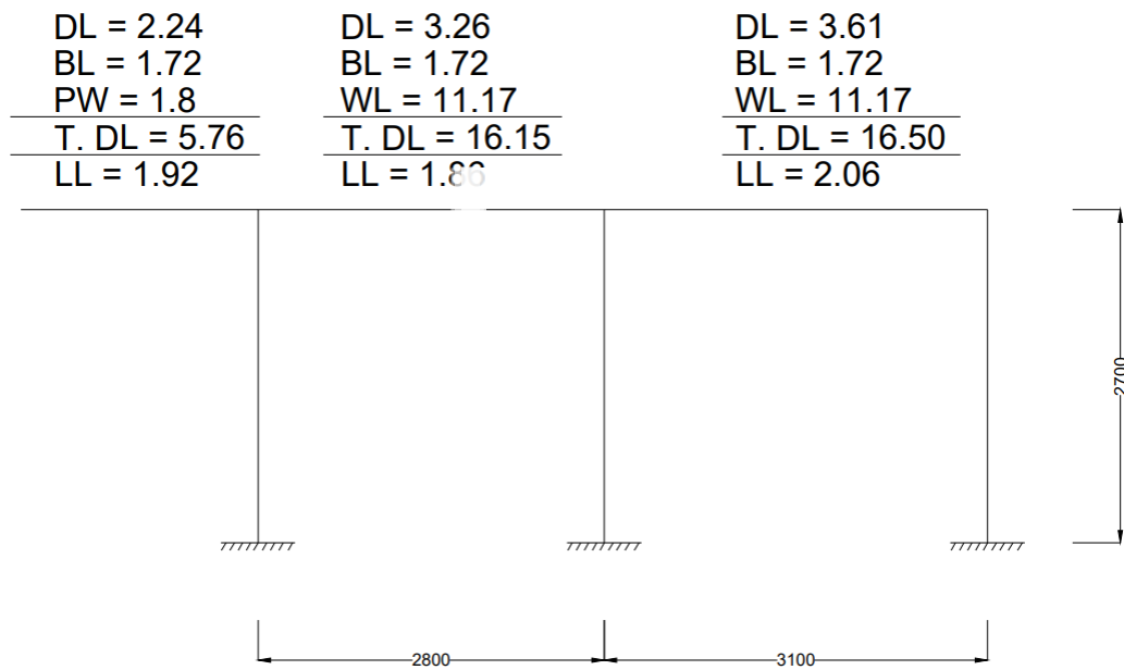
Figure 3.8: Load calculation in frame A3-B3-C3.
