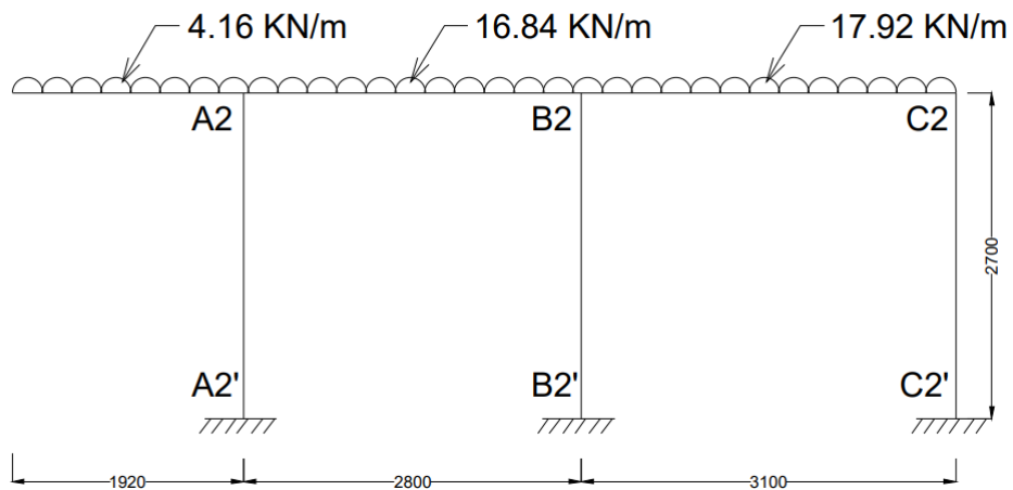
Figure 3.7: Frame A2-B2-C2 with loads.
