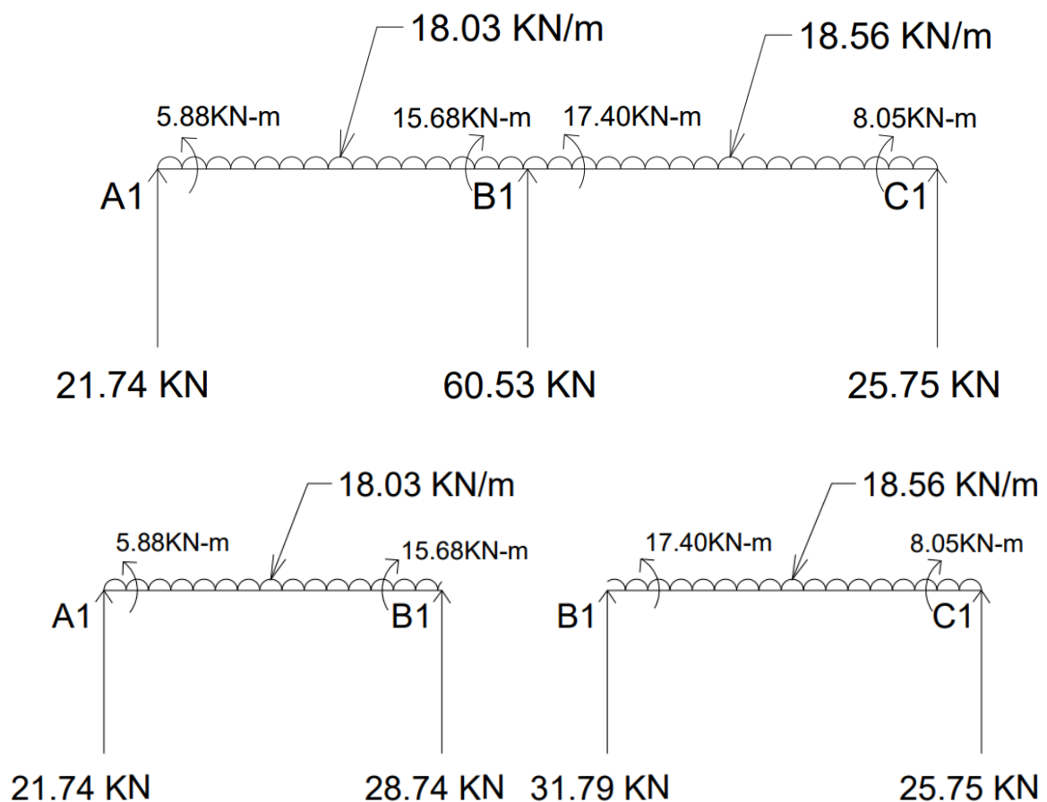
Figure 3.20: Reactions
