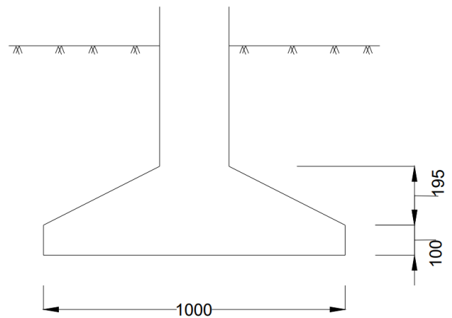
Figure 4.8: One way Shear
