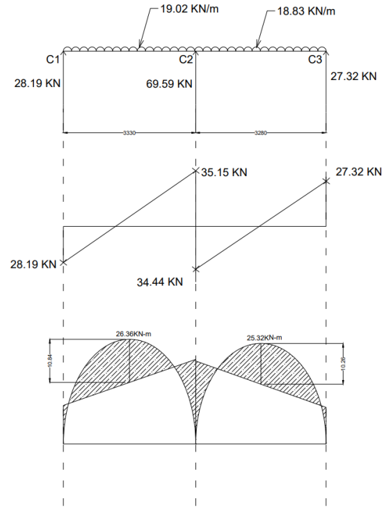
Figure 3.26: Bending Moment and Shear Force Diagram of C1-C2-C3
