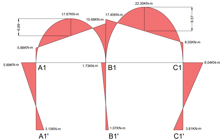
Figure 3.19: Bending Moment Diagram
