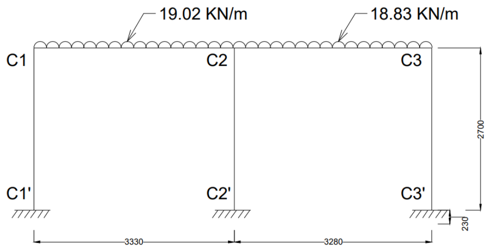
Figure 3.15: Frame C1-C2-C3 with loads.
