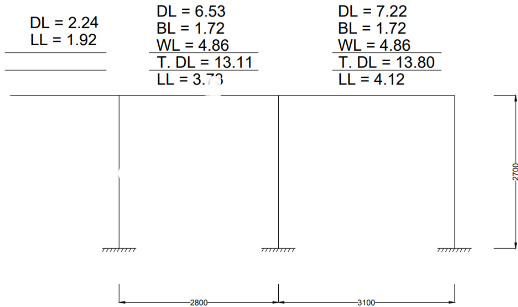
Figure 3.6: Load calculation in frame A2-B2-C2.
