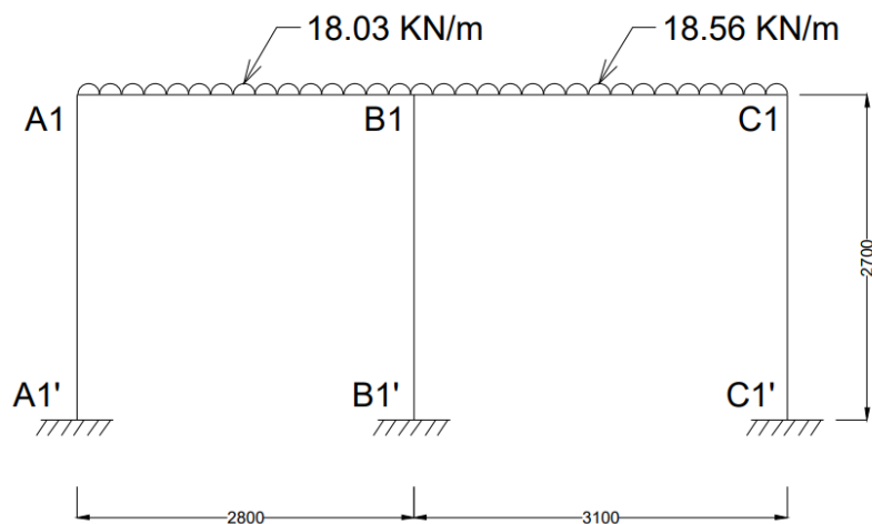
Figure 3.5: Frame A1-B1-C1 with loads.
