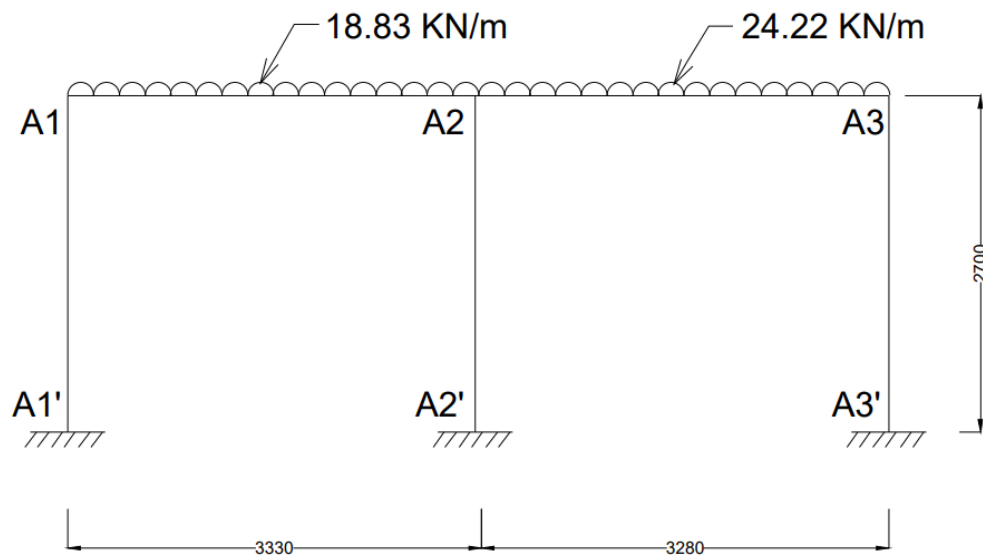
Figure 3.11: Frame A1-A2-A3 with loads.
