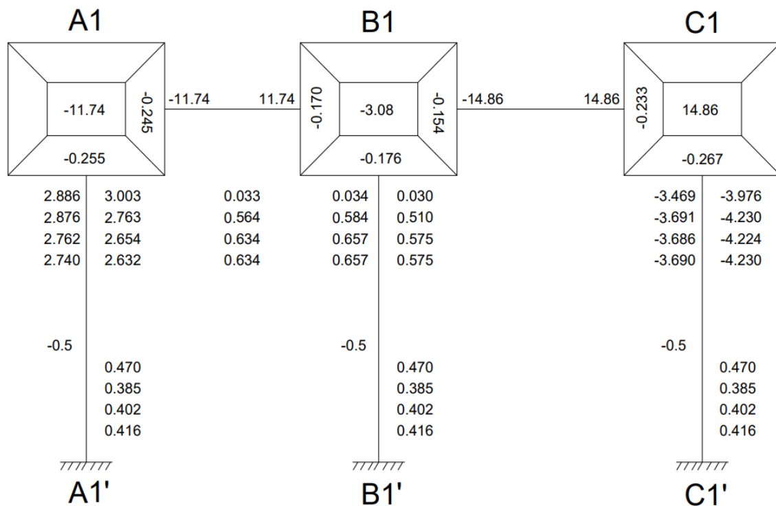
Figure 3.17: Rotation and Displacement Contribution
