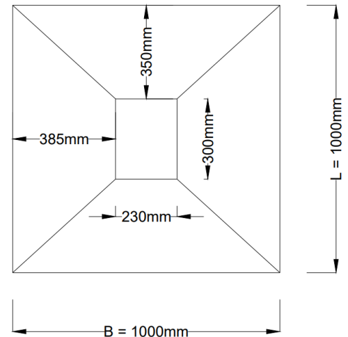
Figure 4.7: Area of Footing
