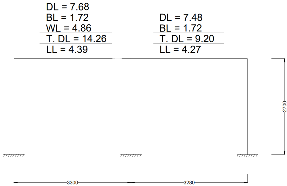
Figure 3.12: Load calculation in frame B1-B2-B3.
