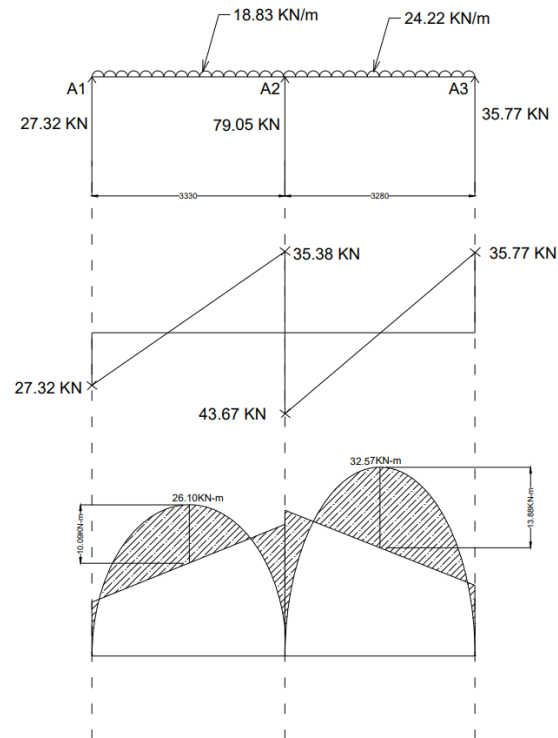
Figure 3.24: Bending Moment and Shear Force Diagram of A1-A2-A3
