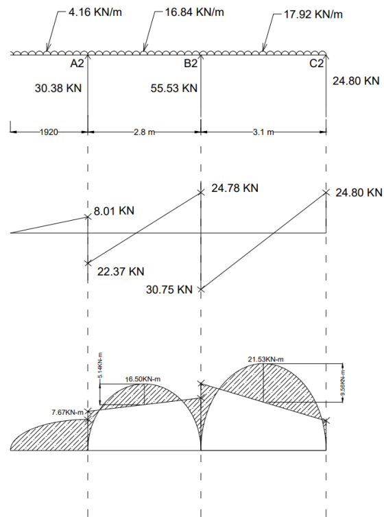
Figure 3.22: Bending Moment and Shear Force Diagram of A2-B2-C2
