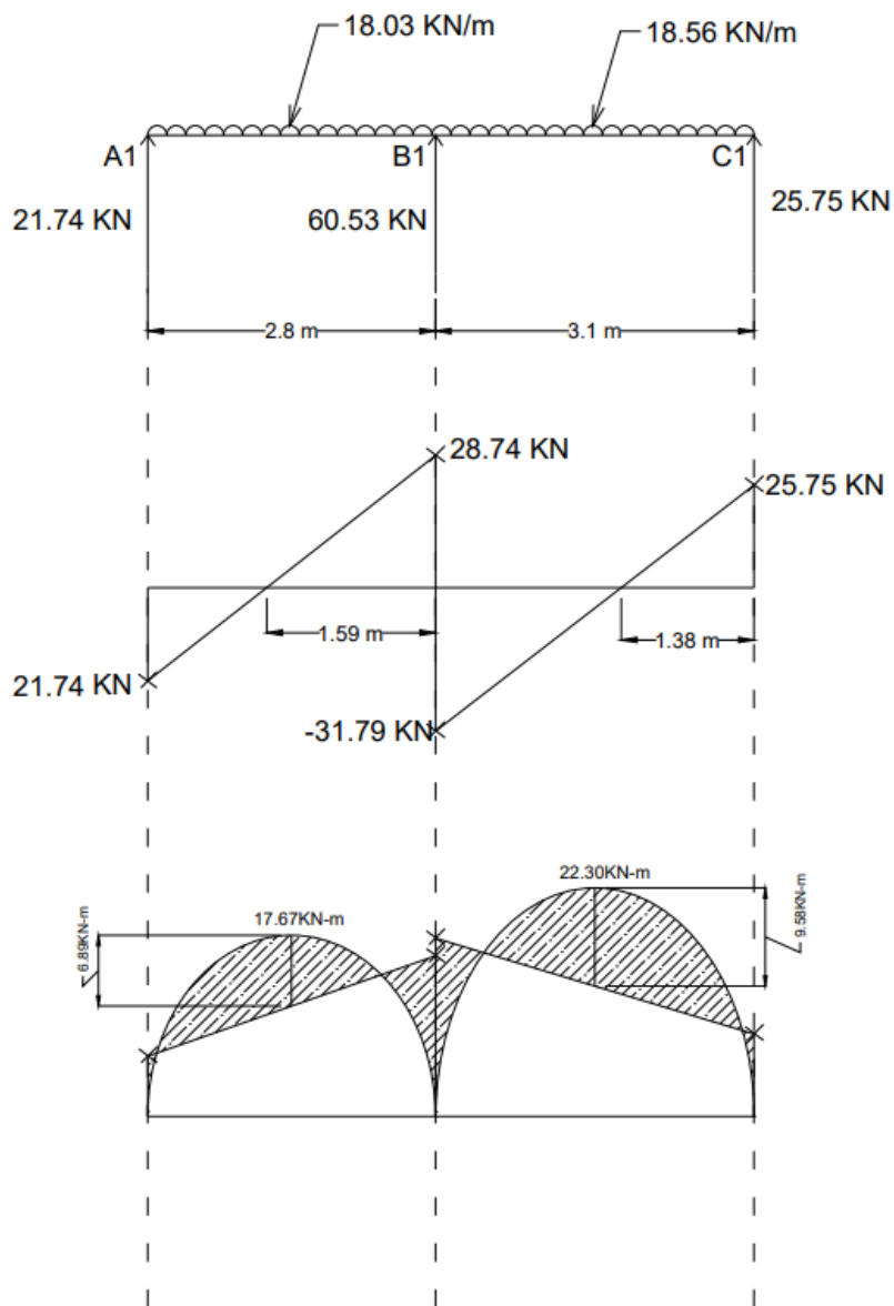
Figure 3.21: Bending Moment and Shear Force Diagram of A1-B1-C1
