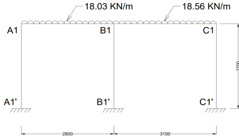
Figure 3.16: Frame A1-B1-C1
