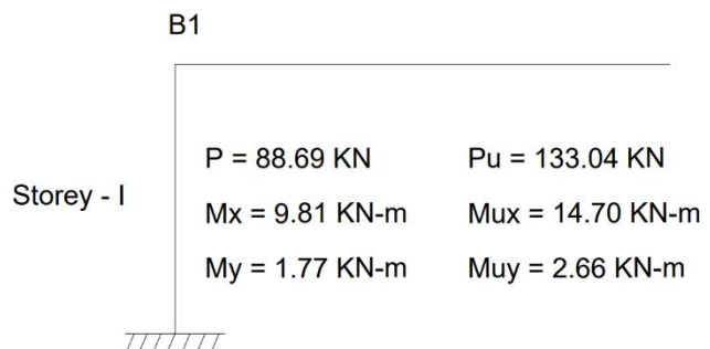
Figure 4.6: Total Loads and moments on B1 column.
