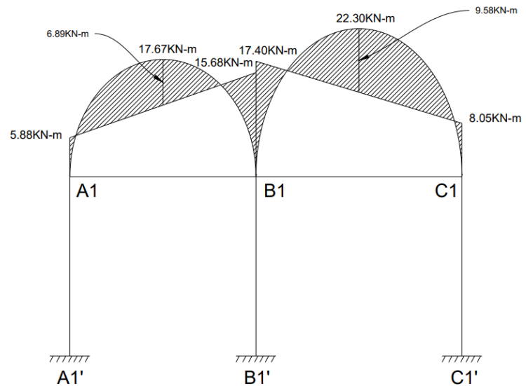
Figure 4.2: Bending moment diagram {frame A1-B1-C1}
