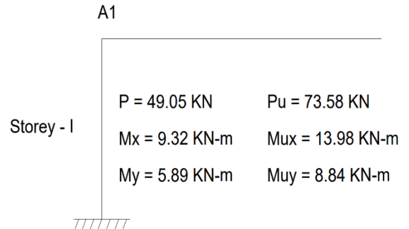
Figure 4.5: Total Loads and moments on A1 column.
