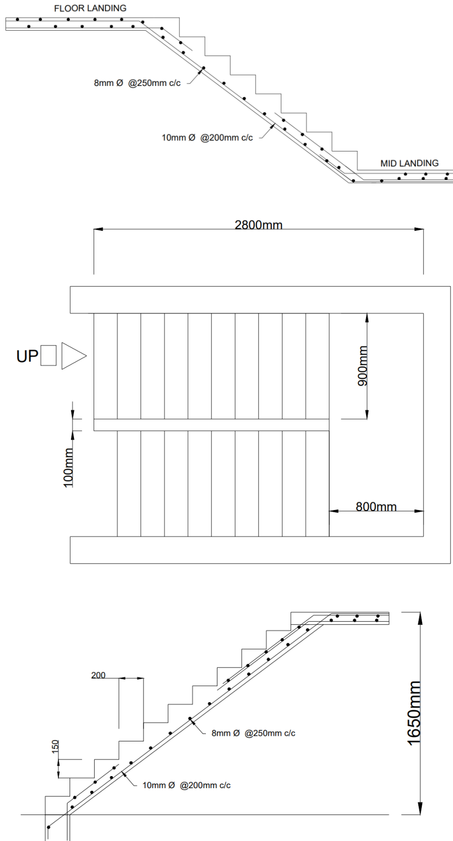
Figure 5.7: Staircase reinforcement
