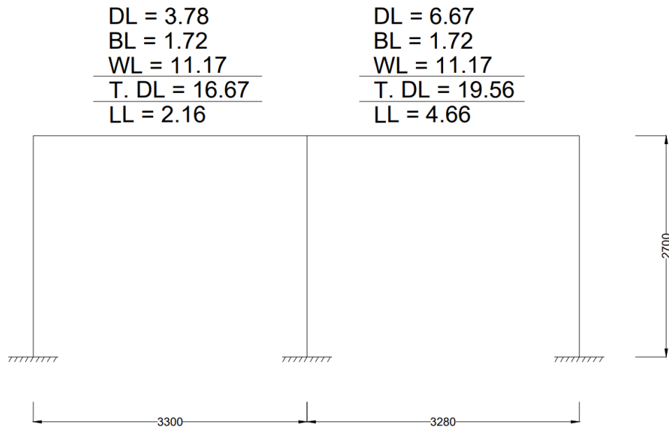
Figure 3.10: Load calculation in frame A1-A2-A3.
