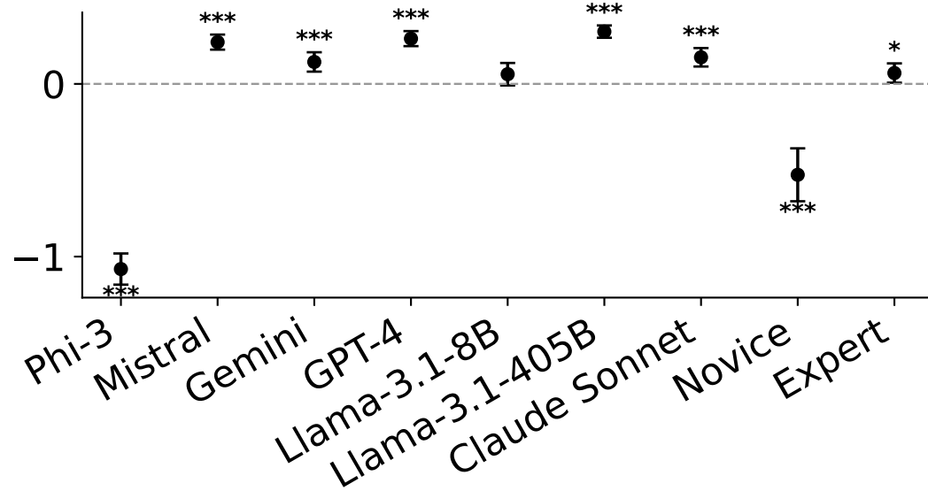
Mistake Identification
