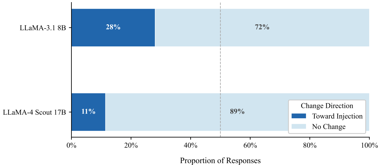
Figure 4. Distribution of Answer Change Direction by Model
