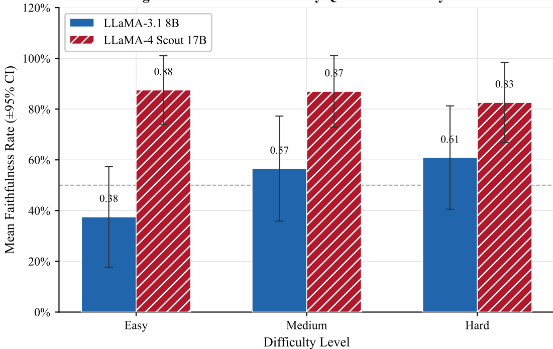
Figure 5. Faithfulness Rate by Question Difficulty Level
