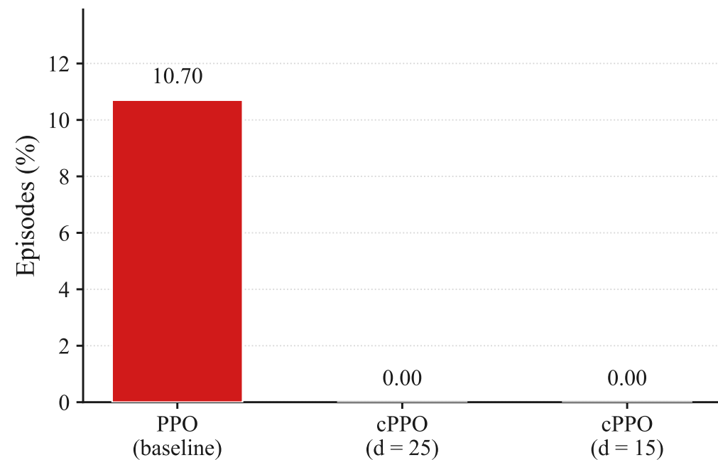
(b) Joint limit touched
